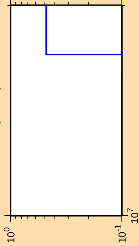
\Delta\sigma/\sigma vs. E for ^{186}\text{Ir}(n,3n\alpha)
