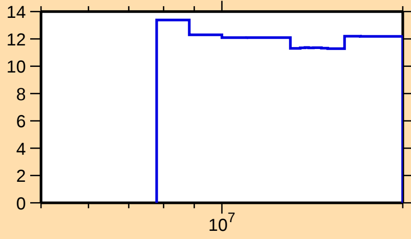
\Delta\sigma/\sigma vs. E for ^{187}\text{Ir}(n,\text{nonel.})
