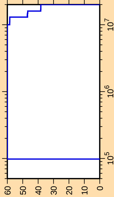
\Delta\sigma/\sigma vs. E for ^{187}\text{Ir}(n,p)
