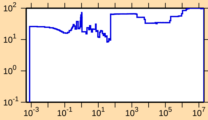
\Delta\sigma/\sigma vs. E for ^{187}\text{Ir}(n,\gamma)
