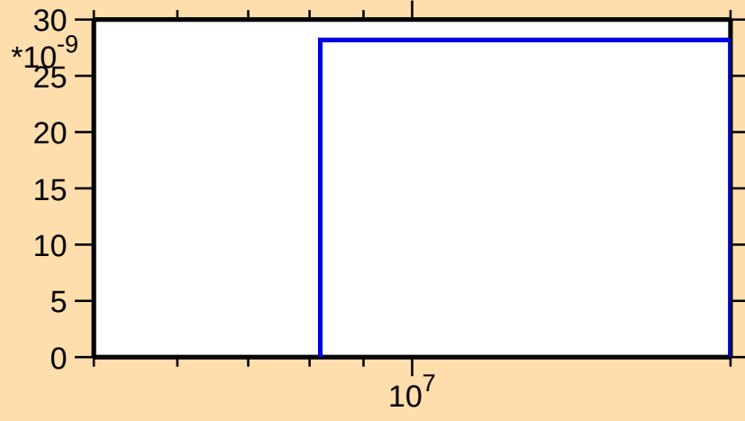
\sigma vs. E for ^{187}\text{Ir}(n,2n\alpha)
