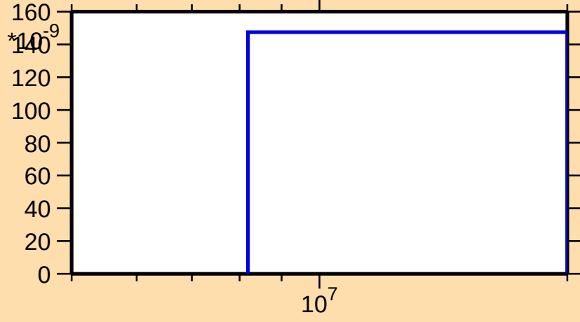
\sigma vs. E for ^{187}\text{Ir}(n,2np)
