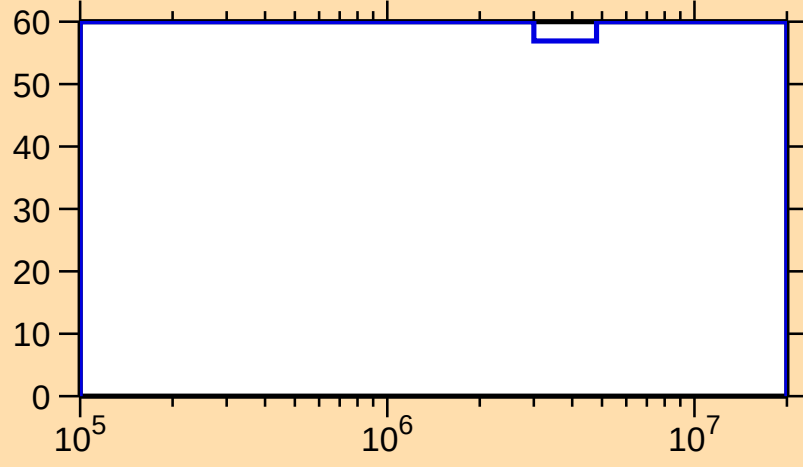
\Delta\sigma/\sigma vs. E for ^{187}\text{Ir}(n,n_1)
