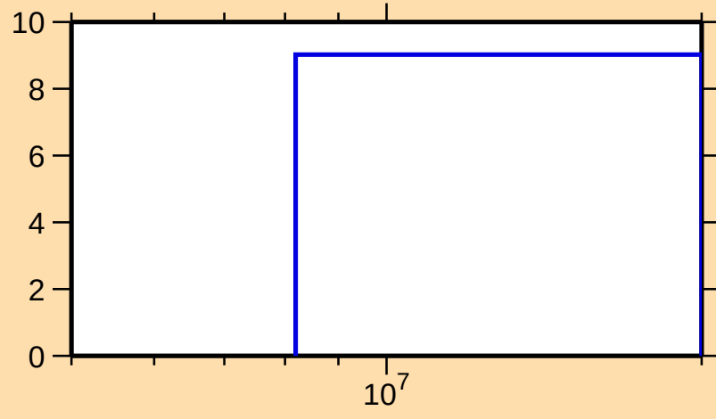
\Delta\sigma/\sigma vs. E for ^{187}\text{Ir}(n,\text{el.})
