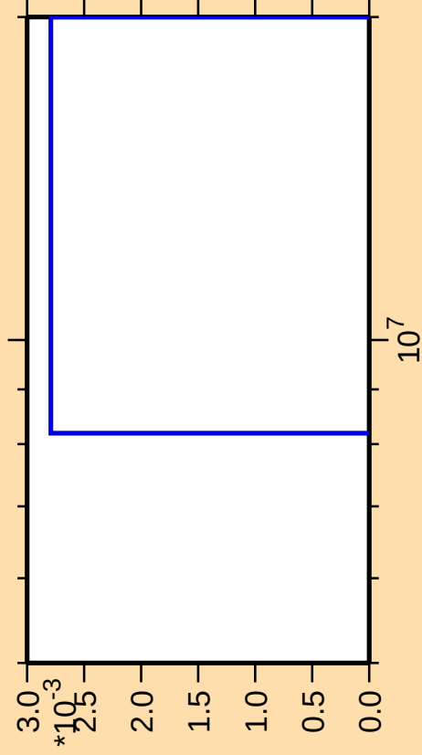
\Delta\sigma/\sigma vs. E for ^{187}\text{Ir}(\text{mt } 34)
