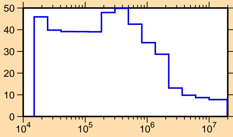
\Delta\sigma/\sigma vs. E for ^{190}\text{Ir}(n,\text{nonel.})
