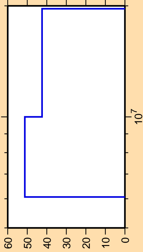
\Delta\sigma/\sigma vs. E for ^{190}\text{Ir}(n,n_1)
