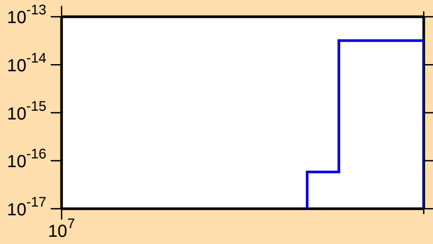
\sigma vs. E for ^{190}\text{Ir}(\text{mt } 34)
