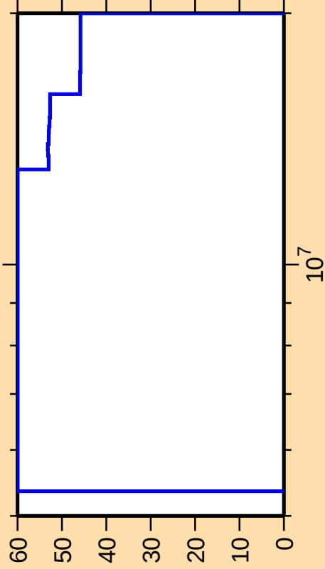
\Delta\sigma/\sigma vs. E for ^{190}\text{Ir}(n,\alpha)
