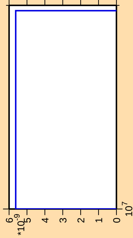
\Delta\sigma/\sigma vs. E for ^{190}\text{Ir}(\text{mt } 42)
