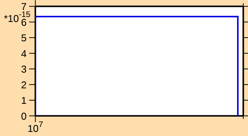
\sigma vs. E for ^{190}\text{Ir}(n,3n\alpha)
