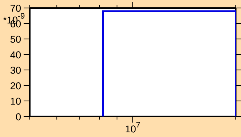
\sigma vs. E for ^{190}\text{Ir}(n,2n\alpha)
