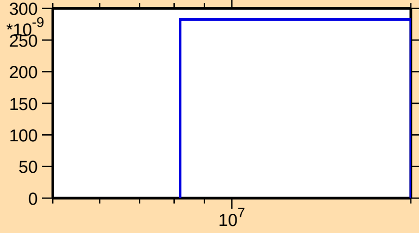
\sigma vs. E for ^{190}\text{Ir}(n,\text{nd})
