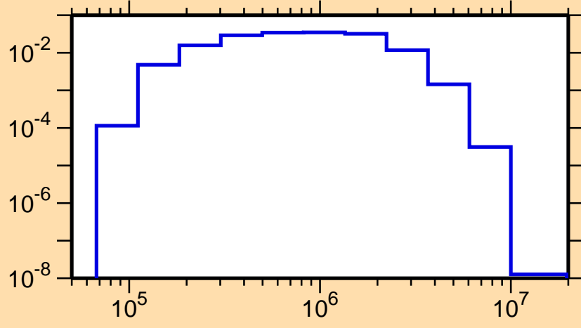
\sigma vs. E for ^{195}\text{Ir}(n,n_2)
