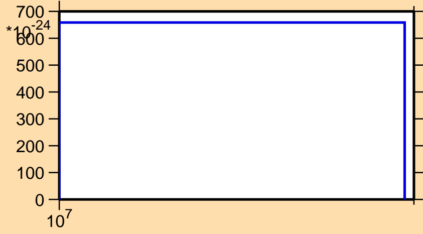
\sigma vs. E for ^{195}\text{Ir} (mt 42)
