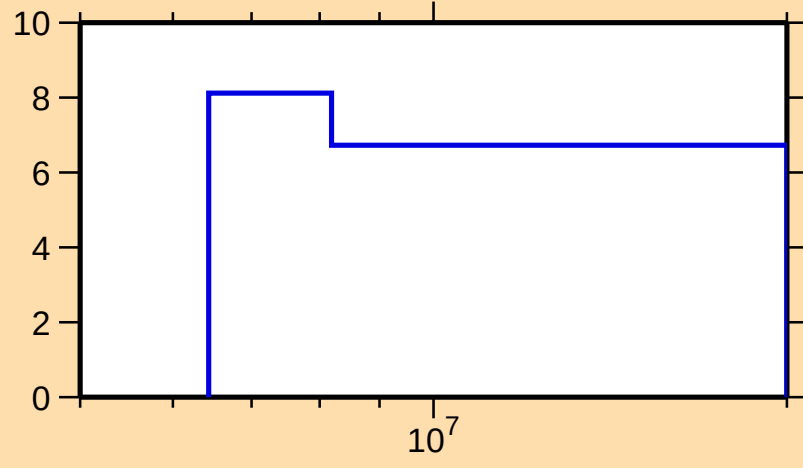
\Delta\sigma/\sigma vs. E for ^{195}\text{Ir}(n,\text{nonel.})
