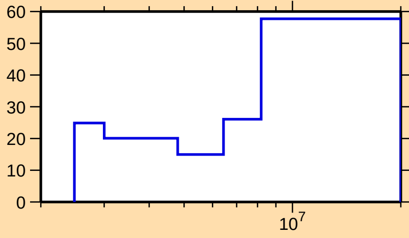
\Delta\sigma/\sigma vs. E for ^{195}\text{Ir}(n,n\text{cont.})
