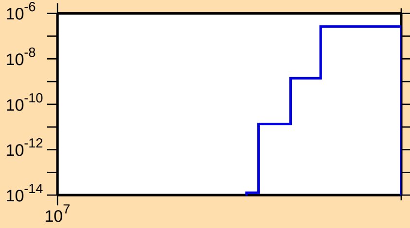
\sigma vs. E for ^{200}\text{Ir}(n,\text{nt})
