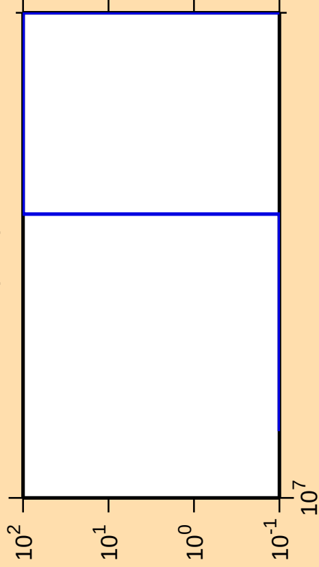
\Delta\sigma/\sigma vs. E for ^{200}\text{Ir}(n,\text{nt})
