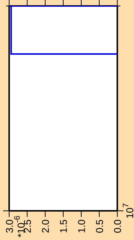
\Delta\sigma/\sigma vs. E for ^{200}\text{Ir}(\text{mt 42})
