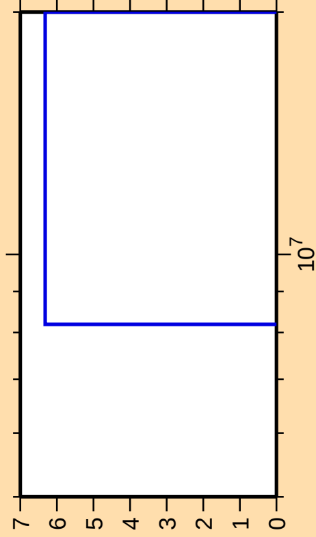
\Delta\sigma/\sigma vs. E for ^{200}\text{Ir}(n,2n\alpha)
