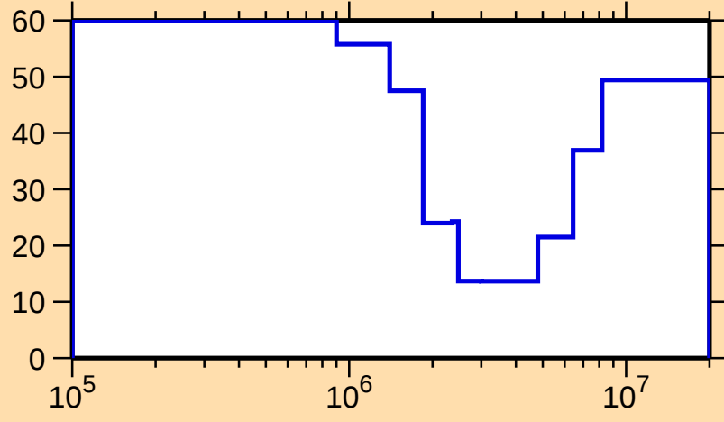
\Delta\sigma/\sigma vs. E for ^{200}\text{Ir}(n,n\text{cont.})
