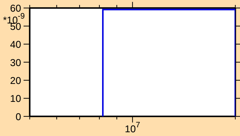
\sigma vs. E for ^{200}\text{Ir}(n,\alpha)
