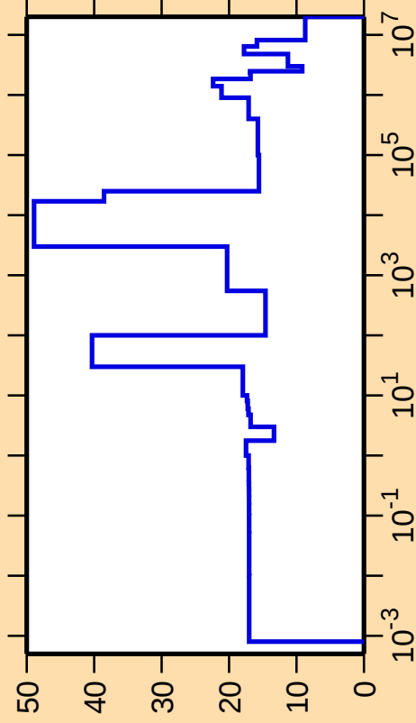
\Delta\sigma/\sigma vs. E for ^{200}\text{Ir}(n,\text{el.})
