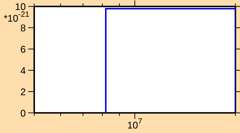
\sigma vs. E for ^{200}\text{Ir}(\text{mt } 42)
