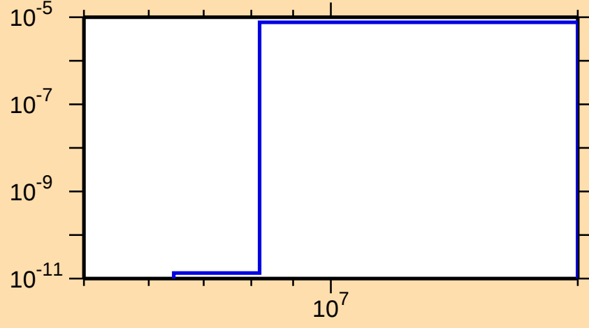
\sigma vs. E for ^{200}\text{Ir}(n,\alpha)
