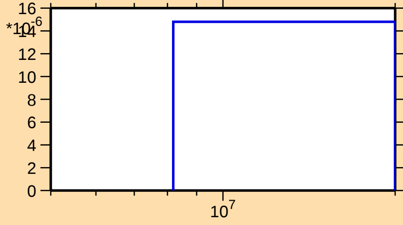
\sigma vs. E for ^{200}\text{Ir}(n,np)
