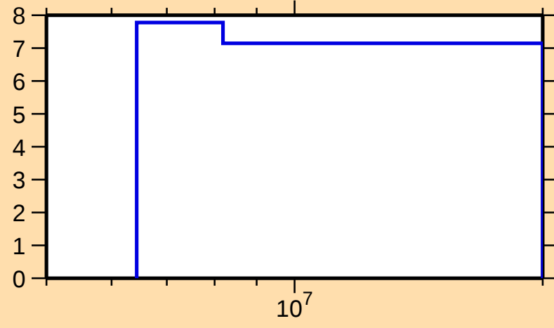
\Delta\sigma/\sigma vs. E for ^{200}\text{Ir}(n,\text{nonel.})
