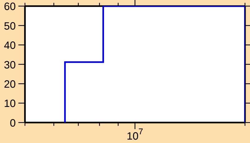
\Delta\sigma/\sigma vs. E for ^{200}\text{Ir}(n,\gamma)
