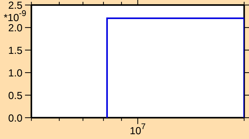
\sigma vs. E for ^{200}\text{Ir}(n,nt)
