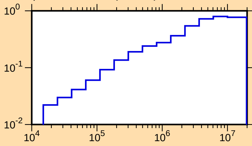
\mu vs. E for ^{41}\text{K}(\text{mt251})
