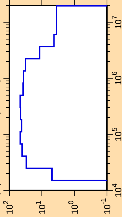
\Delta\mu/\mu vs. E for ^{41}\text{K}(\text{mt251})
