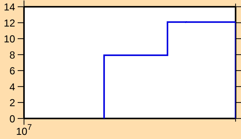
\Delta\sigma/\sigma vs. E for ^{45}\text{K}(n,2n)
