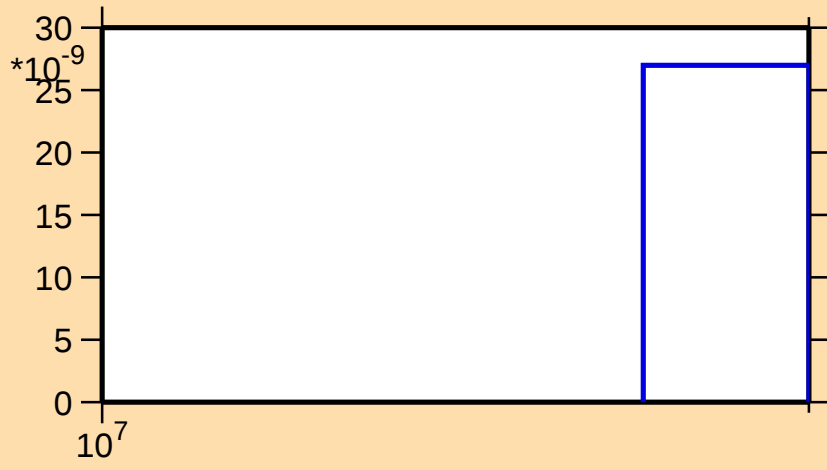
\sigma vs. E for ^{45}\text{K}(\text{n},\text{nd})
