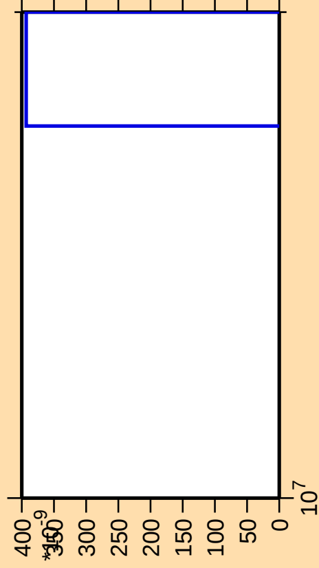
\Delta\sigma/\sigma vs. E for ^{45}\text{K}(n,2n\alpha)
