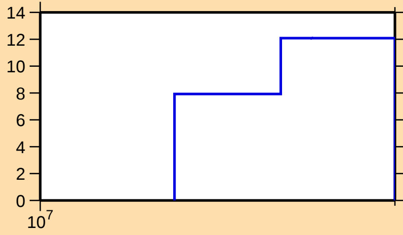
\Delta\sigma/\sigma vs. E for ^{45}\text{K}(n,2n)
