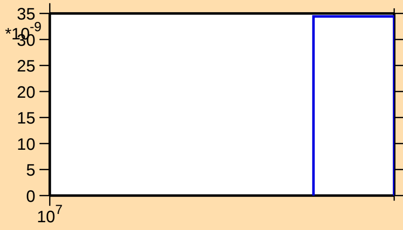
\sigma vs. E for ^{45}\text{K}(\text{n},\text{nt})
