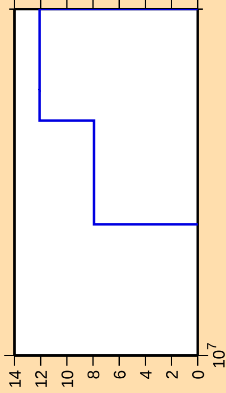
\Delta\sigma/\sigma vs. E for ^{45}\text{K}(n,2n)
