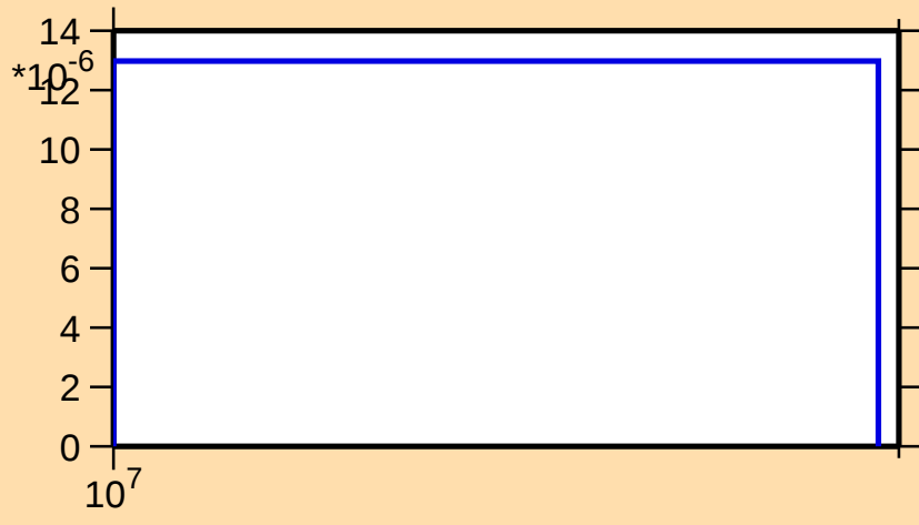
\sigma vs. E for ^{45}\text{K}(n,t)
