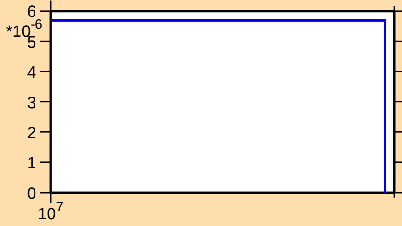
\sigma vs. E for ^{45}\text{K}(n,n\alpha)
