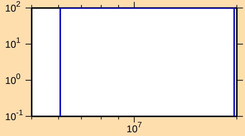
\Delta\sigma/\sigma vs. E for ^{45}\text{K}(n,\text{ncont.})
