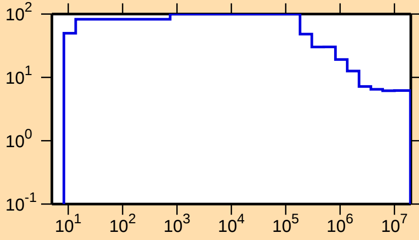
\Delta\sigma/\sigma vs. E for ^{45}\text{K}(n,\text{nonel.})
