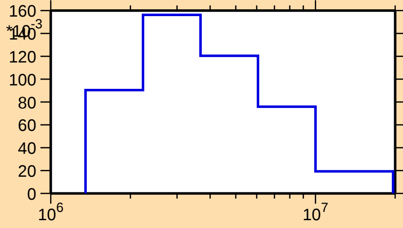
\sigma vs. E for ^{45}\text{K}(n,n_4)
