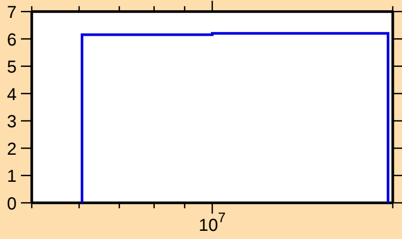
\Delta\sigma/\sigma vs. E for ^{45}\text{K}(n,n\text{onel.})
