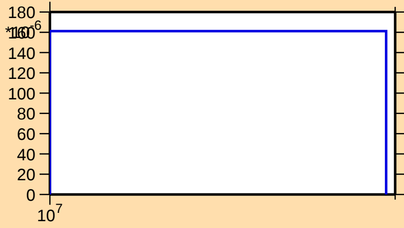
\sigma vs. E for ^{45}\text{K}(n,3n)
