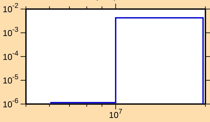
\sigma vs. E for ^{45}\text{K}(n,\alpha)
