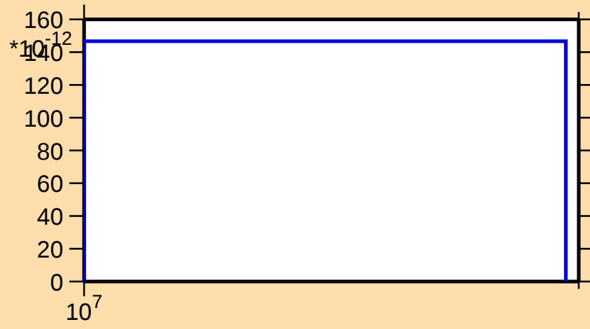
\sigma vs. E for ^{45}\text{K}(\text{n},\text{nd})
