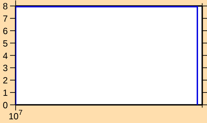
\Delta\sigma/\sigma vs. E for ^{45}\text{K}(n,\text{tot.})
