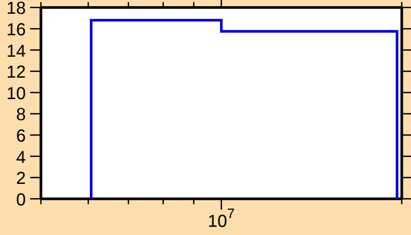
\Delta\sigma/\sigma vs. E for ^{45}\text{K}(\text{n},\text{el.})
