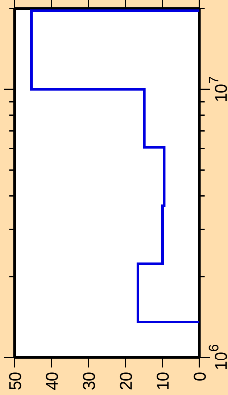
\Delta\sigma/\sigma vs. E for ^{45}\text{K}(n,n_4)
