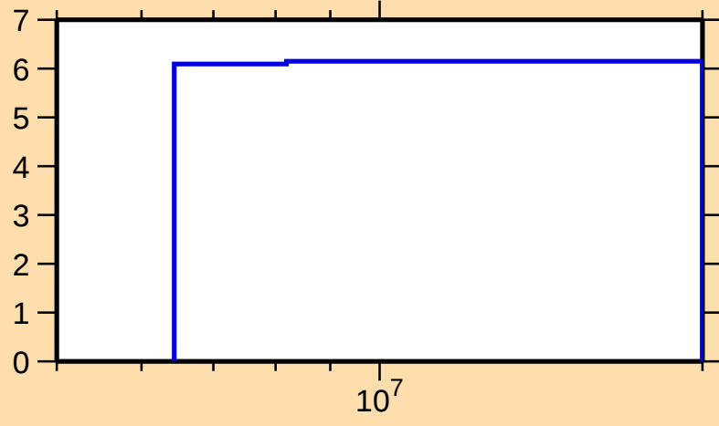
\Delta\sigma/\sigma vs. E for ^{45}\text{K}(\text{n},\text{nonel.})
