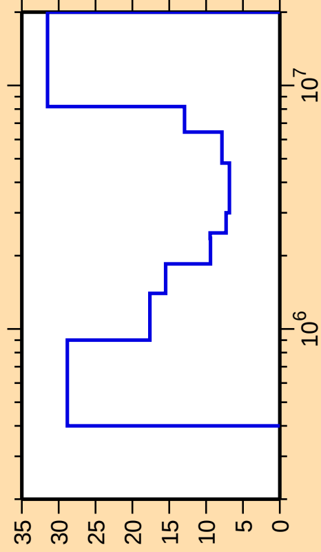
\Delta\sigma/\sigma vs. E for ^{45}\text{K}(n,\text{inel.})
