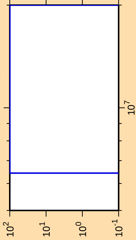
\Delta\sigma/\sigma vs. E for ^{45}\text{K}(\text{n},\text{ncont.})
