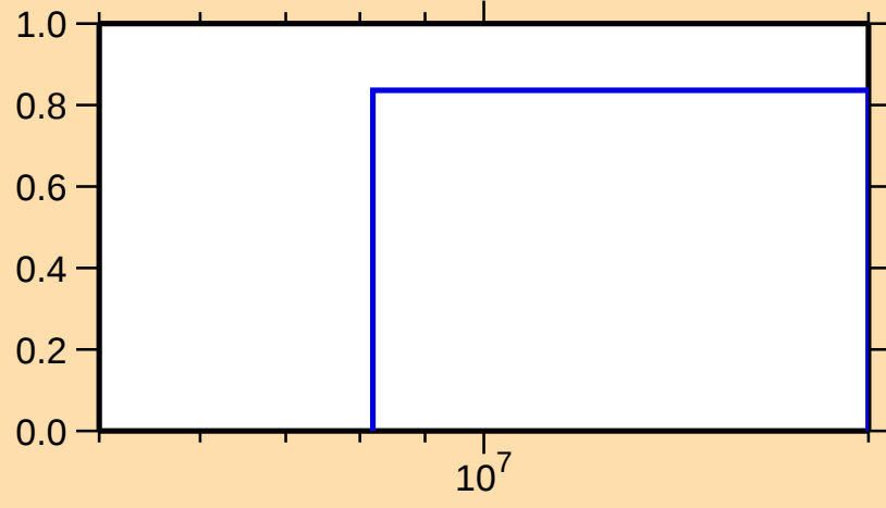
\sigma vs. E for ^{45}\text{K}(n,2n)
