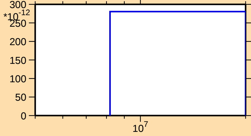
\sigma vs. E for ^{45}\text{K}(n,nt)
