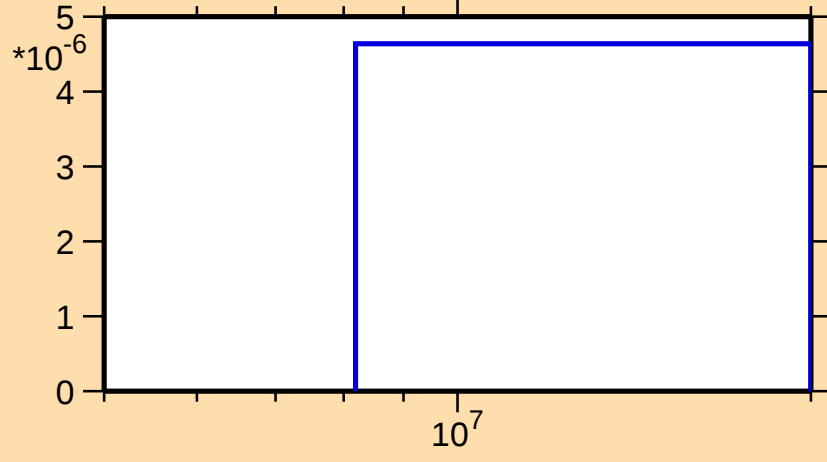
\sigma vs. E for ^{45}\text{K}(n,n\alpha)
