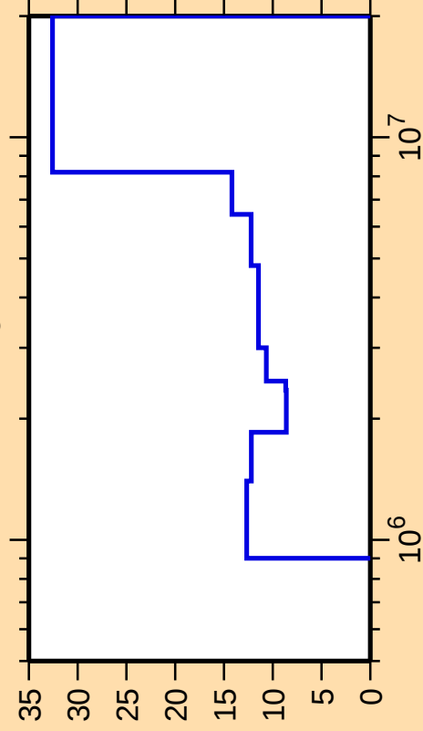
\Delta\sigma/\sigma vs. E for ^{45}\text{K}(n,n_3)
