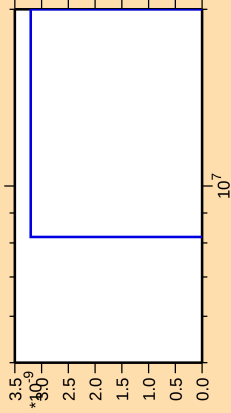
\Delta\sigma/\sigma vs. E for ^{45}\text{K}(n,2n\alpha)
