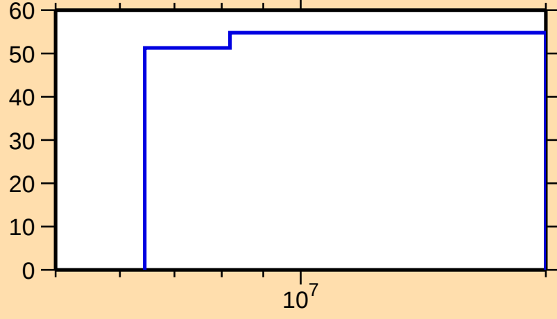
\Delta\sigma/\sigma vs. E for ^{45}\text{K}(n,p)
