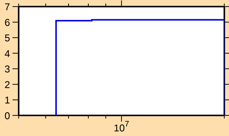
\Delta\sigma/\sigma vs. E for ^{45}\text{K}(n,\text{nonel.})
