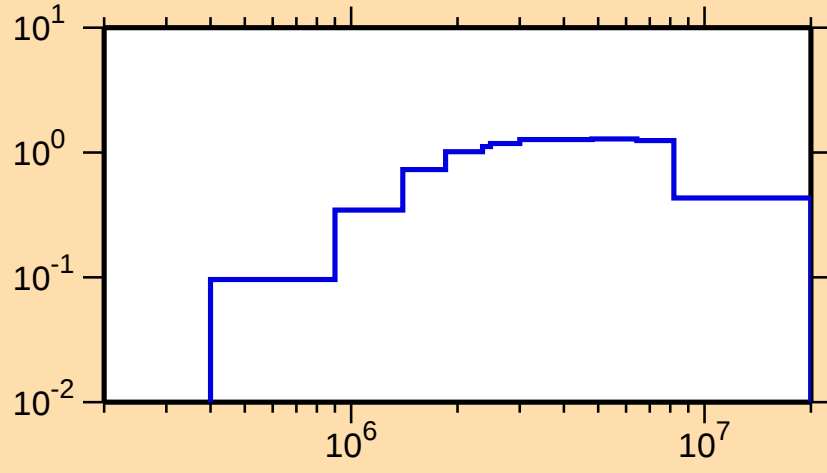
\sigma vs. E for ^{45}\text{K}(n,\text{inel.})
