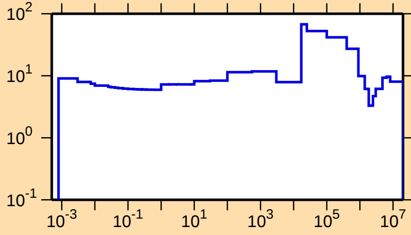
\Delta\sigma/\sigma vs. E for ^{45}\text{K}(\text{n,tot.})
