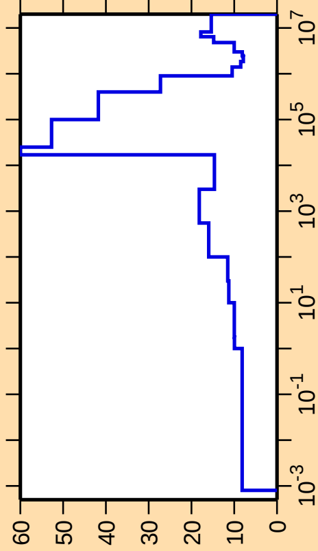
\Delta\sigma/\sigma vs. E for ^{45}\text{K}(\text{n},\text{el.})
