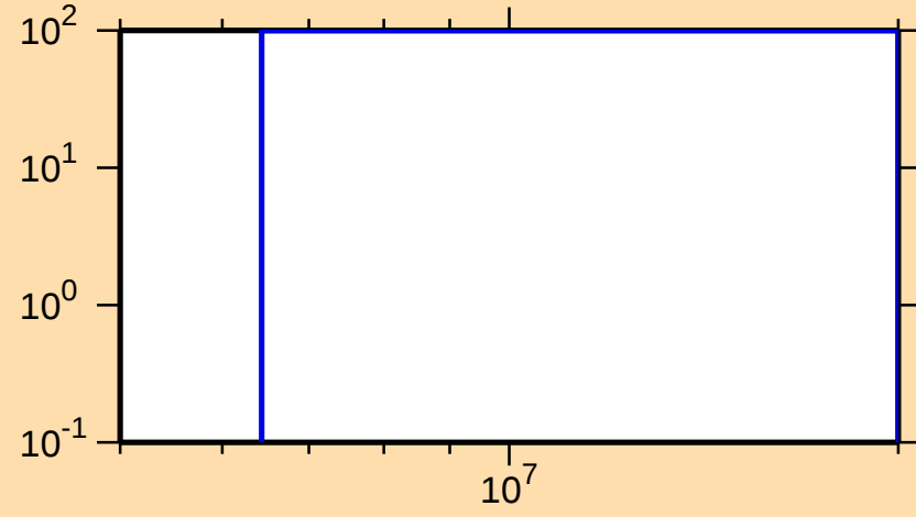
\Delta\sigma/\sigma vs. E for ^{45}\text{K}(n,n\text{cont.})
