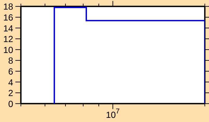
\Delta\sigma/\sigma vs. E for ^{45}\text{K}(n,\text{el.})
