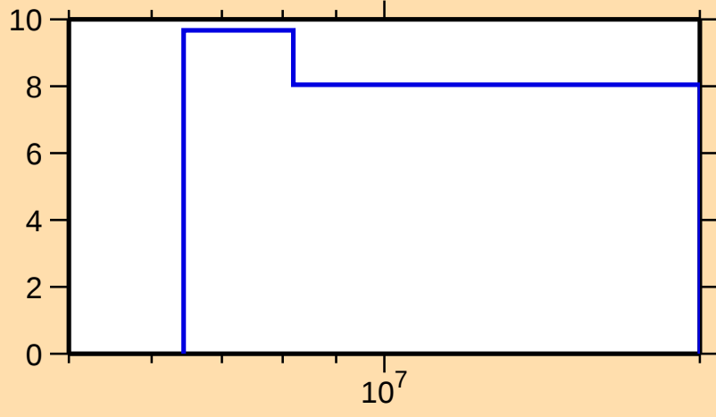
\Delta\sigma/\sigma vs. E for ^{45}\text{K}(n,\text{tot.})
