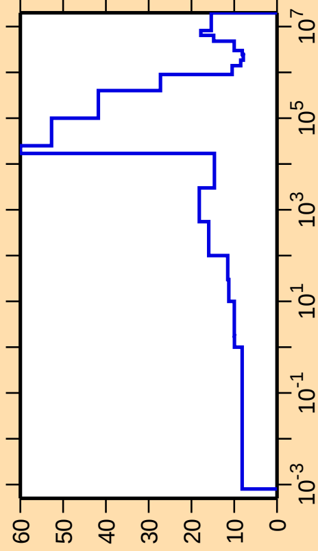
\Delta\sigma/\sigma vs. E for ^{45}\text{K}(\text{n,el.})
