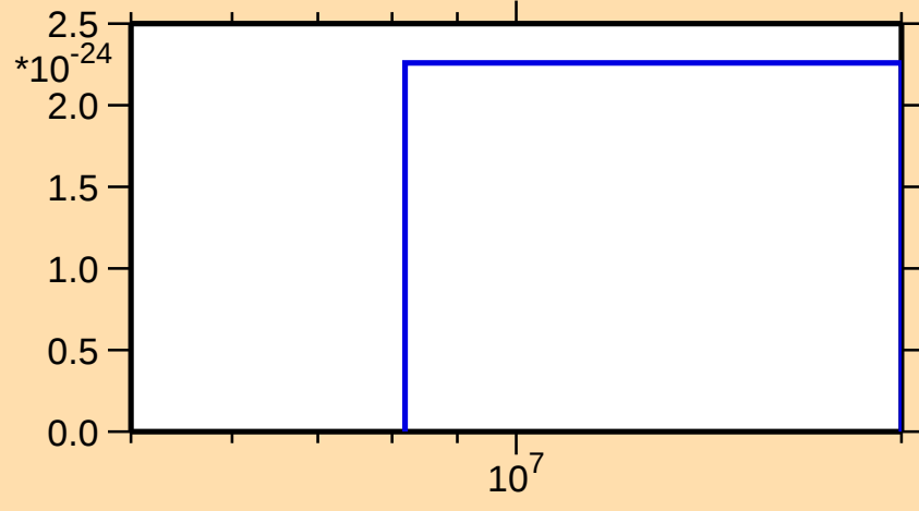
\sigma vs. E for ^{45}\text{K}(n,\text{He}3)
