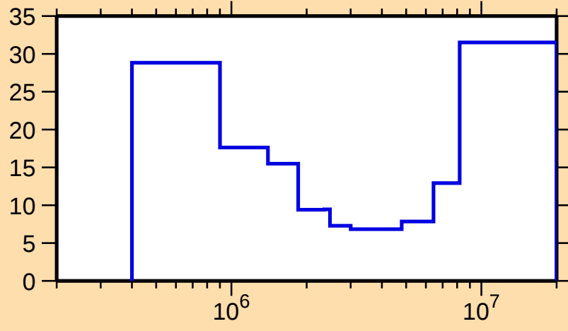
\Delta\sigma/\sigma vs. E for ^{45}\text{K}(n,\text{inel.})
