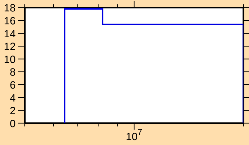
\Delta\sigma/\sigma vs. E for ^{45}\text{K}(\text{n},\text{el.})
