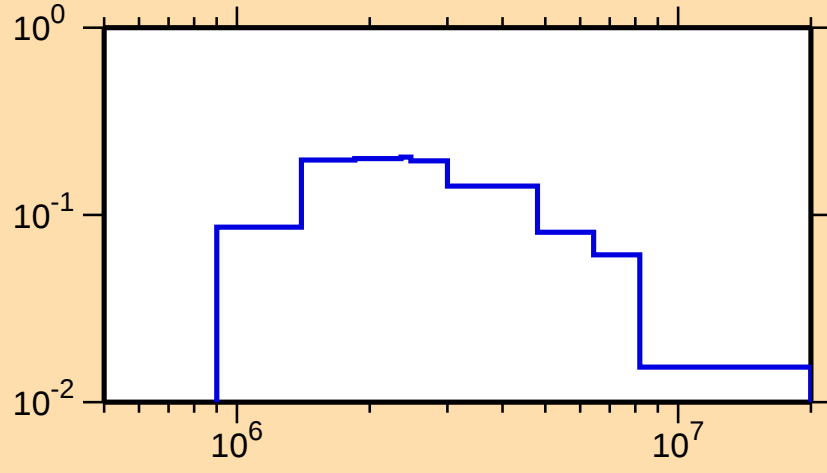
\sigma vs. E for ^{45}\text{K}(n,n_2)
