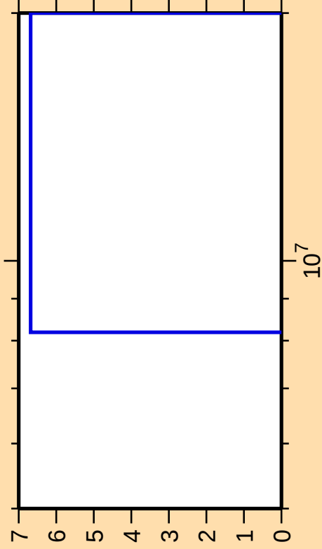
\Delta\sigma/\sigma vs. E for ^{45}\text{K}(n,2n)
