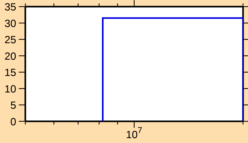
\Delta\sigma/\sigma vs. E for ^{45}\text{K}(n,\text{inel.})
