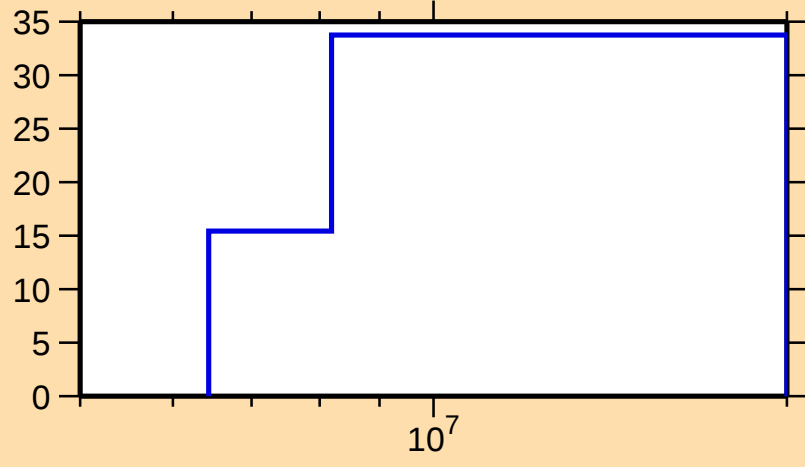
\Delta\sigma/\sigma vs. E for ^{45}\text{K}(n,n_1)
