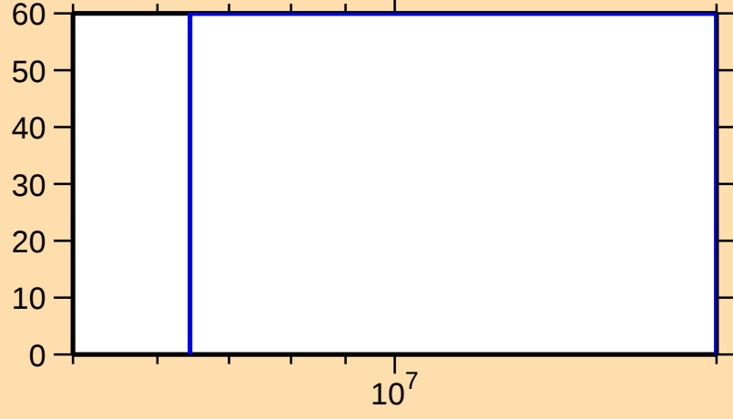
\Delta\sigma/\sigma vs. E for ^{45}\text{K}(n,\gamma)
