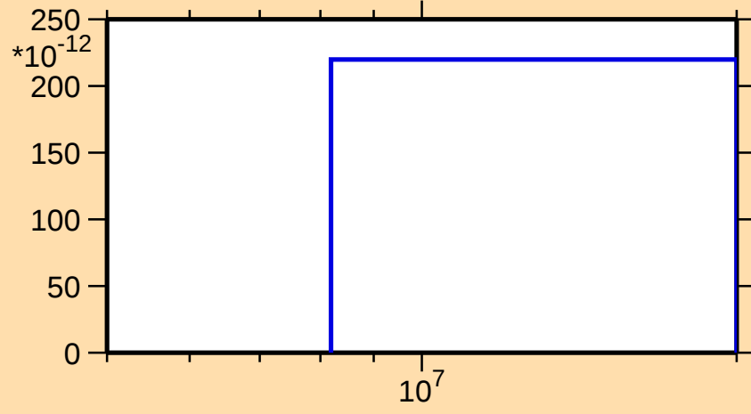
\sigma vs. E for ^{45}\text{K}(n,nd)
