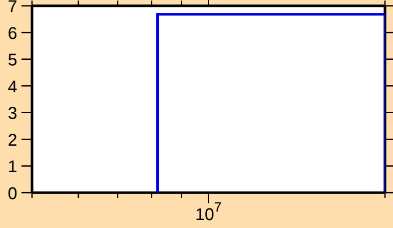
\Delta\sigma/\sigma vs. E for ^{45}\text{K}(n,2n)
