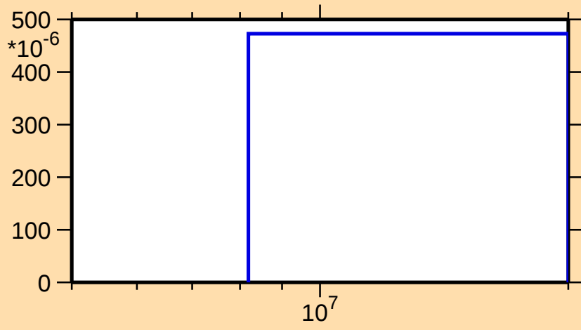
\sigma vs. E for ^{45}\text{K}(n,np)
