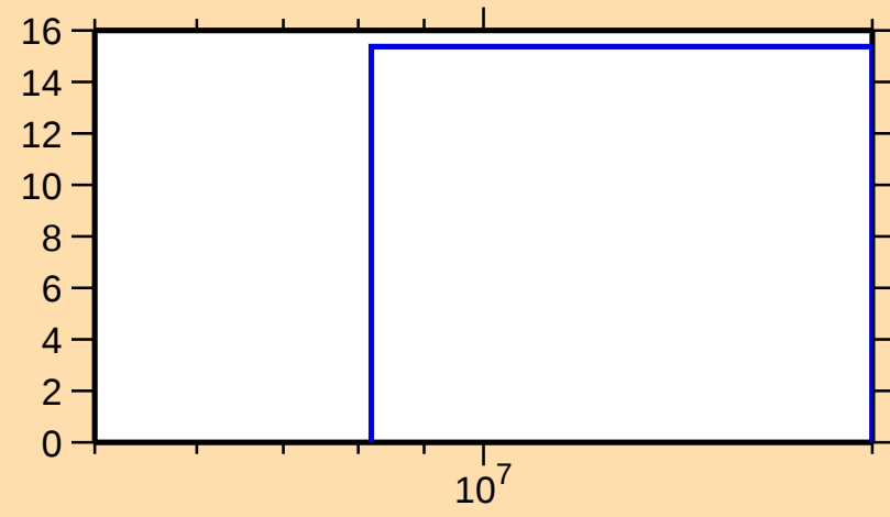
\Delta\sigma/\sigma vs. E for ^{45}\text{K}(n,\text{el.})
