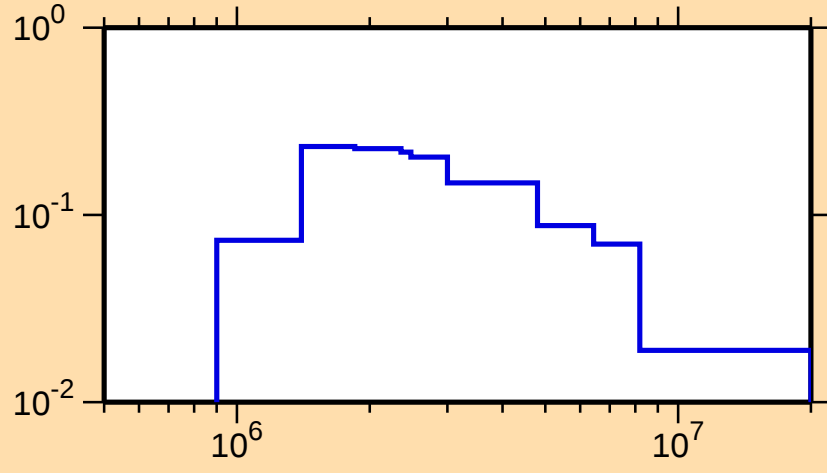
\sigma vs. E for ^{45}\text{K}(n,n_3)
