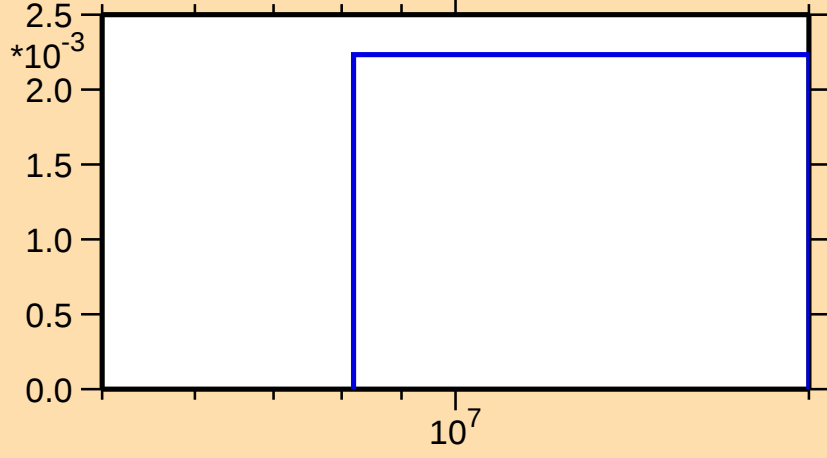
\sigma vs. E for ^{45}\text{K}(n,d)
