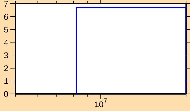
\Delta\sigma/\sigma vs. E for ^{45}\text{K}(n,2n)
