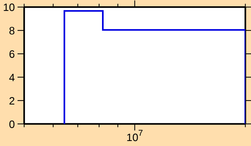
\Delta\sigma/\sigma vs. E for ^{45}\text{K}(\text{n},\text{tot.})
