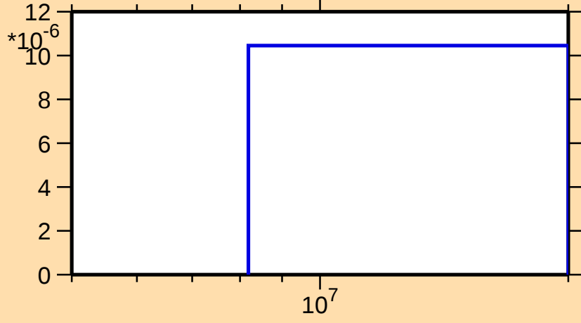
\sigma vs. E for ^{45}\text{K}(n,t)
