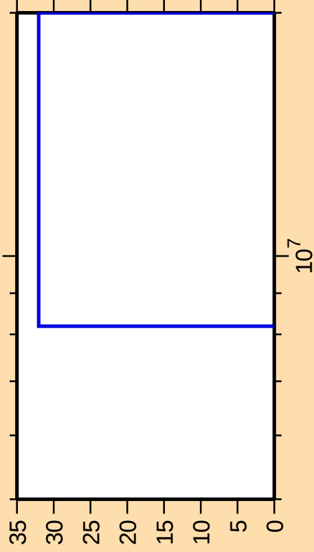
\Delta\sigma/\sigma vs. E for ^{45}\text{K}(n,3n)
