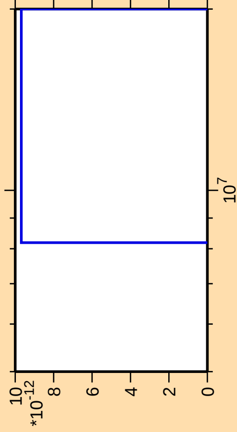
\Delta\sigma/\sigma vs. E for ^{45}\text{K}(n,\text{He}3)
