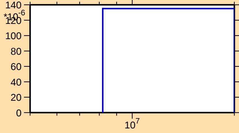
\sigma vs. E for ^{45}\text{K}(n,3n)
