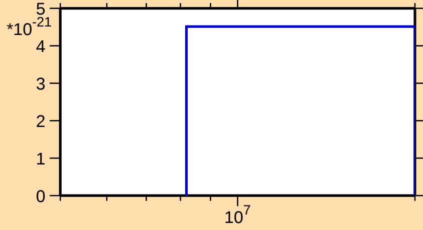
\sigma vs. E for ^{45}\text{K}(n,2n\alpha)
