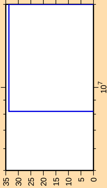
\Delta\sigma/\sigma vs. E for ^{45}\text{K}(n,n_1)
