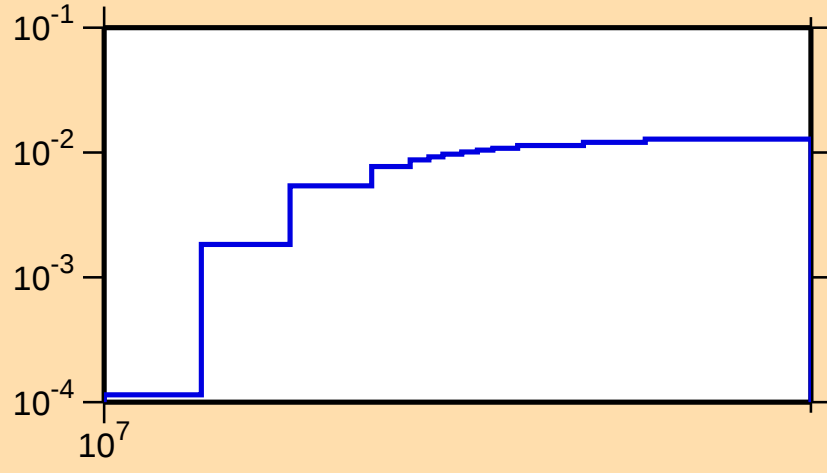
\sigma vs. E for ^{75}\text{Kr}(n,2n)
