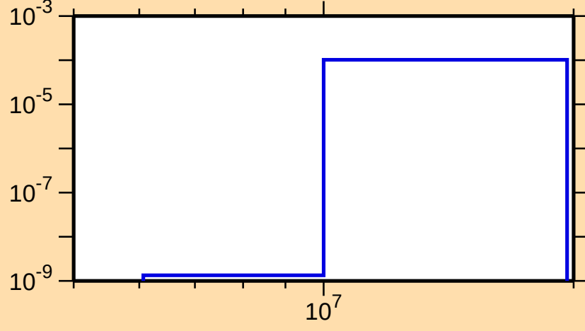
\sigma vs. E for ^{75}\text{Kr}(n,\text{He3})
