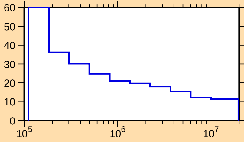
\Delta\sigma/\sigma vs. E for ^{75}\text{Kr}(\text{n,nonel.})
