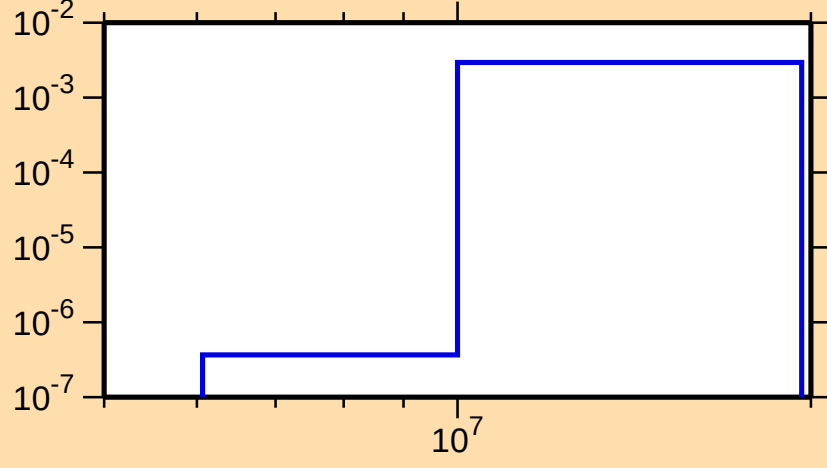
\sigma vs. E for ^{75}\text{Kr}(n,n\alpha)
