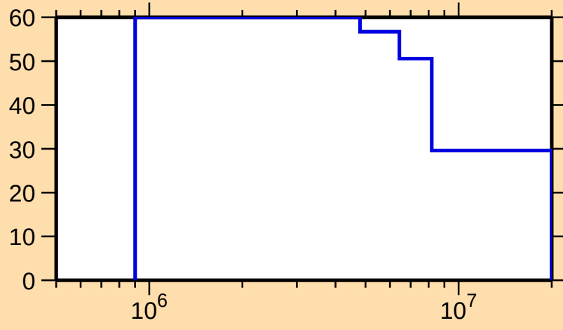
\Delta\sigma/\sigma vs. E for ^{75}\text{Kr}(n,n\text{cont.})
