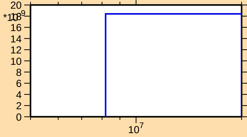
\sigma vs. E for ^{75}\text{Kr}(n,\text{nd})
