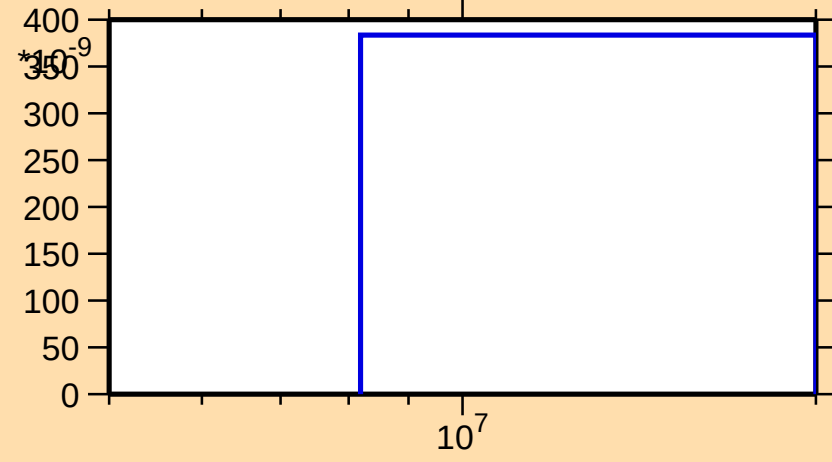
\sigma vs. E for ^{75}\text{Kr}(n,\text{pt})
