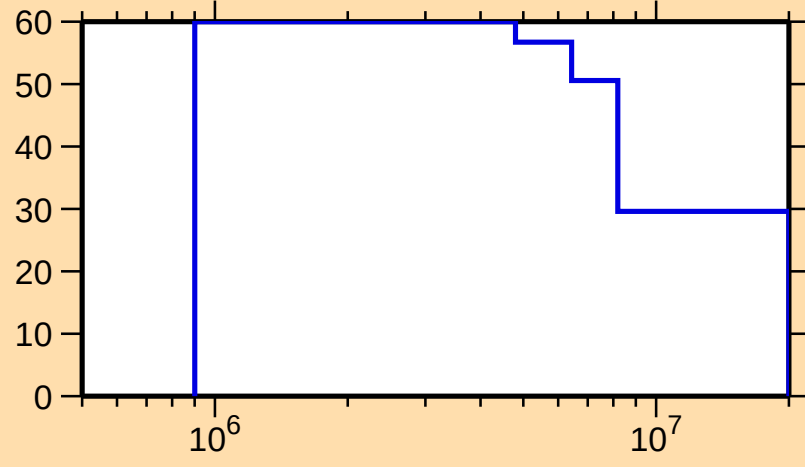
\Delta\sigma/\sigma vs. E for ^{75}\text{Kr}(n,n\text{cont.})
