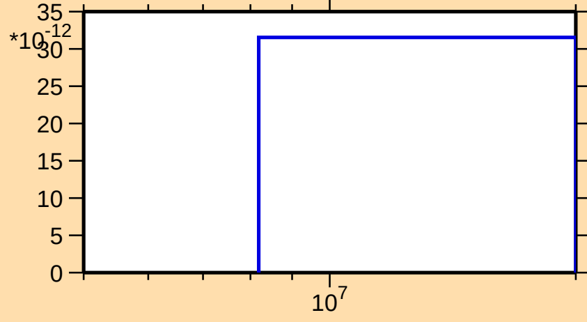
\sigma vs. E for ^{75}\text{Kr}(n,2n\alpha)
