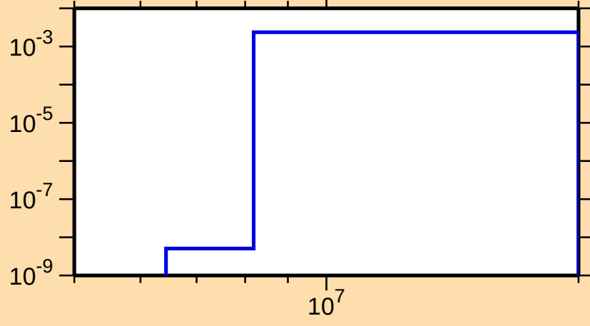
\sigma vs. E for ^{75}\text{Kr}(n,n\alpha)
