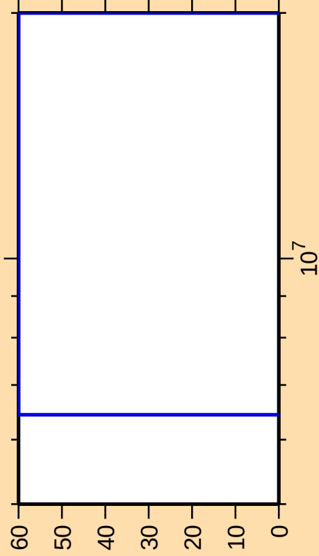
\Delta\sigma/\sigma vs. E for ^{75}\text{Kr}(n,n\alpha)
