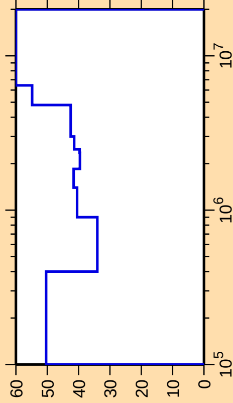
\Delta\sigma/\sigma vs. E for ^{75}\text{Kr}(n,p)
