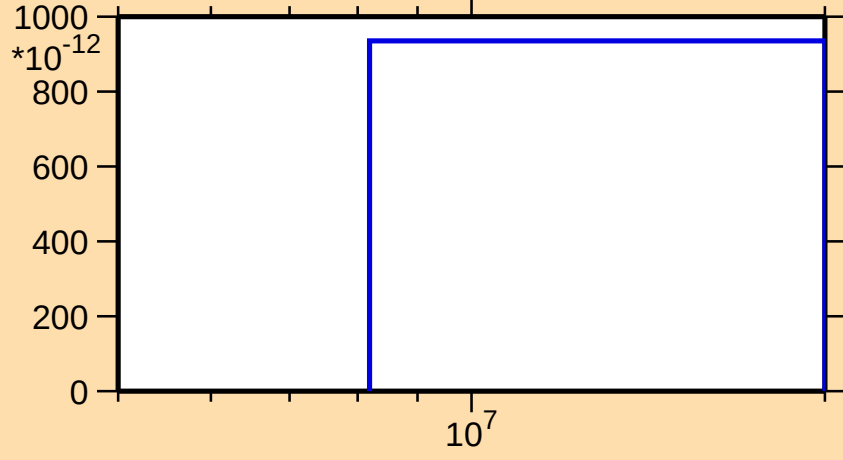
\sigma vs. E for ^{75}\text{Kr}(\text{mt } 34)
