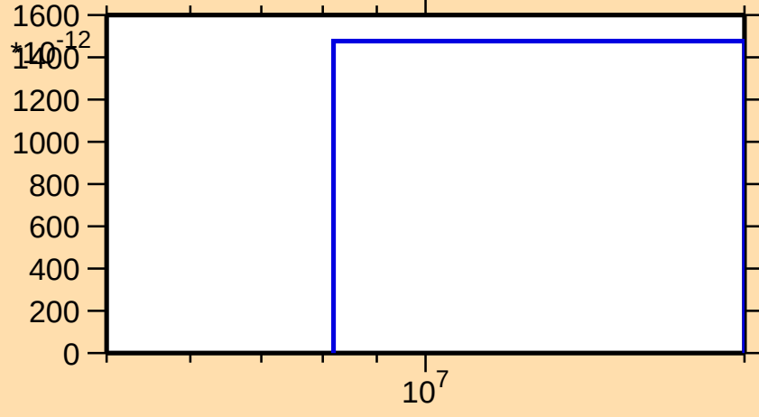
\sigma vs. E for ^{75}\text{Kr}(\text{mt } 45)
