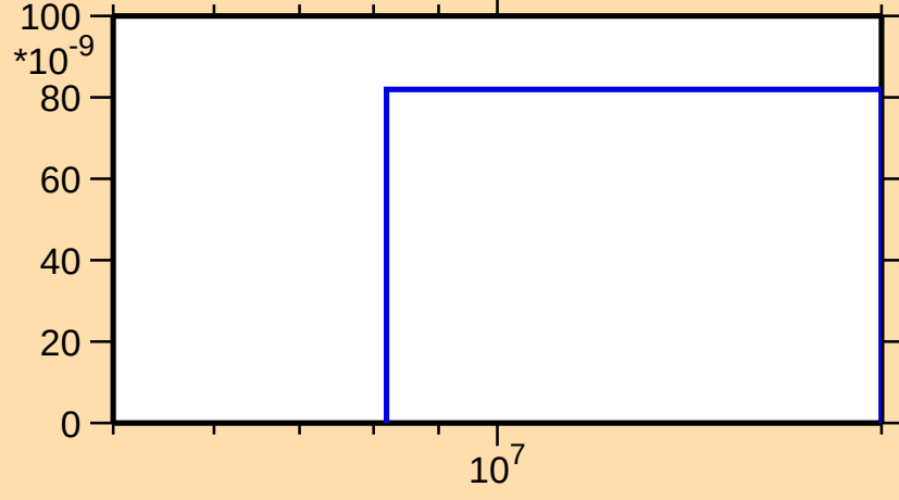
\sigma vs. E for ^{75}\text{Kr}(n,2np)
