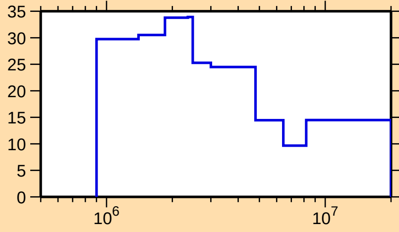
\Delta\sigma/\sigma vs. E for ^{75}\text{Kr}(n,\text{el.})
