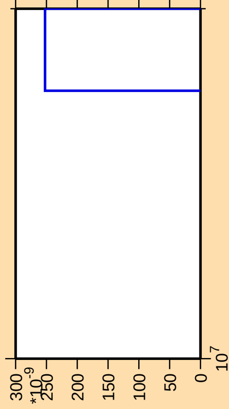
\Delta\sigma/\sigma vs. E for ^{80}\text{Kr}(\text{mt } 34)
