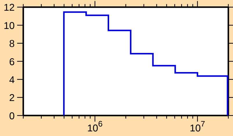
\Delta\sigma/\sigma vs. E for ^{80}\text{Kr}(n,\text{nonel.})
