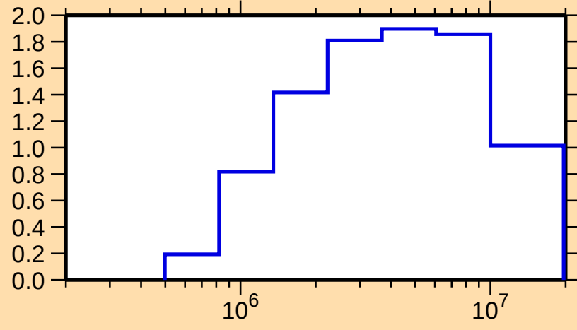
\sigma vs. E for ^{80}\text{Kr}(n,\text{inel.})
