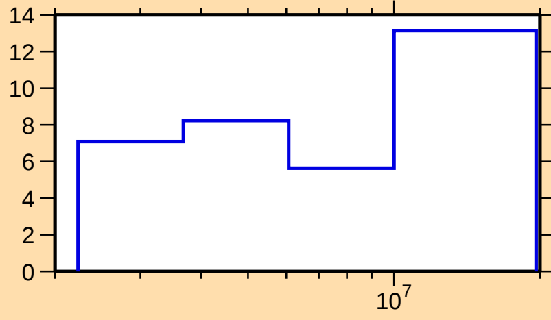
\Delta\sigma/\sigma vs. E for ^{80}\text{Kr}(\text{n},\text{el.})
