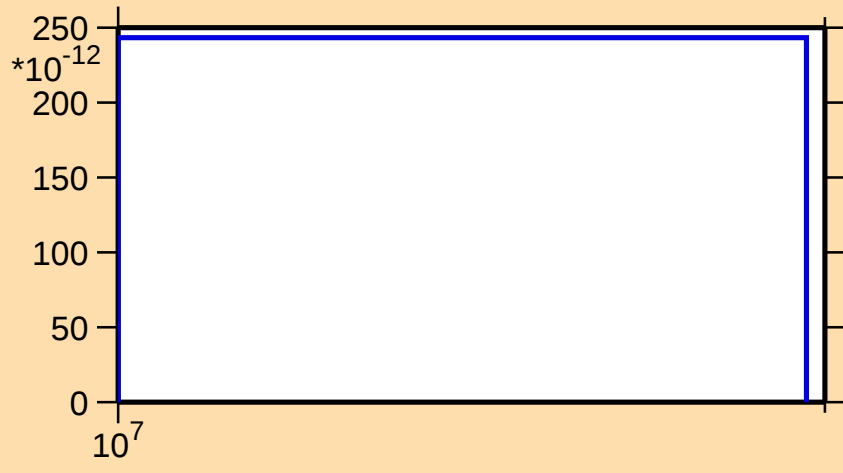
\sigma vs. E for ^{80}\text{Kr}(n,\text{pd})
