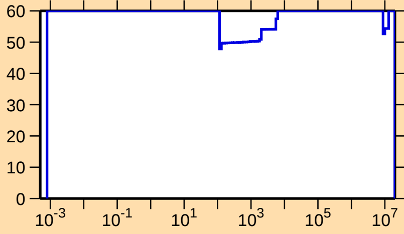
\Delta\sigma/\sigma vs. E for ^{81}\text{Kr}(n,\gamma)
