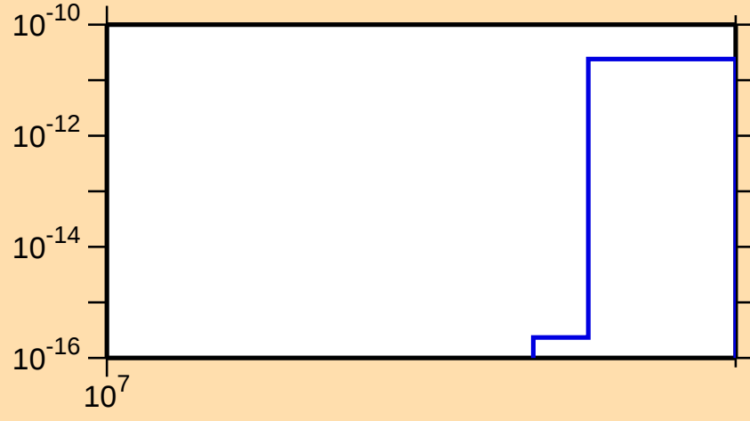
\sigma vs. E for ^{81}\text{Kr}(n,\text{pd})
