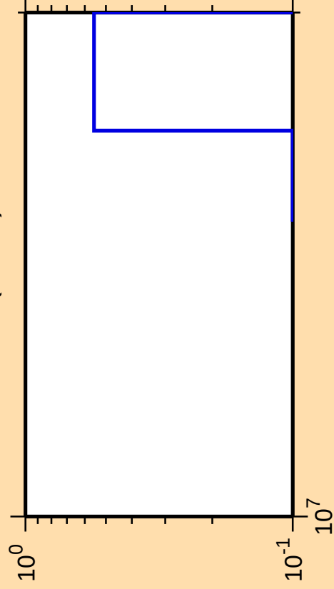
\Delta\sigma/\sigma vs. E for ^{81}\text{Kr} (mt 34)
