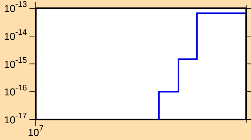
\sigma vs. E for ^{81}\text{Kr} (mt 34)
