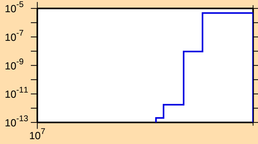
\sigma vs. E for ^{81}\text{Kr}(n,\text{nd})
