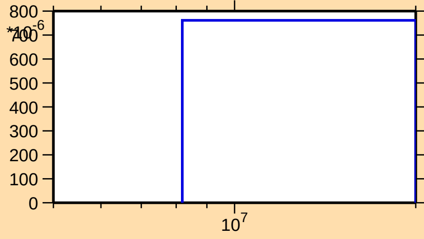
\sigma vs. E for ^{81}\text{Kr}(n,n\alpha)
