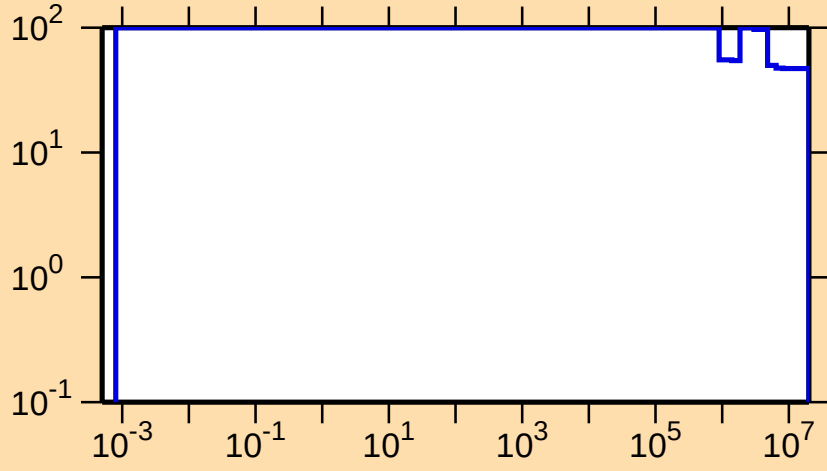
\Delta\sigma/\sigma vs. E for ^{81}\text{Kr}(n,p)
