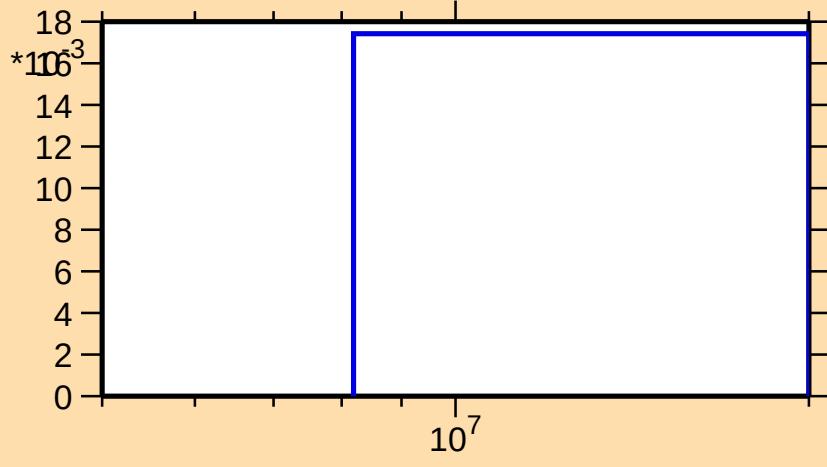
\sigma vs. E for ^{81}\text{Kr}(n,np)
