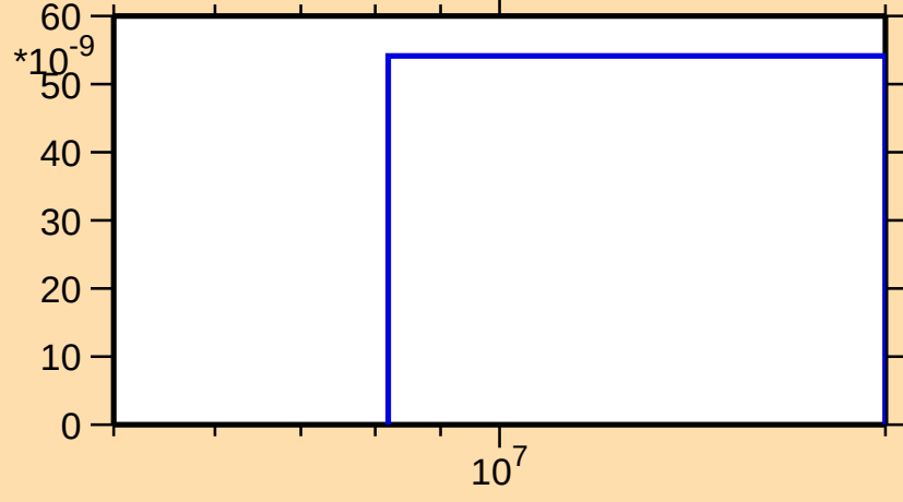
\sigma vs. E for ^{81}\text{Kr}(n,2np)
