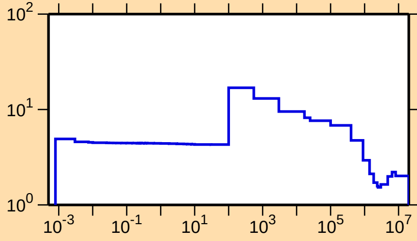
\sigma vs. E for ^{81}\text{Kr}(n,\text{el.})
