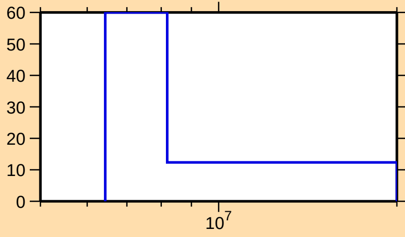
\Delta\sigma/\sigma vs. E for ^{81}\text{Kr}(n,2n)
