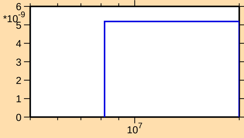
\sigma vs. E for ^{81}\text{Kr}(n,\text{He}3)
