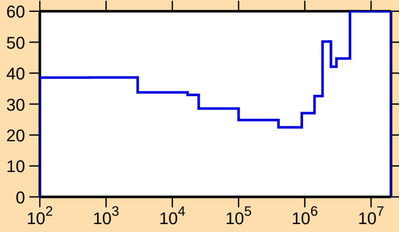
\Delta\sigma/\sigma vs. E for ^{81}\text{Kr}(n,n_1)
