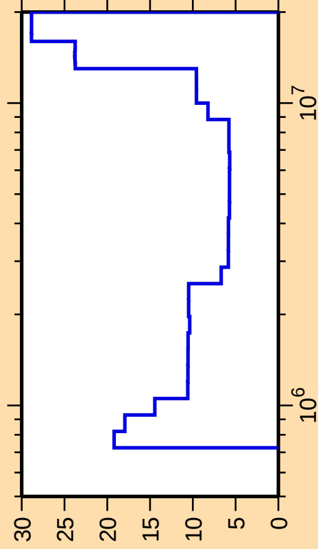
\Delta\sigma/\sigma vs. E for ^{82}\text{Kr}(\text{n,inel.})
