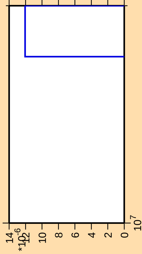
\Delta\sigma/\sigma vs. E for ^{82}\text{Kr}(n,\text{nt})
