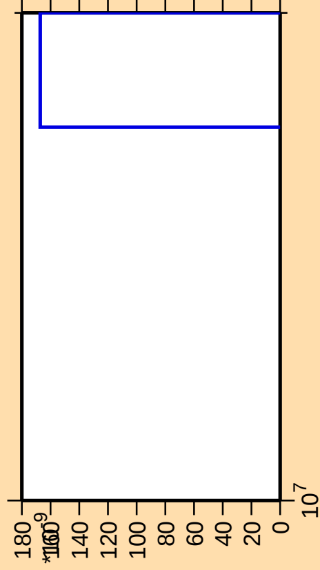
\Delta\sigma/\sigma vs. E for ^{82}\text{Kr} (mt 34)
