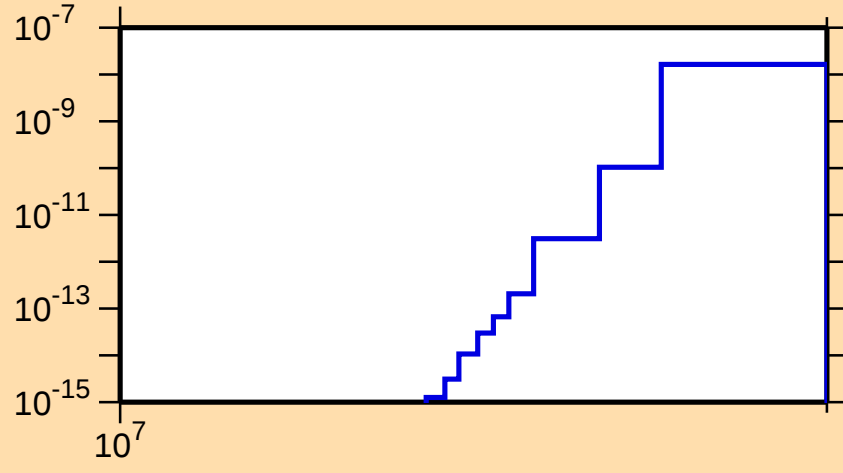
\sigma vs. E for ^{82}\text{Kr}(n,\text{He3})
