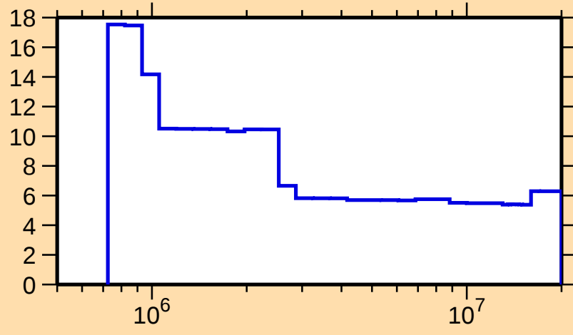
\Delta\sigma/\sigma vs. E for ^{82}\text{Kr}(\text{n,nonel.})
