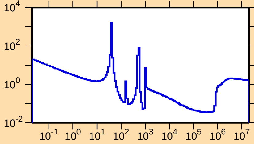
\sigma vs. E for ^{82}\text{Kr}(n,\text{nonel.})
