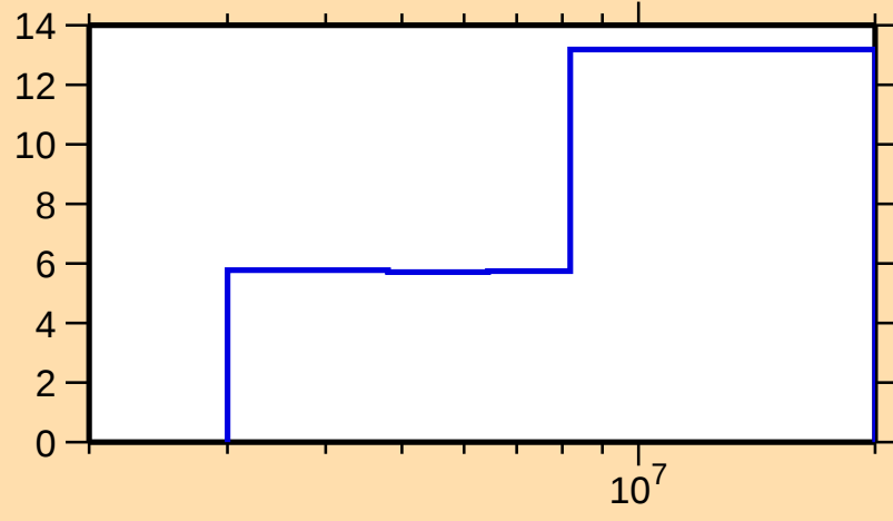
\Delta\sigma/\sigma vs. E for ^{82}\text{Kr}(\text{n},\text{inel.})
