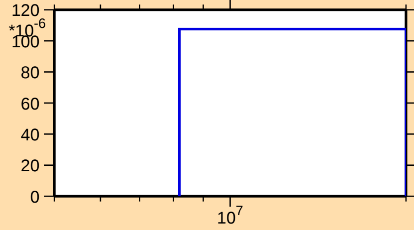
\sigma vs. E for ^{82}\text{Kr}(n,n\alpha)
