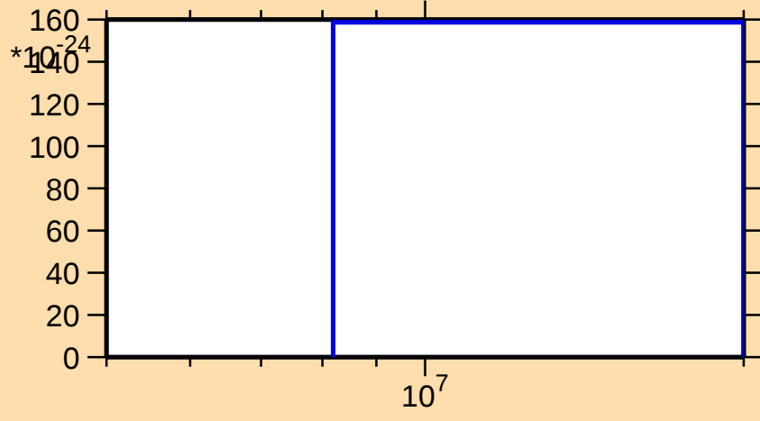
\sigma vs. E for ^{82}\text{Kr}(\text{mt } 34)
