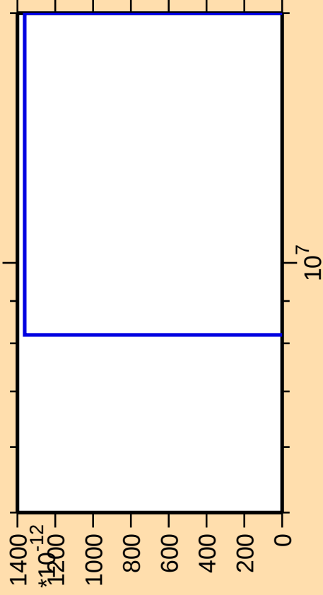
\Delta\sigma/\sigma vs. E for ^{82}\text{Kr}(\text{mt } 34)
