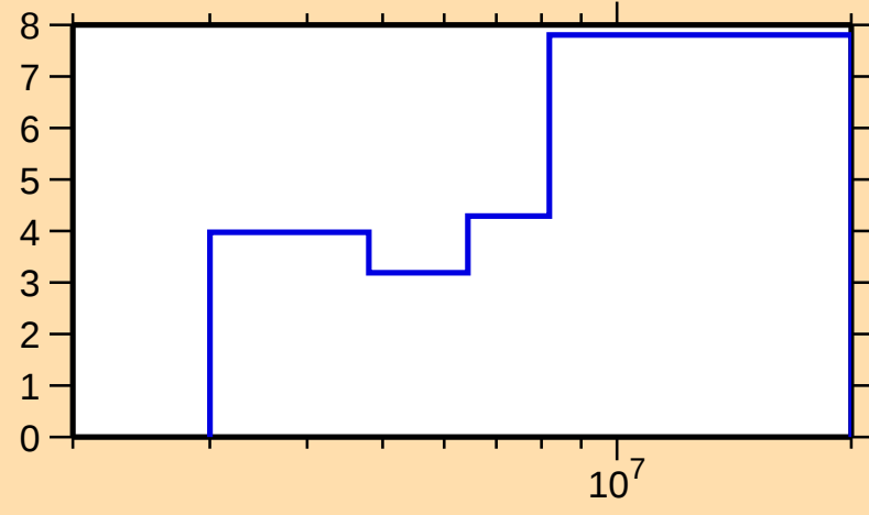
\Delta\sigma/\sigma vs. E for ^{82}\text{Kr}(\text{n},\text{tot.})
