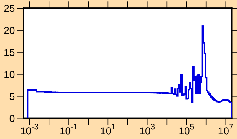
\sigma vs. E for ^{86}\text{Kr}(n,\text{tot.})
