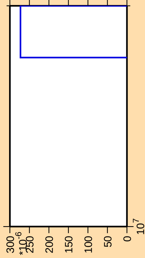
\Delta\sigma/\sigma vs. E for ^{86}\text{Kr}(n,\text{nd})
