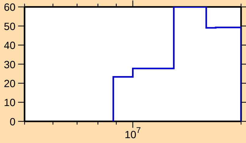
\Delta\sigma/\sigma vs. E for ^{91}\text{Kr}(n,2n)
