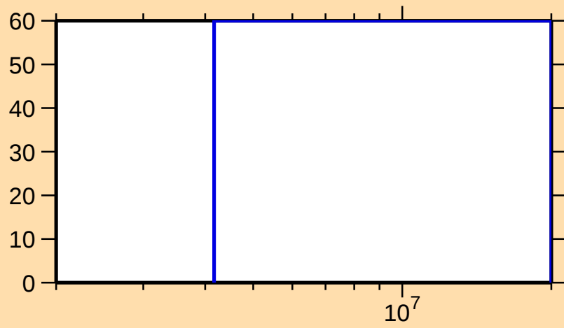
\Delta\sigma/\sigma vs. E for ^{91}\text{Kr}(n,\gamma)
