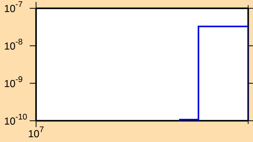
\sigma vs. E for ^{91}\text{Kr}(n,2n\alpha)
