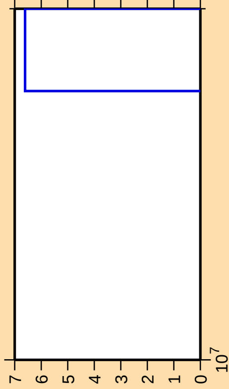
\Delta\sigma/\sigma vs. E for ^{91}\text{Kr}(n,2np)
