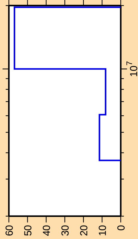
\Delta\sigma/\sigma vs. E for ^{91}\text{Kr}(n,2n)
