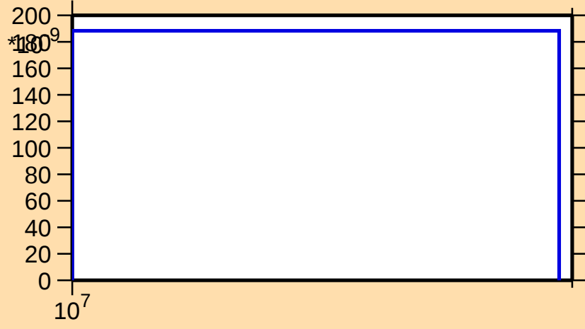
\sigma vs. E for ^{91}\text{Kr}(n,np)
