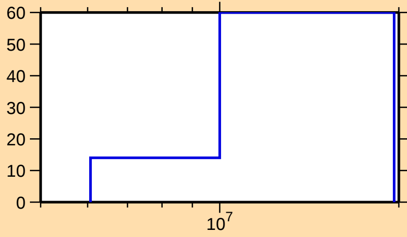
\Delta\sigma/\sigma vs. E for ^{91}\text{Kr}(n,p)
