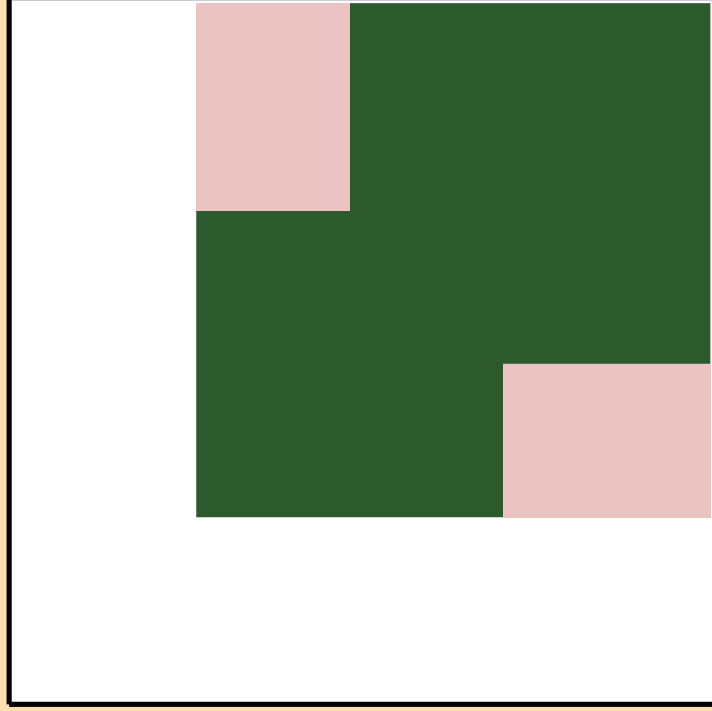
\sigma vs. E for ^{91}\text{Kr}(n,2n)
