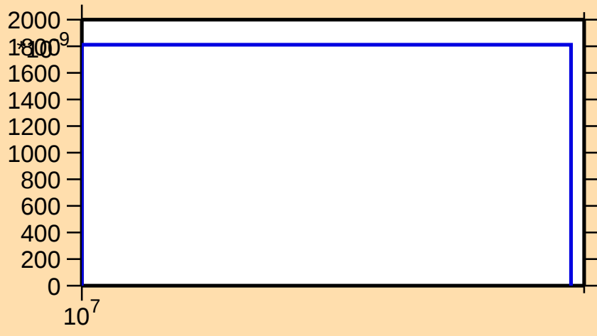
\sigma vs. E for ^{91}\text{Kr}(n,d)
