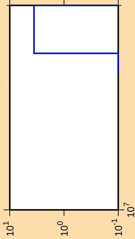
\Delta\sigma/\sigma vs. E for ^{119}\text{La}(n,2n\alpha)
