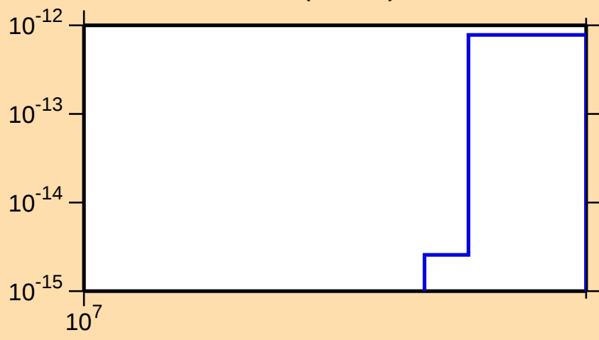
\sigma vs. E for ^{119}\text{La}(n,2n\alpha)
