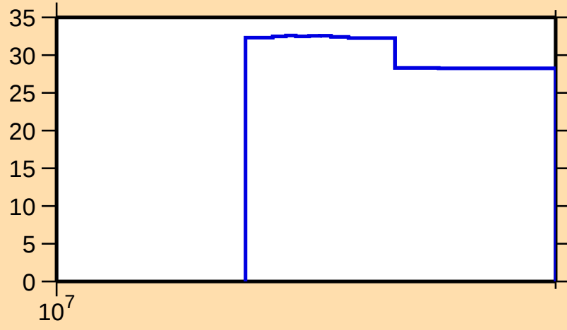
\Delta\sigma/\sigma vs. E for ^{119}\text{La}(n,\text{inel.})
