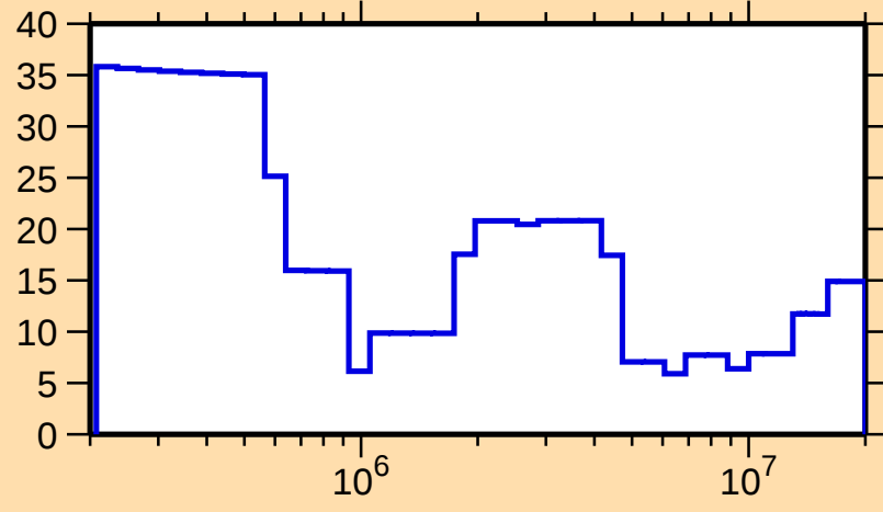
\Delta\sigma/\sigma vs. E for ^{119}\text{La}(n,\text{el.})
