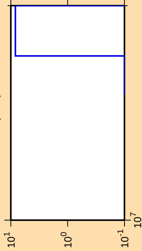
\Delta\sigma/\sigma vs. E for ^{119}\text{La}(n,nt)
