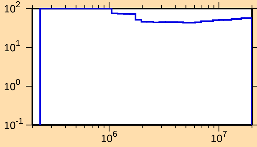
\Delta\sigma/\sigma vs. E for ^{119}\text{La}(n,n_1)
