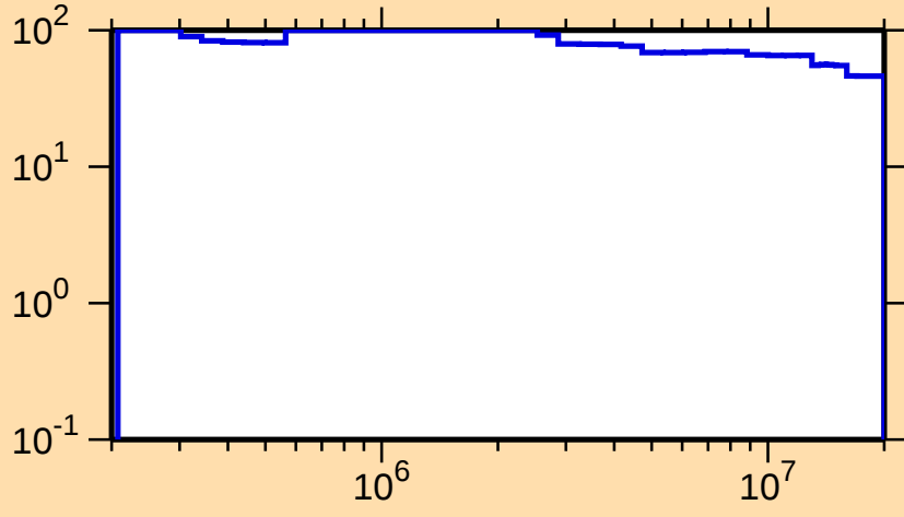
\Delta\sigma/\sigma vs. E for ^{119}\text{La}(n,n\text{cont.})
