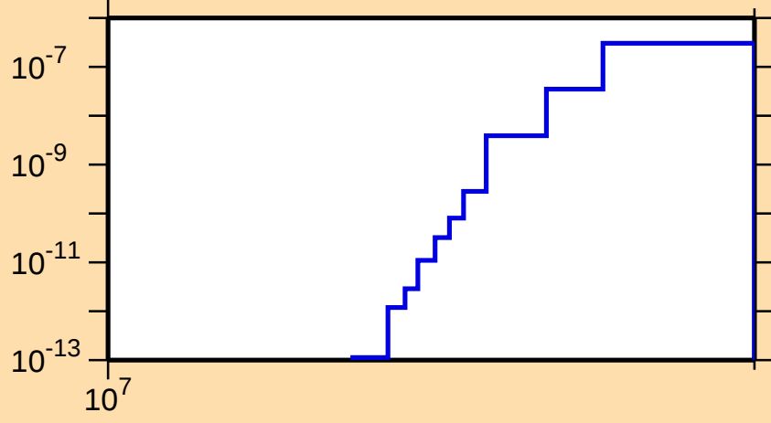
\sigma vs. E for ^{119}\text{La}(n,\text{nd})
