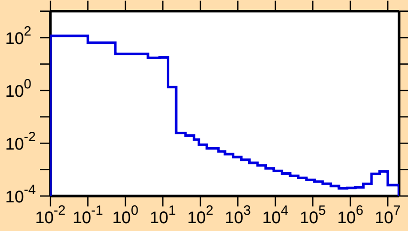
\sigma vs. E for ^{119}\text{La}(n,\gamma)
