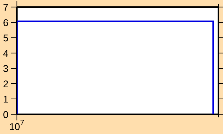
\Delta\sigma/\sigma vs. E for ^{119}\text{La}(n,\text{nonel.})
