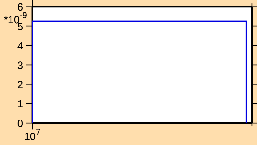
\sigma vs. E for ^{119}\text{La}(n,\text{nd})
