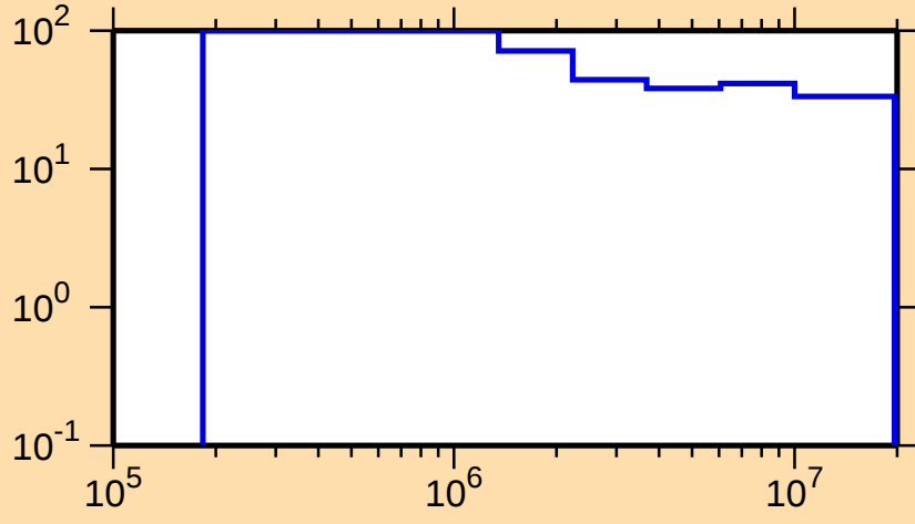
\Delta\sigma/\sigma vs. E for ^{119}\text{La}(n,\text{inel.})
