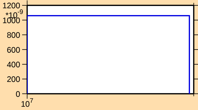
\sigma vs. E for ^{119}\text{La}(n,2np)
