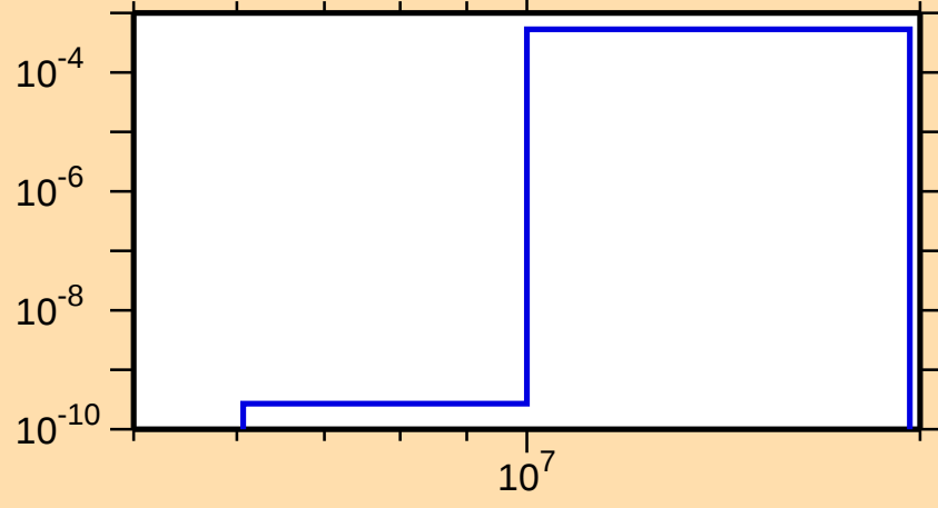
\sigma vs. E for ^{119}\text{La}(n,t)
