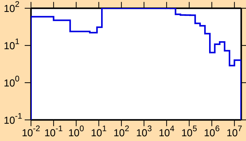
\Delta\sigma/\sigma vs. E for ^{119}\text{La}(n,\text{tot.})
