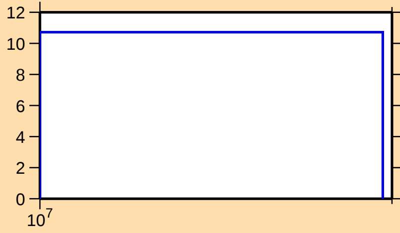
\Delta\sigma/\sigma vs. E for ^{119}\text{La}(n,\text{el.})
