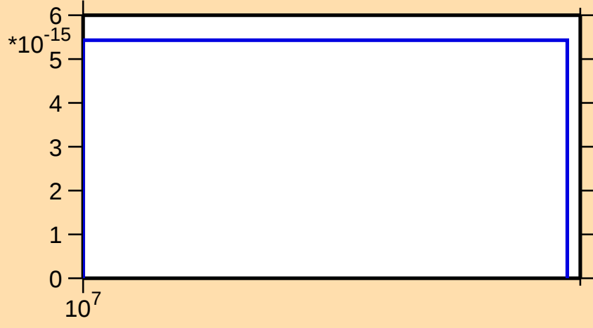
\sigma vs. E for ^{119}\text{La}(n,2n\alpha)
