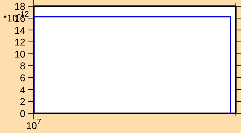
\sigma vs. E for ^{119}\text{La} (mt 34)
