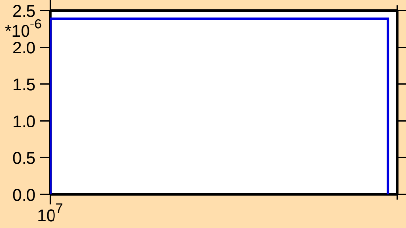
\sigma vs. E for ^{119}\text{La}(n,2n)
