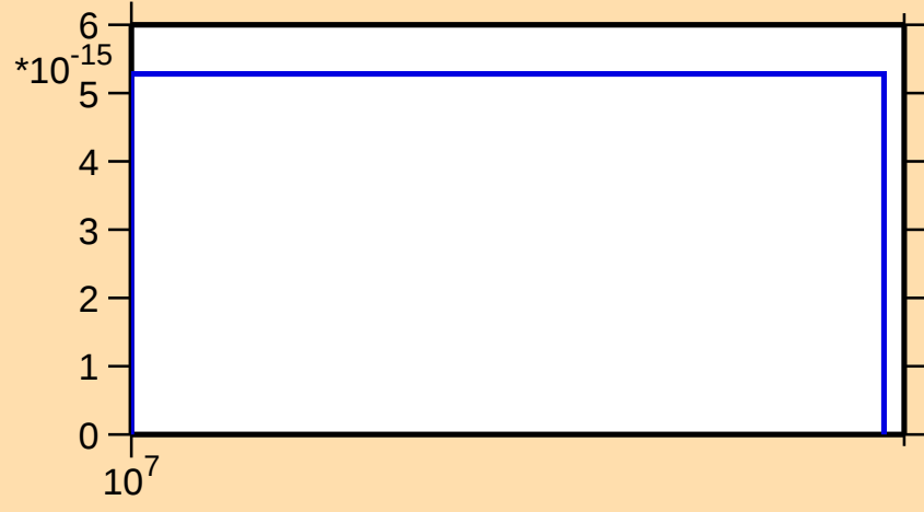
\sigma vs. E for ^{119}\text{La}(n,nt)
