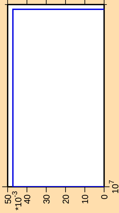
\Delta\sigma/\sigma vs. E for ^{119}\text{La}(n,nt)
