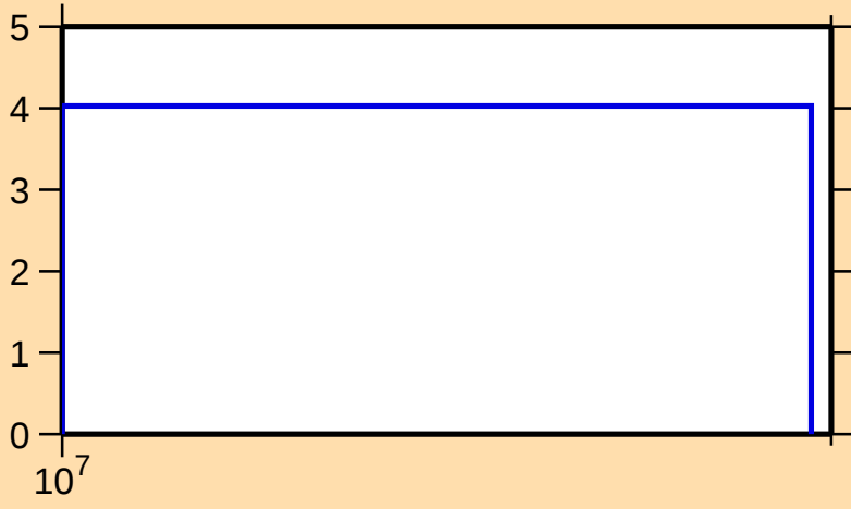
\Delta\sigma/\sigma vs. E for ^{119}\text{La}(n,\text{tot.})
