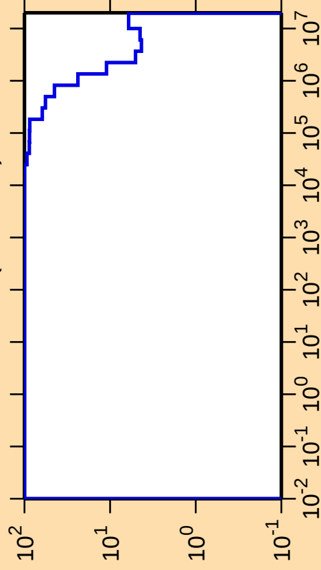
\Delta\sigma/\sigma vs. E for ^{119}\text{La}(n,\text{nonel.})
