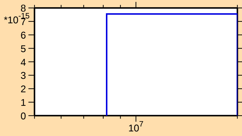
\sigma vs. E for ^{119}\text{La}(n,nt)
