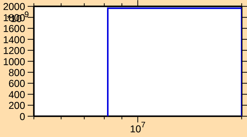
\sigma vs. E for ^{119}\text{La}(n,2n)
