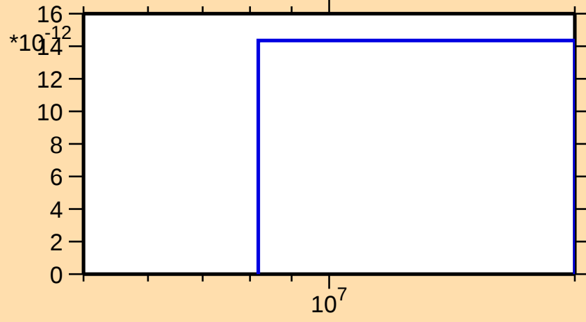
\sigma vs. E for ^{119}\text{La}(\text{mt } 34)
