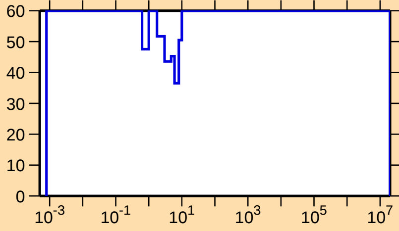
\Delta\sigma/\sigma vs. E for ^{119}\text{La}(n,\gamma)
