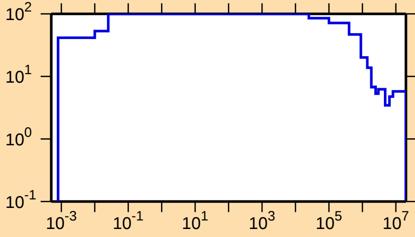
\Delta\sigma/\sigma vs. E for ^{119}\text{La}(n,\text{nonel.})
