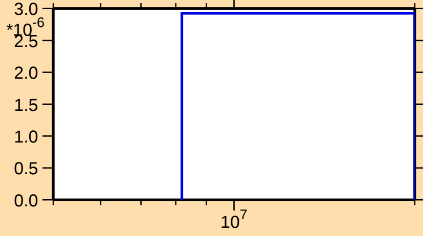
\sigma vs. E for ^{119}\text{La}(n,\text{pt})
