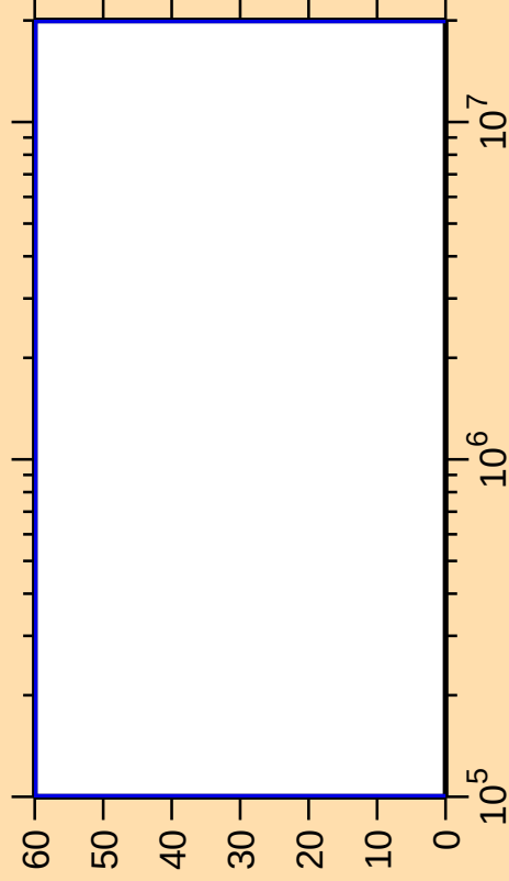
\Delta\sigma/\sigma vs. E for ^{123}\text{La}(n,\text{ncont.})
