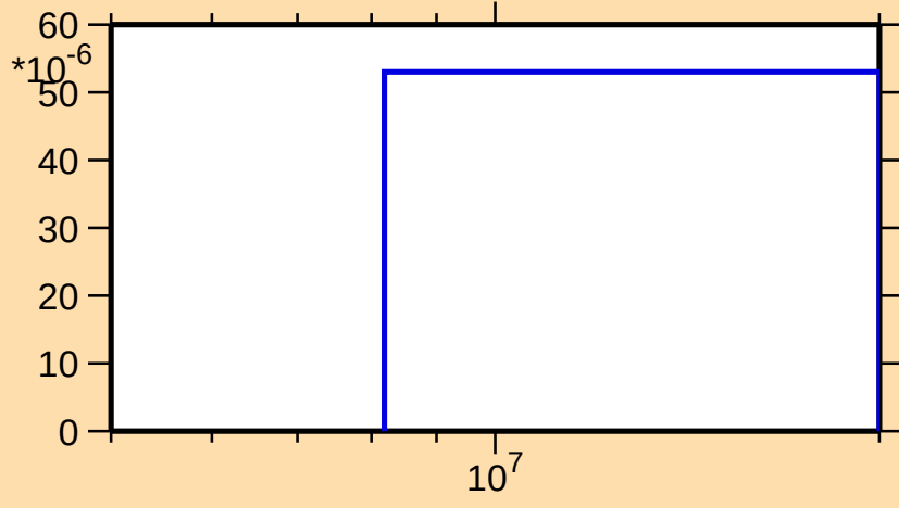
\sigma vs. E for ^{123}\text{La}(n,\text{pd})
