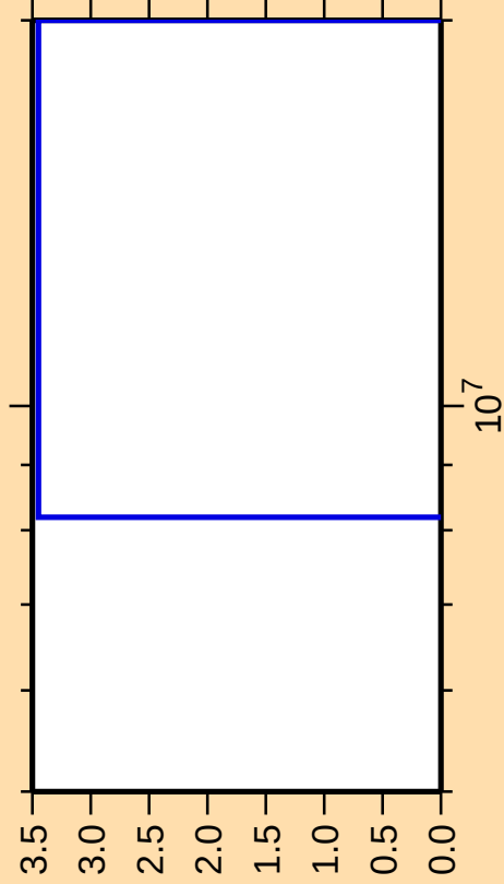
\Delta\sigma/\sigma vs. E for ^{123}\text{La}(n,nt)
