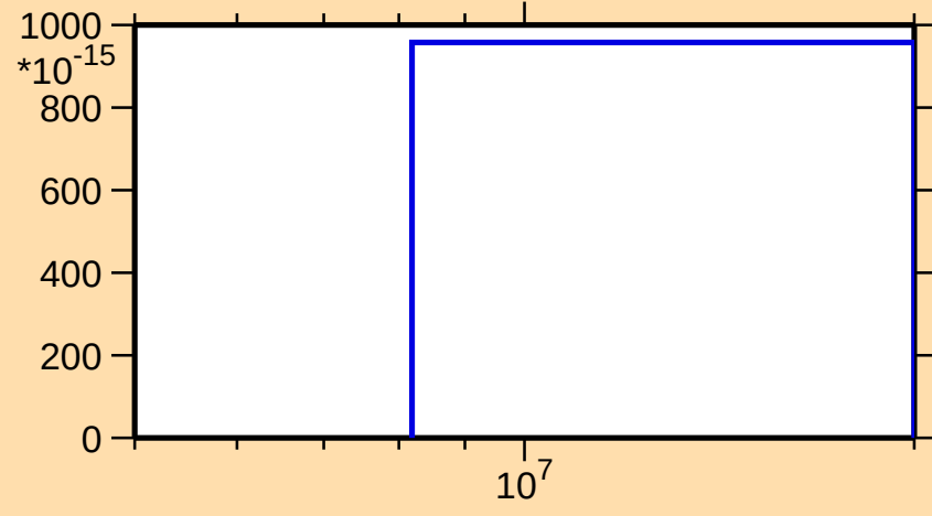
\sigma vs. E for ^{123}\text{La}(n,2n\alpha)
