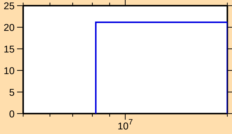
\Delta\sigma/\sigma vs. E for ^{123}\text{La}(n,\text{tot.})
