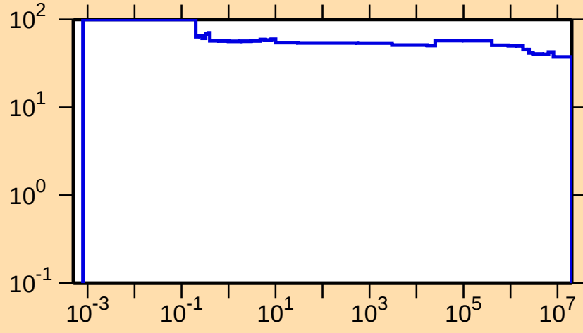
\Delta\sigma/\sigma vs. E for ^{123}\text{La}(n,\text{nonel.})
