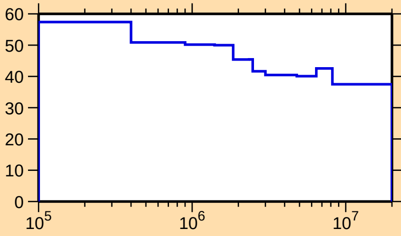
\Delta\sigma/\sigma vs. E for ^{123}\text{La}(n,n\text{onel.})
