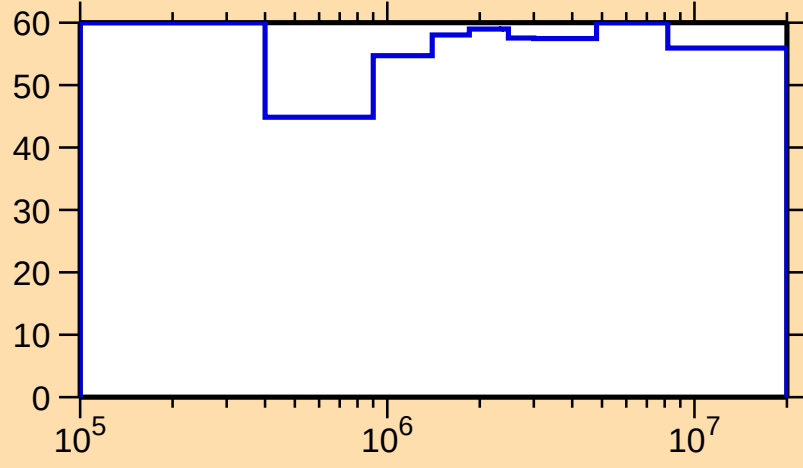
\Delta\sigma/\sigma vs. E for ^{123}\text{La}(n,\text{inel.})
