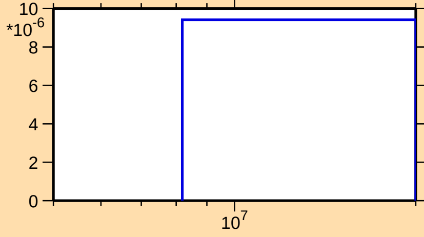
\sigma vs. E for ^{123}\text{La}(n,2np)
