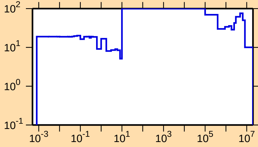
\Delta\sigma/\sigma vs. E for ^{123}\text{La}(n,\text{el.})
