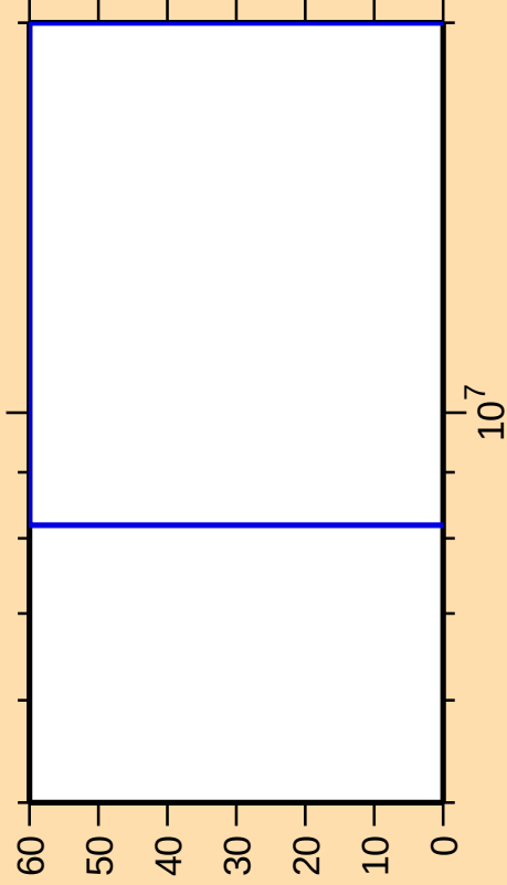
\Delta\sigma/\sigma vs. E for ^{123}\text{La}(n,nd)
