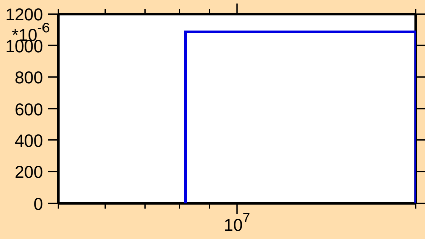
\sigma vs. E for ^{123}\text{La}(n,2n)
