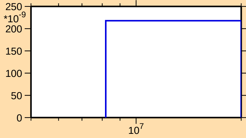
\sigma vs. E for ^{123}\text{La}(\text{mt117})
