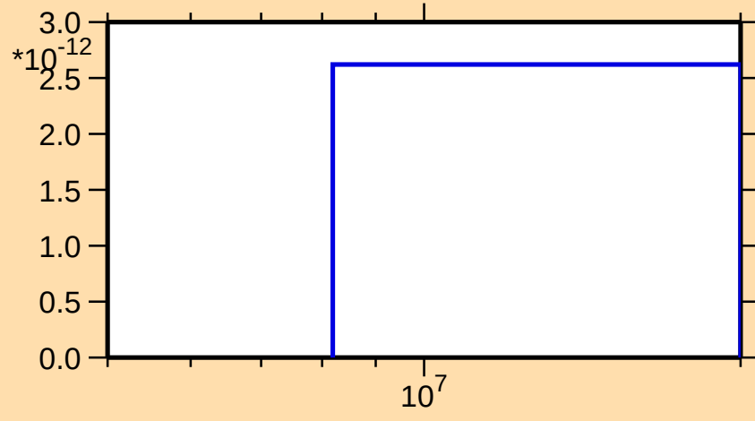
\sigma vs. E for ^{123}\text{La} (mt 34)
