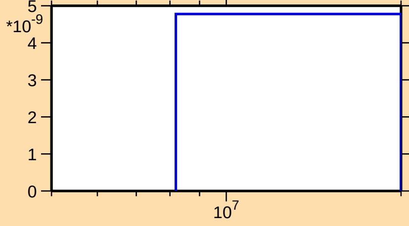
\sigma vs. E for ^{123}\text{La}(n,\text{pt})
