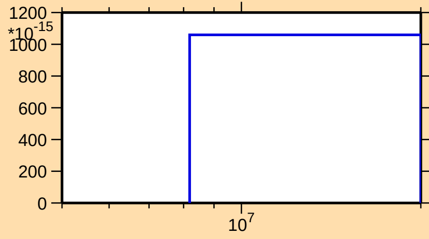
\sigma vs. E for ^{123}\text{La}(n,nt)
