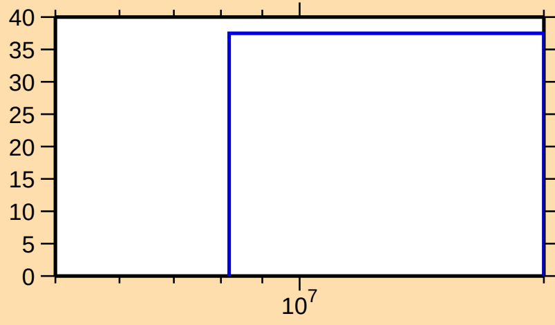
\Delta\sigma/\sigma vs. E for ^{123}\text{La}(n,\text{nonel.})
