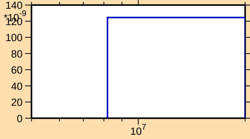
\sigma vs. E for ^{123}\text{La}(n,nd)
