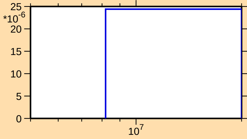
\sigma vs. E for ^{123}\text{La} (mt 45)
