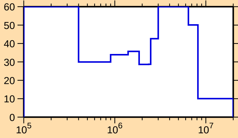
\Delta\sigma/\sigma vs. E for ^{123}\text{La}(n,\text{el.})
