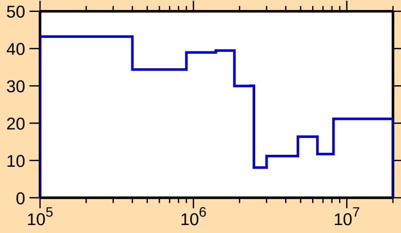
\Delta\sigma/\sigma vs. E for ^{123}\text{La}(n,\text{tot.})
