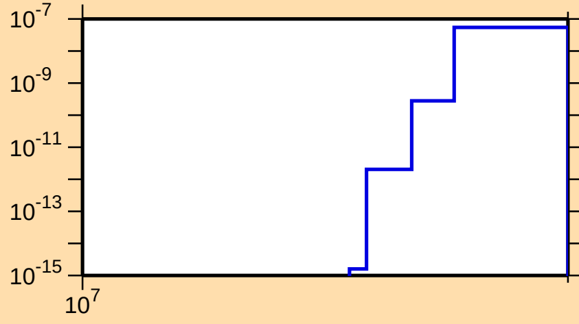
\sigma vs. E for ^{127}\text{La}(n,2n\alpha)
