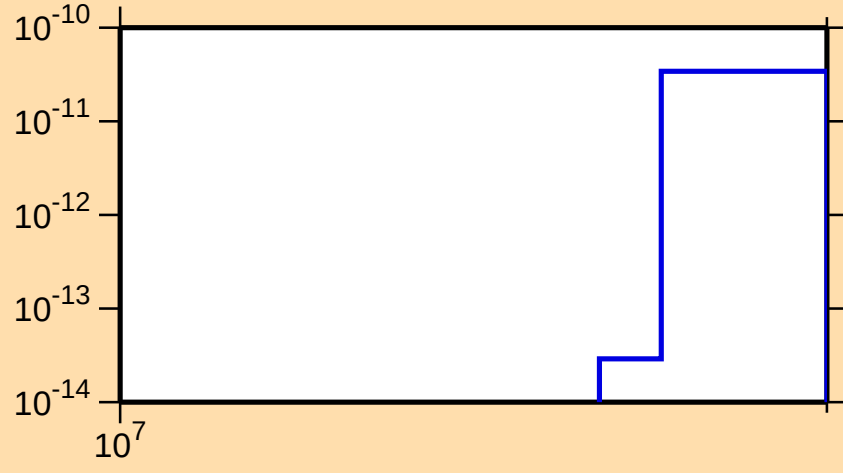
\sigma vs. E for ^{127}\text{La} (mt 34)
