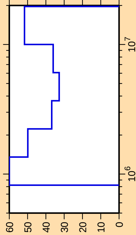
\Delta\sigma/\sigma vs. E for ^{127}\text{La}(n,n\text{cont.})
