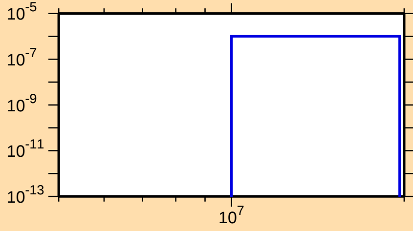
\sigma vs. E for ^{127}\text{La} (mt 45)
