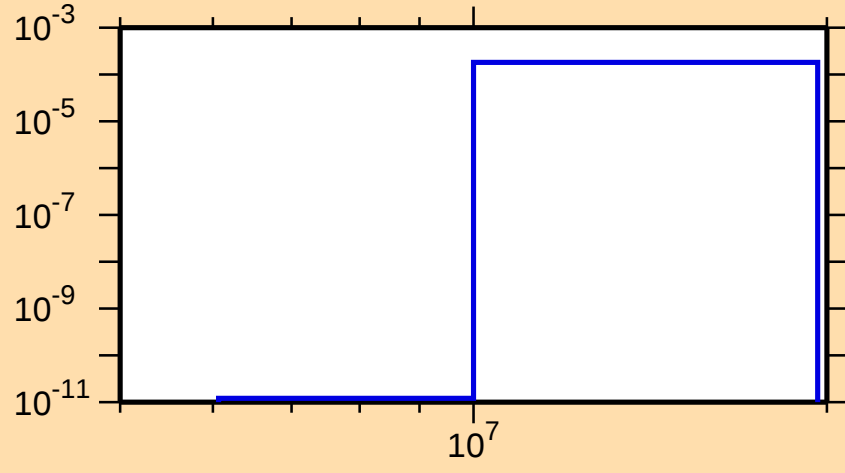
\sigma vs. E for ^{127}\text{La}(n,t)
