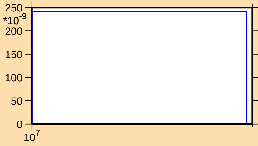
\sigma vs. E for ^{127}\text{La}(n,\text{nd})
