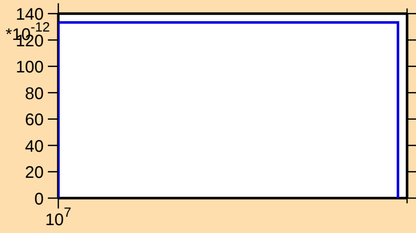
\sigma vs. E for ^{127}\text{La}(n,nt)
