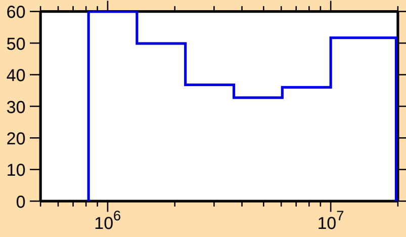
\Delta\sigma/\sigma vs. E for ^{127}\text{La}(n,n\text{cont.})
