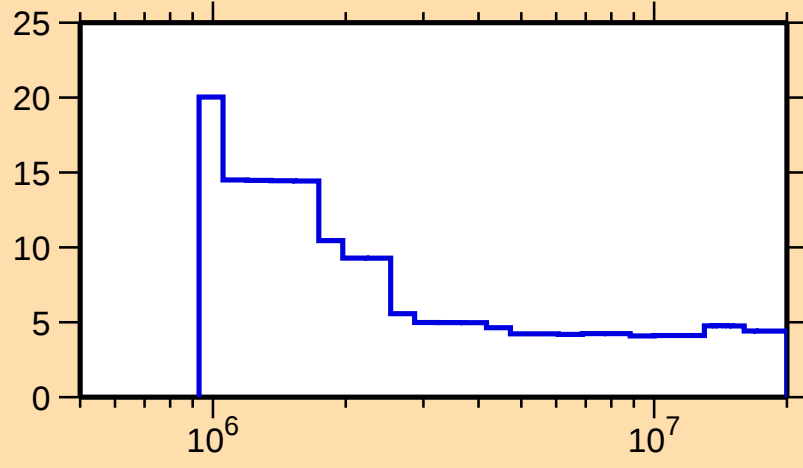
\Delta\sigma/\sigma vs. E for ^{130}\text{La}(n,\text{nonel.})
