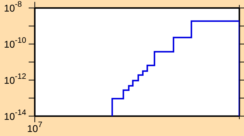
\sigma vs. E for ^{130}\text{La}(\text{mt117})
