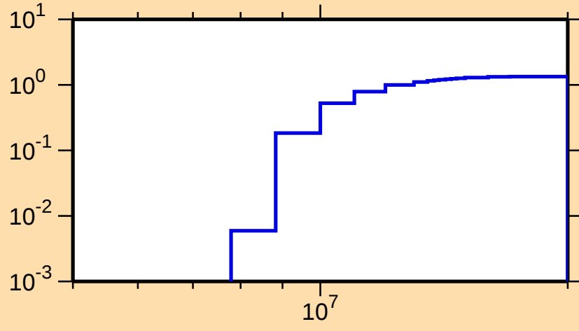
\sigma vs. E for ^{130}\text{La}(n,2n)
