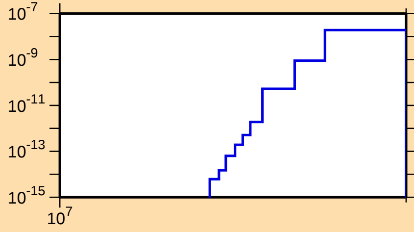
\sigma vs. E for ^{130}\text{La}(n,\text{pd})
