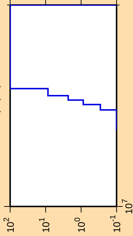
\Delta\sigma/\sigma vs. E for ^{130}\text{La}(n,\text{pd})
