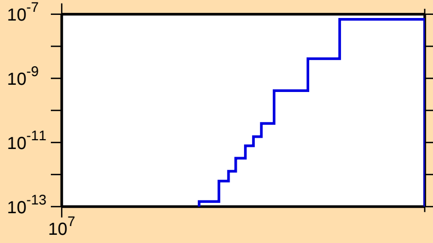
\sigma vs. E for ^{130}\text{La}(\text{mt } 45)
