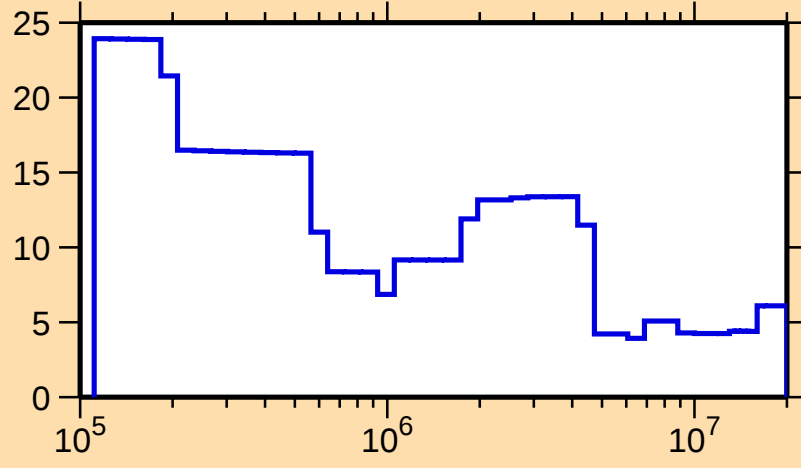
\Delta\sigma/\sigma vs. E for ^{130}\text{La}(n,\text{el.})
