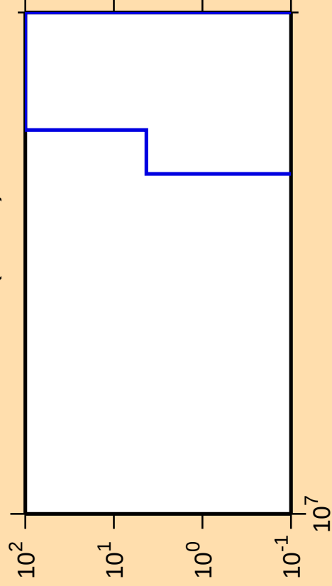
\Delta\sigma/\sigma vs. E for ^{130}\text{La} (mt 34)
