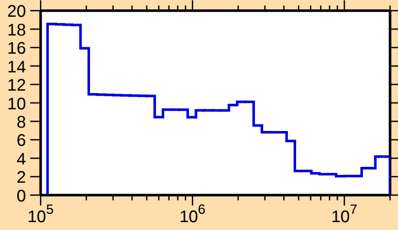
\Delta\sigma/\sigma vs. E for ^{130}\text{La}(n,\text{tot.})
