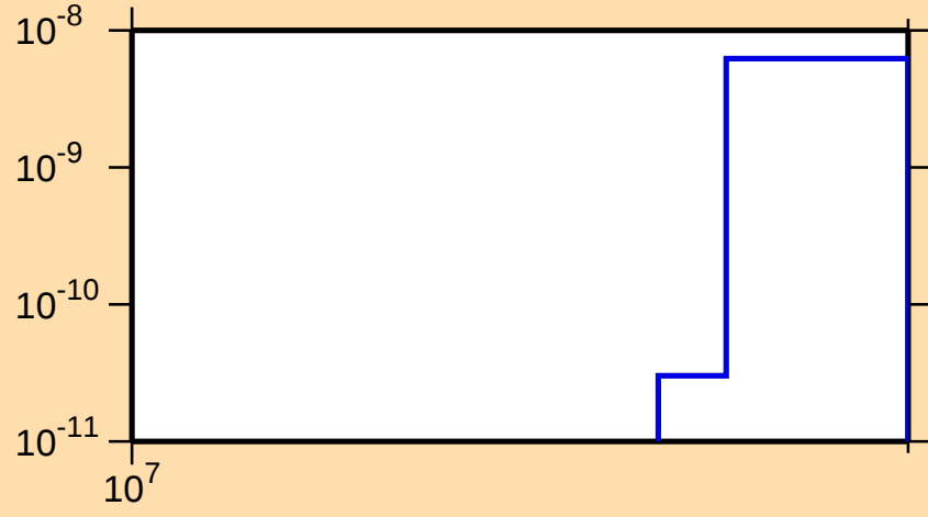
\sigma vs. E for ^{130}\text{La}(n,\text{pt})
