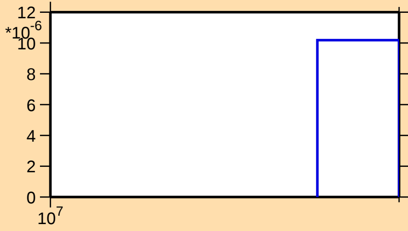
\sigma vs. E for ^{130}\text{La}(n,3n)
