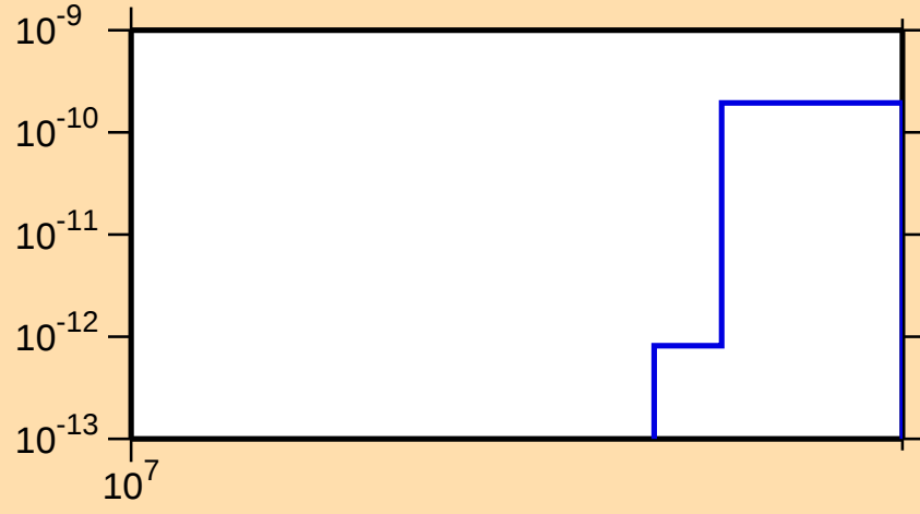
\sigma vs. E for ^{130}\text{La} (mt 34)
