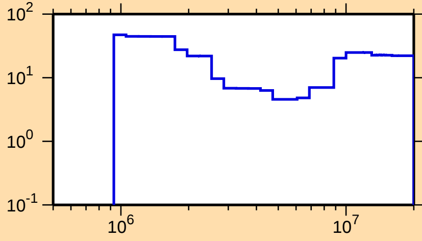
\Delta\sigma/\sigma vs. E for ^{130}\text{La}(n,\text{inel.})
