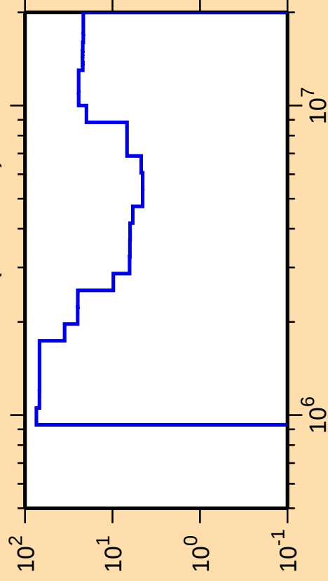
\Delta\sigma/\sigma vs. E for ^{130}\text{La}(n,n\text{cont.})
