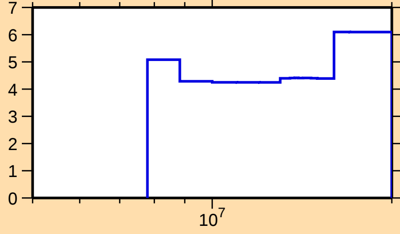
\Delta\sigma/\sigma vs. E for ^{130}\text{La}(n,\text{el.})
