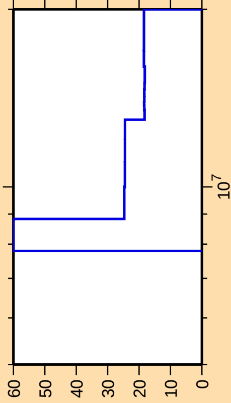
\Delta\sigma/\sigma vs. E for ^{130}\text{La}(n,2n)
