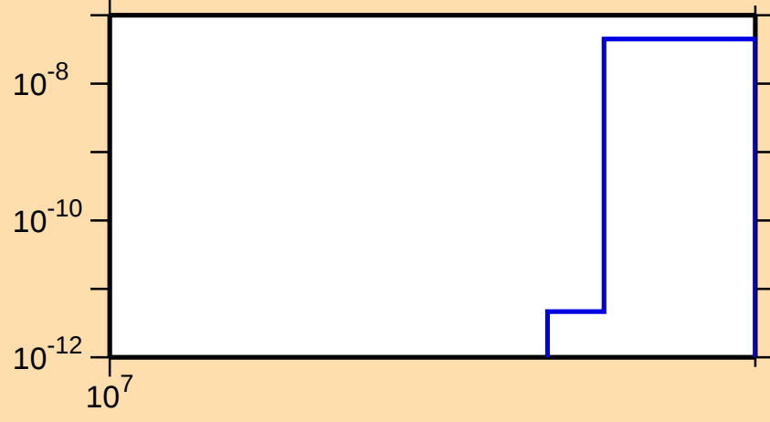
\sigma vs. E for ^{130}\text{La}(n,nt)
