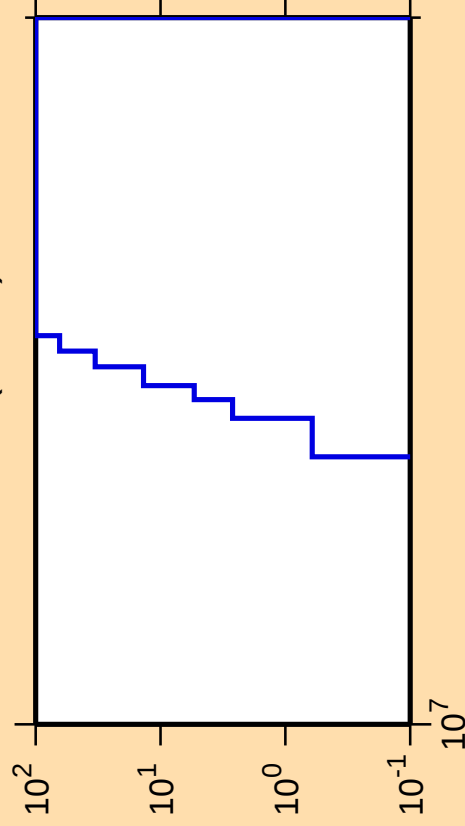
\Delta\sigma/\sigma vs. E for ^{130}\text{La}(\text{mt } 45)
