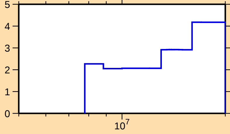
\Delta\sigma/\sigma vs. E for ^{130}\text{La}(n,\text{tot.})
