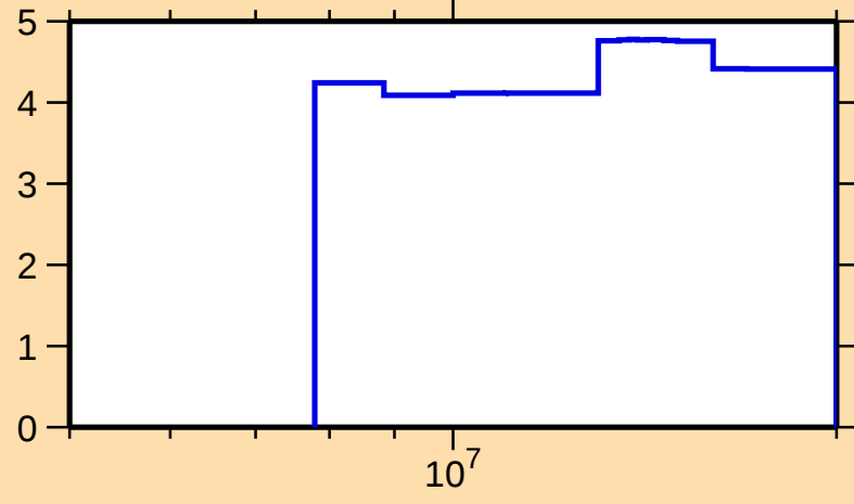
\Delta\sigma/\sigma vs. E for ^{130}\text{La}(n,\text{nonel.})
