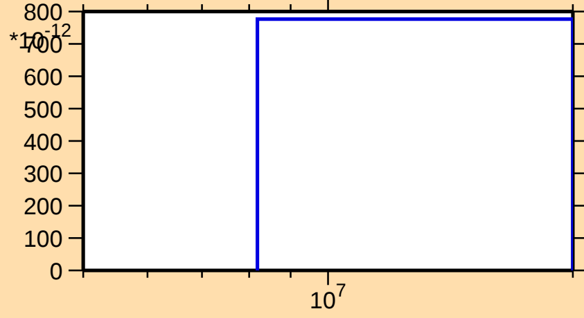
\sigma vs. E for ^{130}\text{La}(\text{mt } 45)
