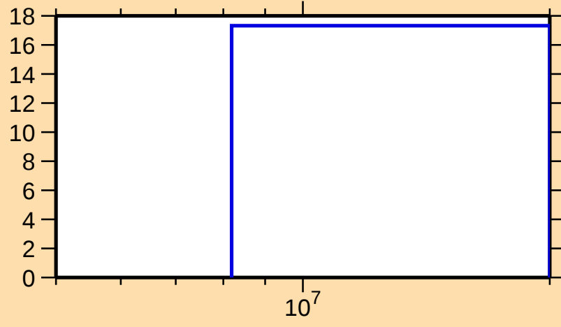
\Delta\sigma/\sigma vs. E for ^{130}\text{La}(n,\text{inel.})
