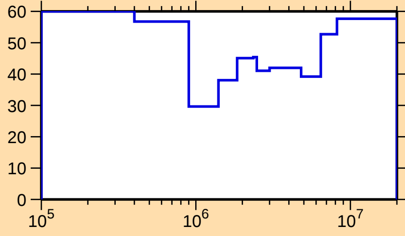
\Delta\sigma/\sigma vs. E for ^{130}\text{La}(n,n_1)
