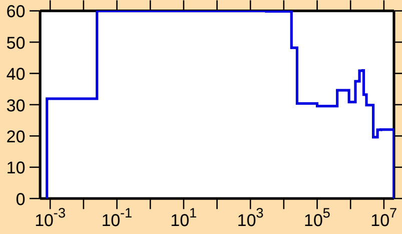
\Delta\sigma/\sigma vs. E for ^{130}\text{La}(n,p)
