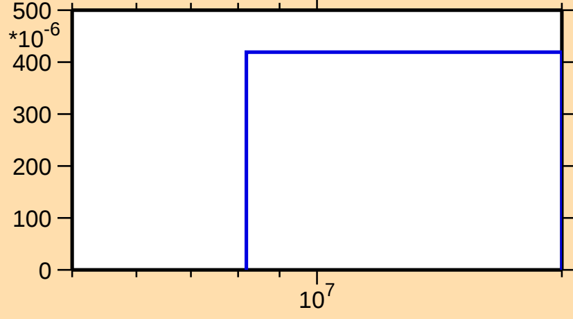
\sigma vs. E for ^{130}\text{La}(n,2np)
