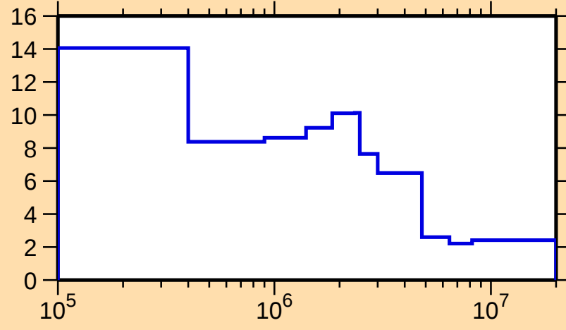
\Delta\sigma/\sigma vs. E for ^{130}\text{La}(n,\text{tot.})
