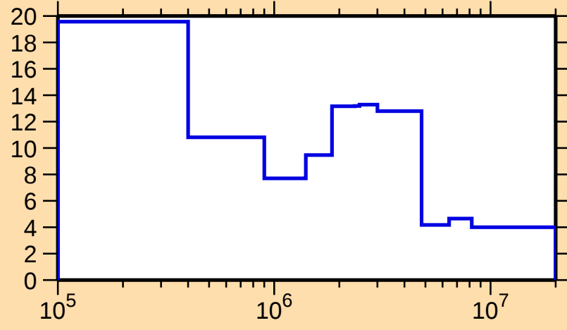
\Delta\sigma/\sigma vs. E for ^{130}\text{La}(n,\text{el.})
