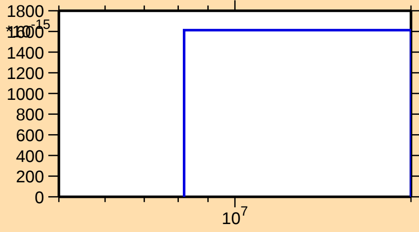
\sigma vs. E for ^{130}\text{La}(\text{mt } 34)
