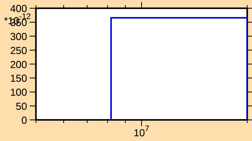
\sigma vs. E for ^{130}\text{La}(n,nt)
