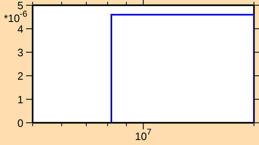
\sigma vs. E for ^{130}\text{La}(n,\text{nd})
