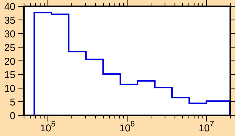
\Delta\sigma/\sigma vs. E for ^{133}\text{La}(n,\text{tot.})
