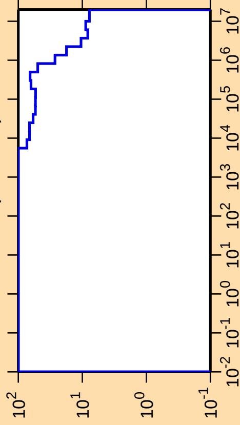
\Delta\sigma/\sigma vs. E for ^{133}\text{La}(n,\text{nonel.})
