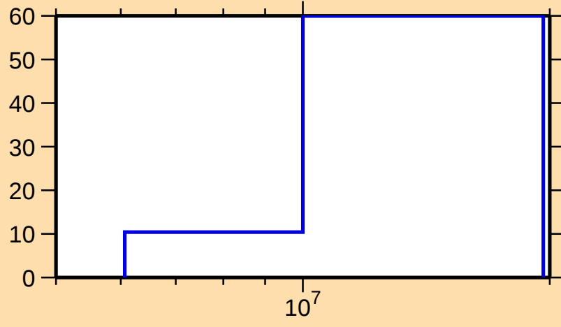
\Delta\sigma/\sigma vs. E for ^{133}\text{La}(n,\text{inel.})
