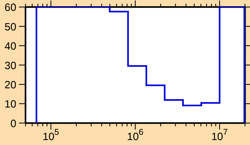
\Delta\sigma/\sigma vs. E for ^{133}\text{La}(n,\text{inel.})
