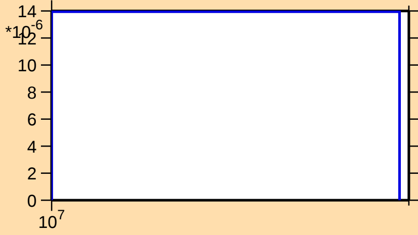
\sigma vs. E for ^{133}\text{La}(n,3n)
