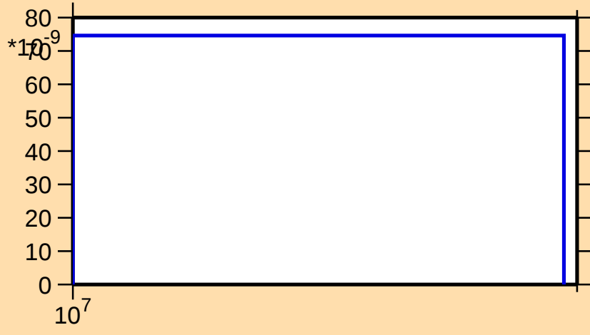
\sigma vs. E for ^{133}\text{La}(n,\text{nd})
