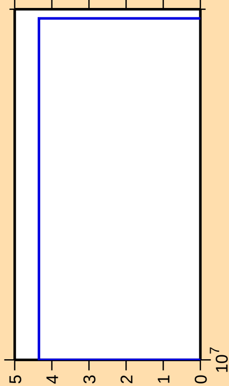
\Delta\sigma/\sigma vs. E for ^{133}\text{La}(n,\text{pd})
