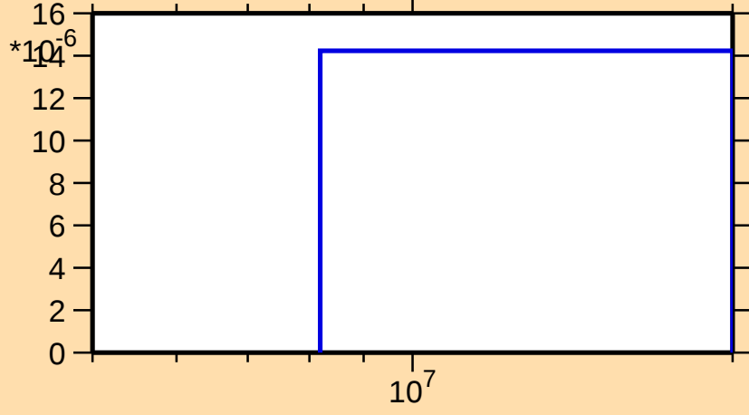
\sigma vs. E for ^{133}\text{La}(n,3n)
