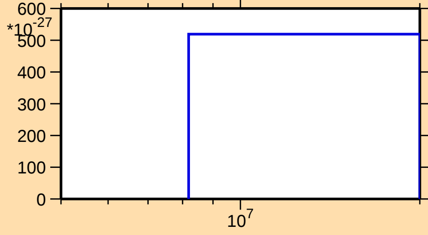
\sigma vs. E for ^{133}\text{La}(\text{mt } 11)
