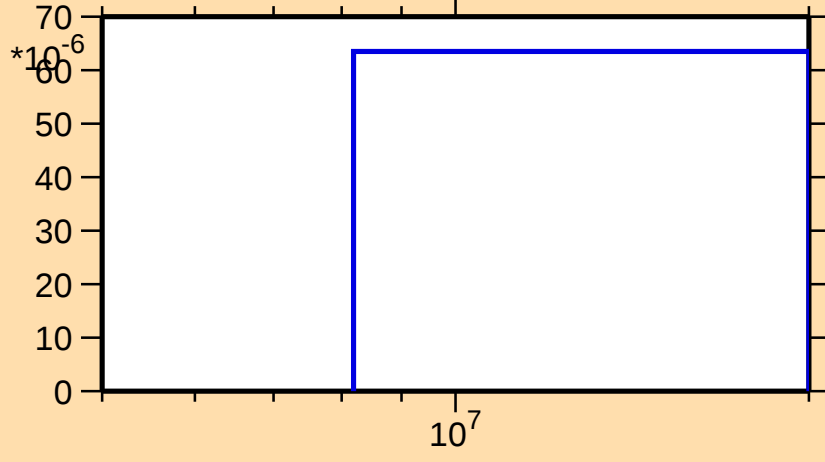
\sigma vs. E for ^{133}\text{La}(n,t)
