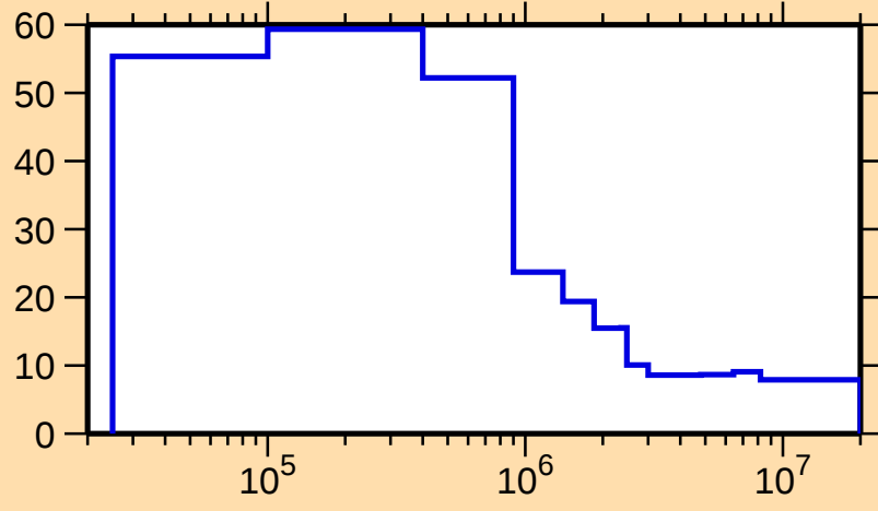
\Delta\sigma/\sigma vs. E for ^{133}\text{La}(n,\text{nonel.})
