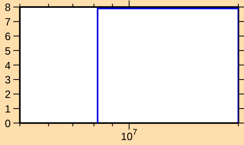
\Delta\sigma/\sigma vs. E for ^{133}\text{La}(n,\text{nonel.})
