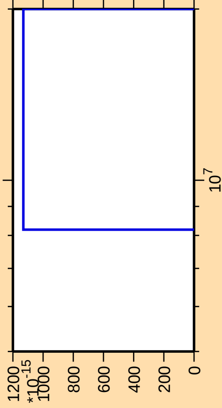
\Delta\sigma/\sigma vs. E for ^{133}\text{La}(\text{mt } 11)
