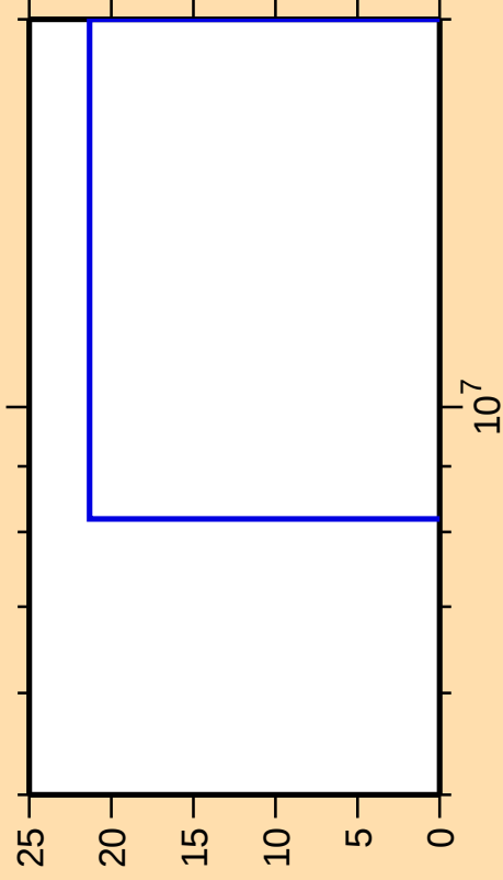
\Delta\sigma/\sigma vs. E for ^{133}\text{La}(\text{mt } 45)
