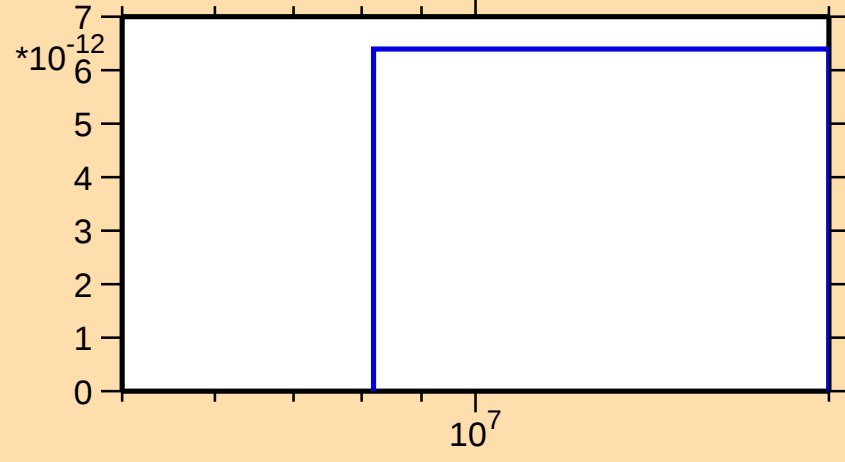
\sigma vs. E for ^{133}\text{La}(\text{mt } 45)
