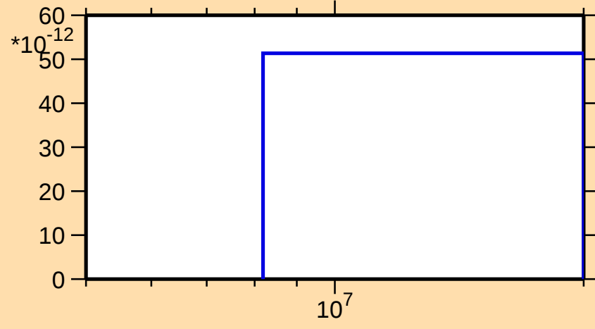
\sigma vs. E for ^{133}\text{La}(n,2n\alpha)
