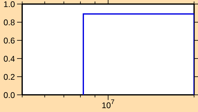
\sigma vs. E for ^{133}\text{La}(n,2n)
