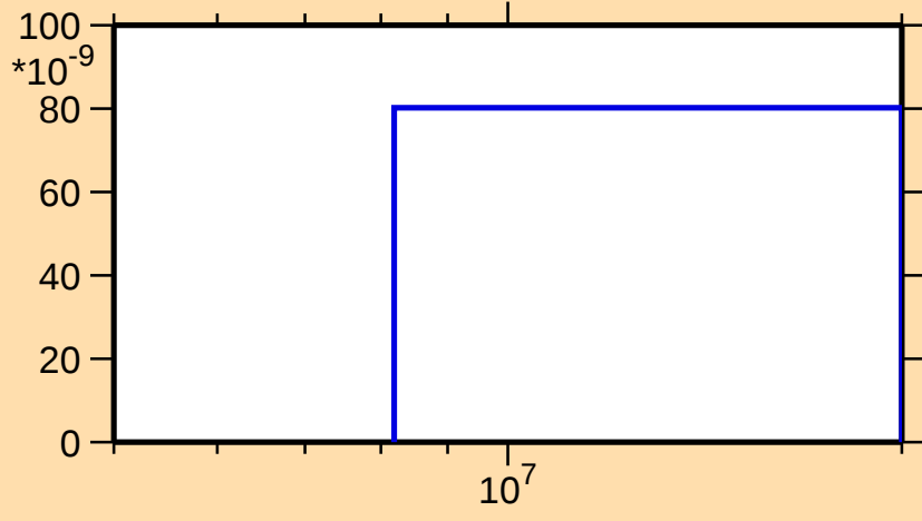
\sigma vs. E for ^{133}\text{La}(n,p\alpha)
