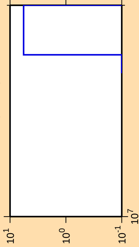
\Delta\sigma/\sigma vs. E for ^{148}\text{La}(n,3n\alpha)
