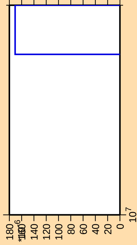
\Delta\sigma/\sigma vs. E for ^{148}\text{La} (mt 42)
