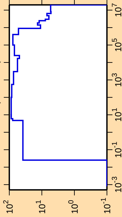
\Delta\sigma/\sigma vs. E for ^{148}\text{La}(n,\text{nonel.})
