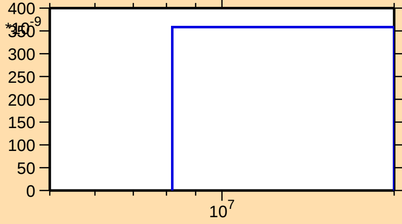
\sigma vs. E for ^{148}\text{La}(n,\text{nd})
