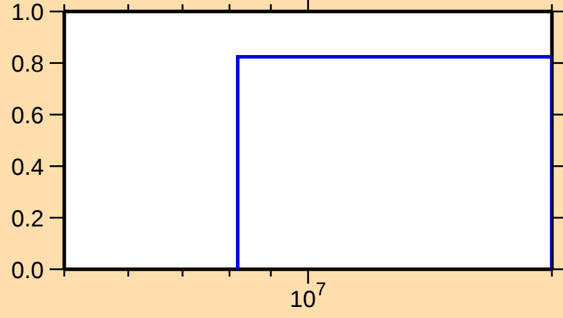
\sigma vs. E for ^{148}\text{La}(n,3n)
