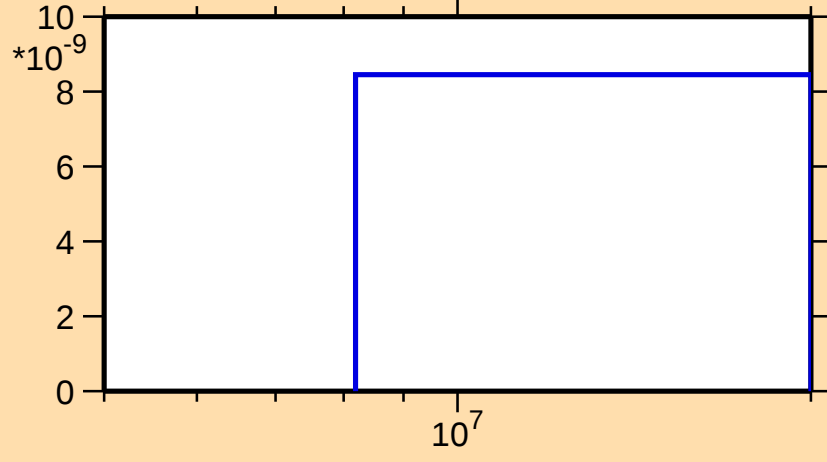
\sigma vs. E for ^{148}\text{La}(n,2np)
