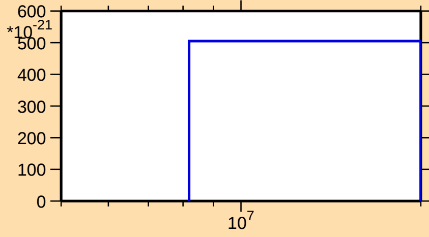
\sigma vs. E for ^{148}\text{La}(\text{mt } 42)
