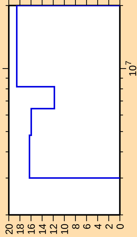
\Delta\sigma/\sigma vs. E for ^{148}\text{La}(n,2n)
