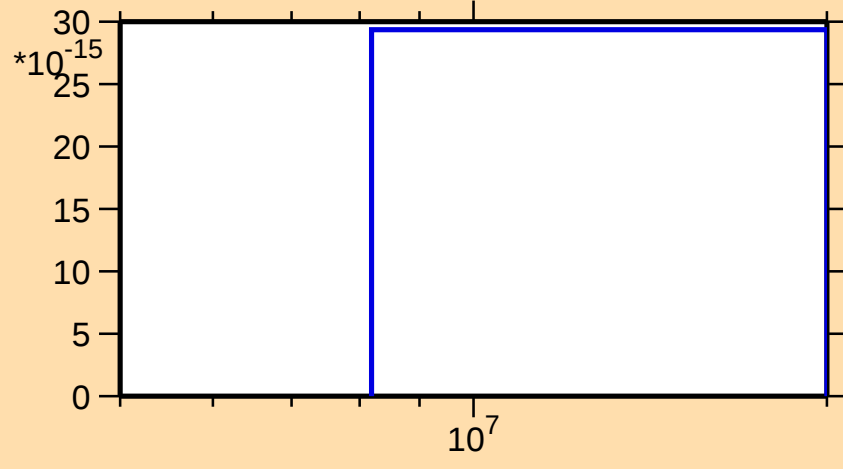
\sigma vs. E for ^{148}\text{La}(\text{mt 11})
