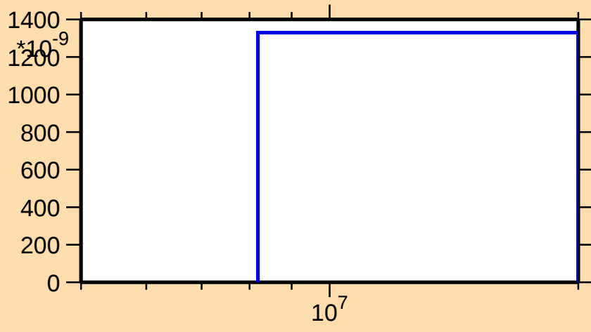
\sigma vs. E for ^{148}\text{La}(n,nt)
