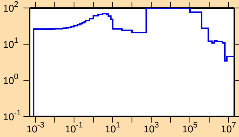
\Delta\sigma/\sigma vs. E for ^{148}\text{La}(n,\text{tot.})
