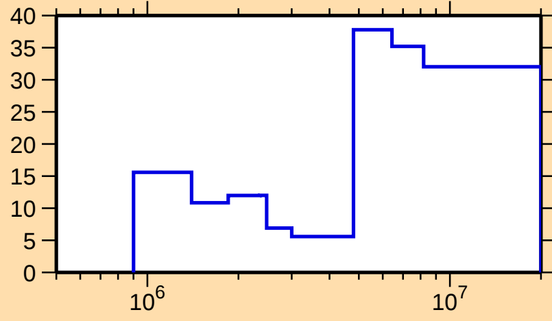
\Delta\sigma/\sigma vs. E for ^{148}\text{La}(n,\text{inel.})
