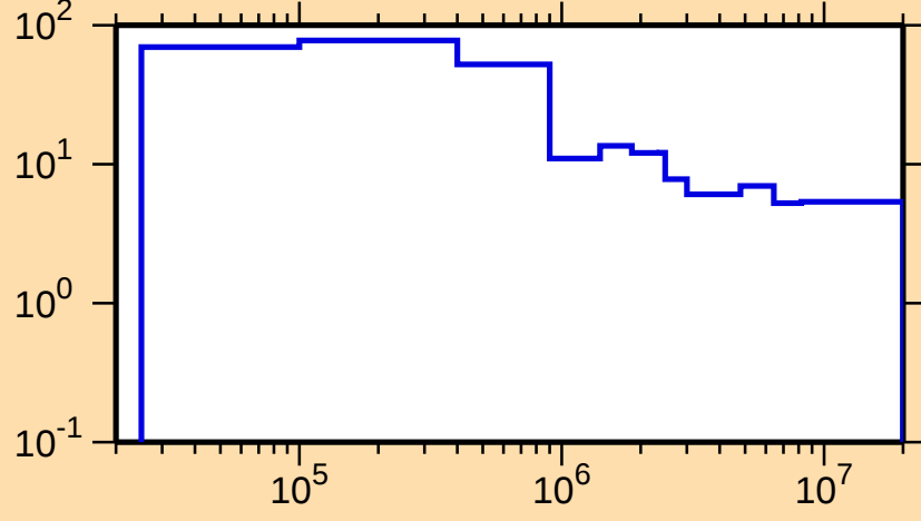
\Delta\sigma/\sigma vs. E for ^{148}\text{La}(n,\text{nonel.})
