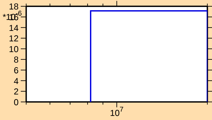
\sigma vs. E for ^{148}\text{La}(n,np)
