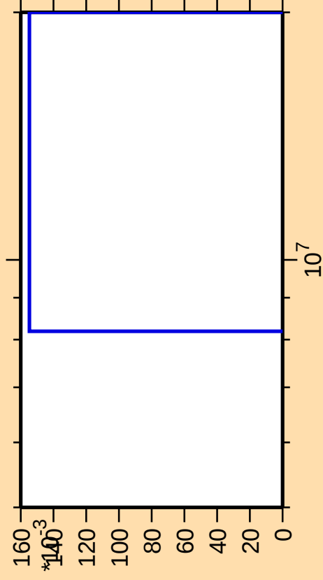
\Delta\sigma/\sigma vs. E for ^{148}\text{La}(\text{mt 11})
