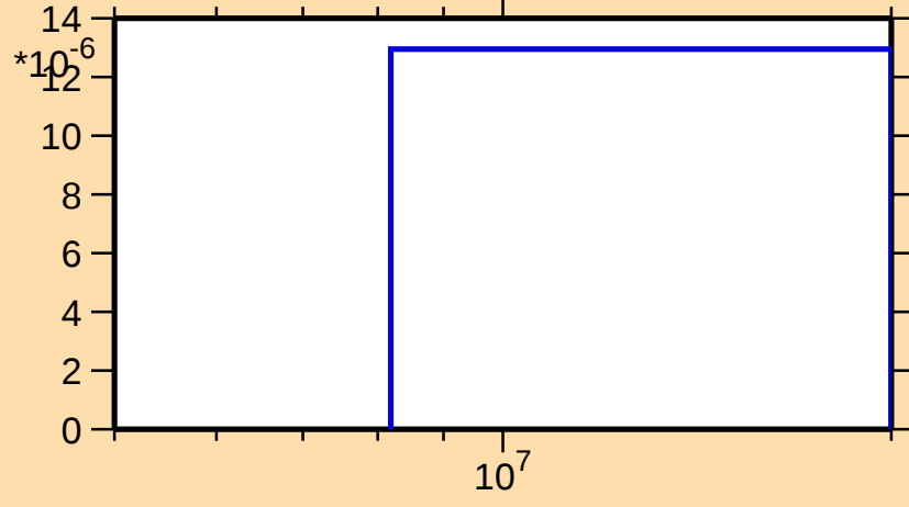
\sigma vs. E for ^{148}\text{La}(n,n\alpha)
