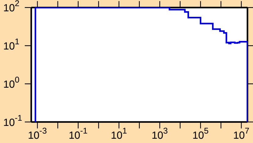
\Delta\sigma/\sigma vs. E for ^{253}\text{Lw}(n,\text{nonel.})
