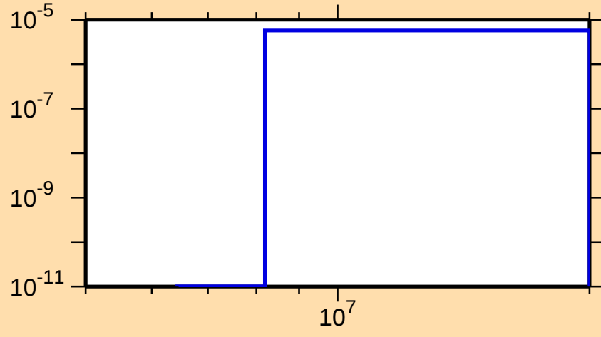
\sigma vs. E for ^{253}\text{Lw}(\text{mt117})
