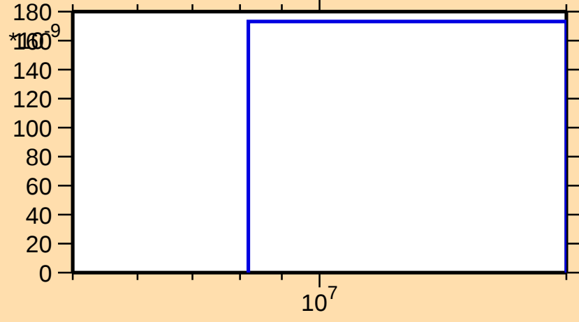
\sigma vs. E for ^{253}\text{Lw}(n,nd)
