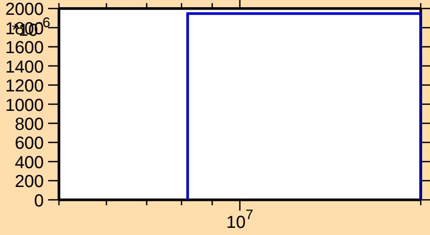
\sigma vs. E for ^{253}\text{Lw}(n,3n)
