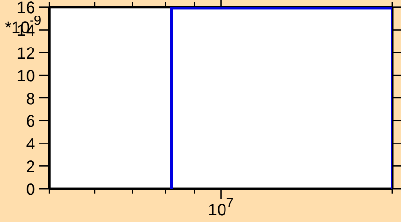
\sigma vs. E for ^{253}\text{Lw}(n,nt)
