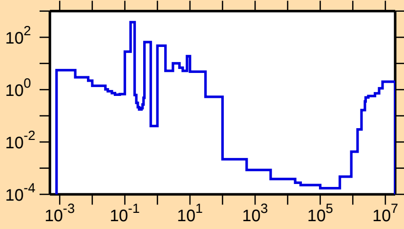
\sigma vs. E for ^{253}\text{Lw}(n,f)
