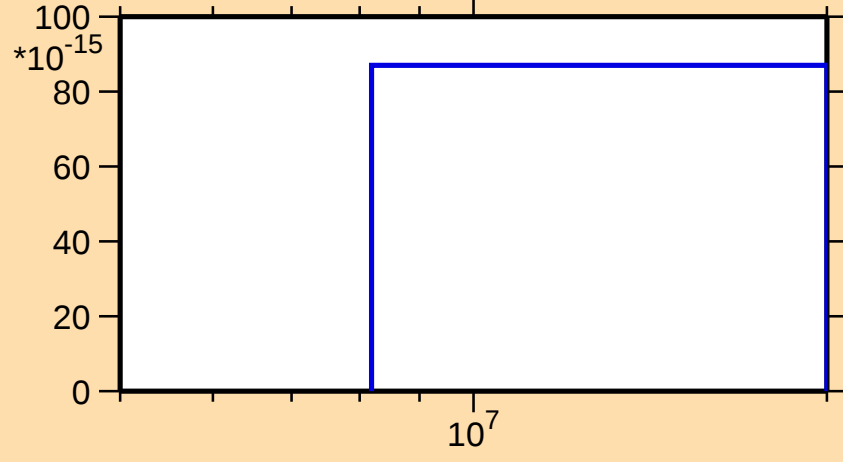
\sigma vs. E for ^{253}\text{Lw}(n,pt)
