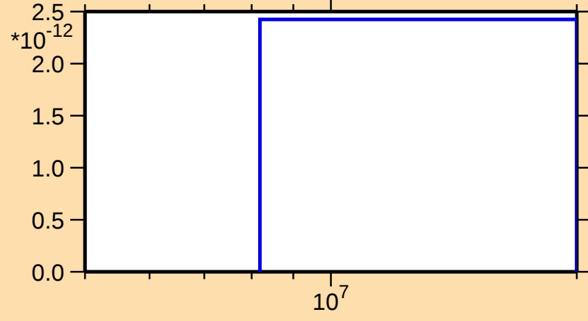
\sigma vs. E for ^{253}\text{Lw}(n,\text{pd})
