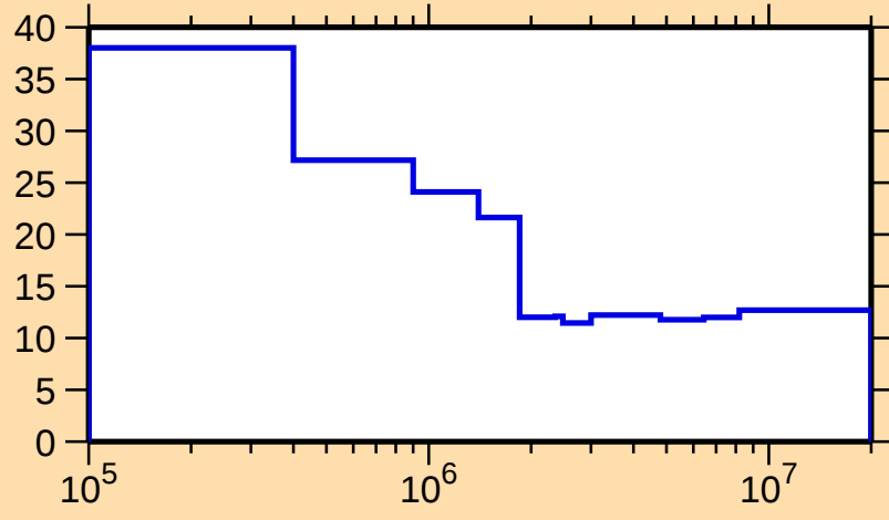
\Delta\sigma/\sigma vs. E for ^{253}\text{Lw}(n,n\text{onel.})
