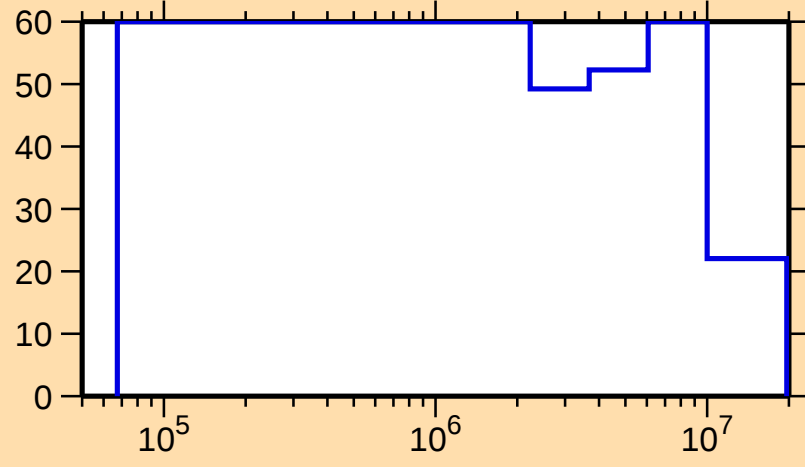
\Delta\sigma/\sigma vs. E for ^{259}\text{Lw}(n, n_1)
