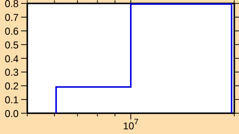
\sigma vs. E for ^{259}\text{Lw}(n,2n)
