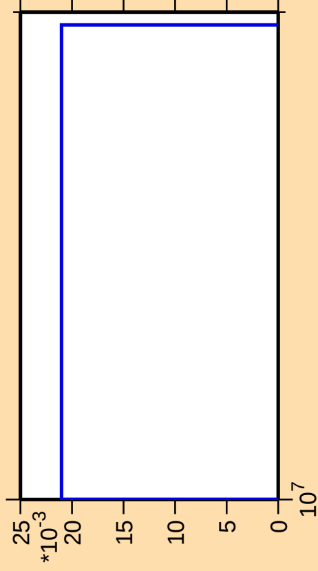
\Delta\sigma/\sigma vs. E for ^{259}\text{Lw}(\text{mt 34})
