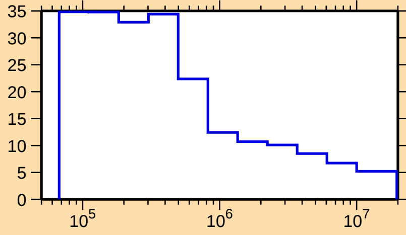
\Delta\sigma/\sigma vs. E for ^{259}\text{Lw}(n,\text{nonel.})
