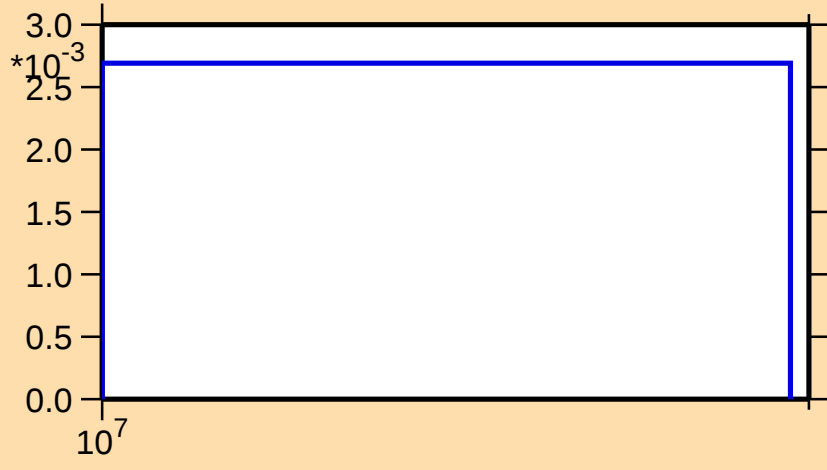
\sigma vs. E for ^{259}\text{Lw}(n,3n\alpha)
