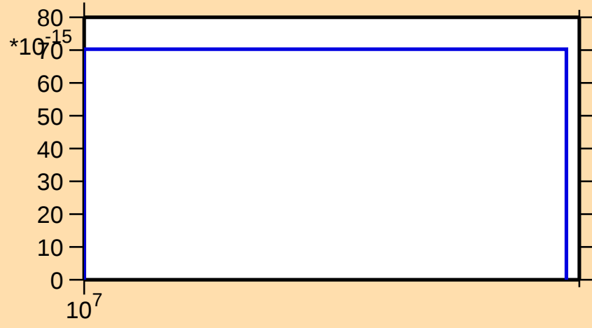
\sigma vs. E for ^{259}\text{Lw}(\text{mt 11})
