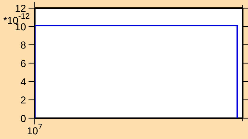
\sigma vs. E for ^{259}\text{Lw}(\text{mt117})
