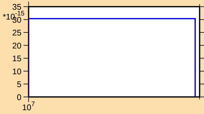
\sigma vs. E for ^{259}\text{Lw}(\text{mt } 42)
