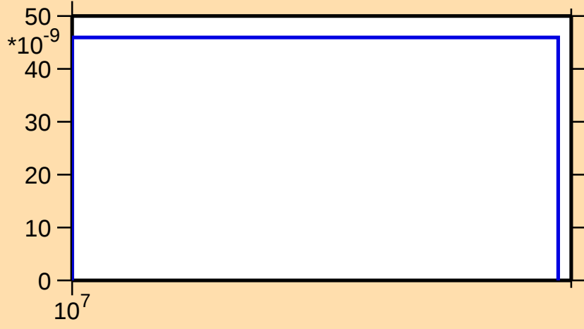
\sigma vs. E for ^{259}\text{Lw}(n,2np)
