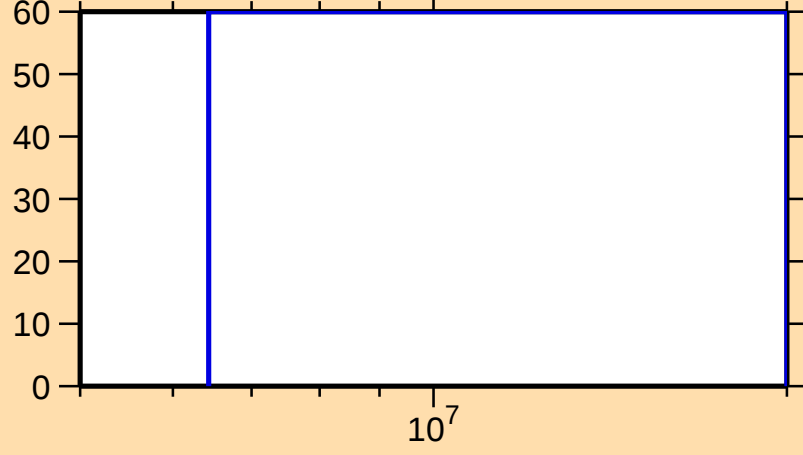
\Delta\sigma/\sigma vs. E for ^{259}\text{Lw}(n,2n)
