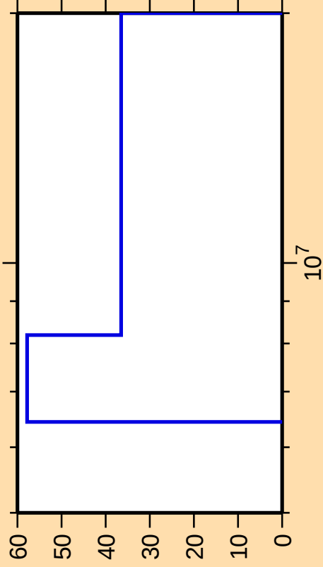
\Delta\sigma/\sigma vs. E for ^{259}\text{Lw}(n,f)
