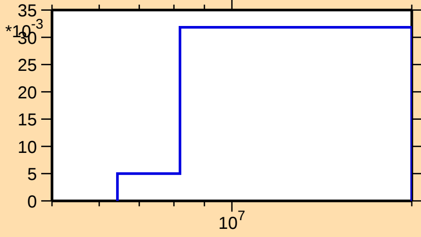
\sigma vs. E for ^{259}\text{Lw}(n,2n\alpha)
