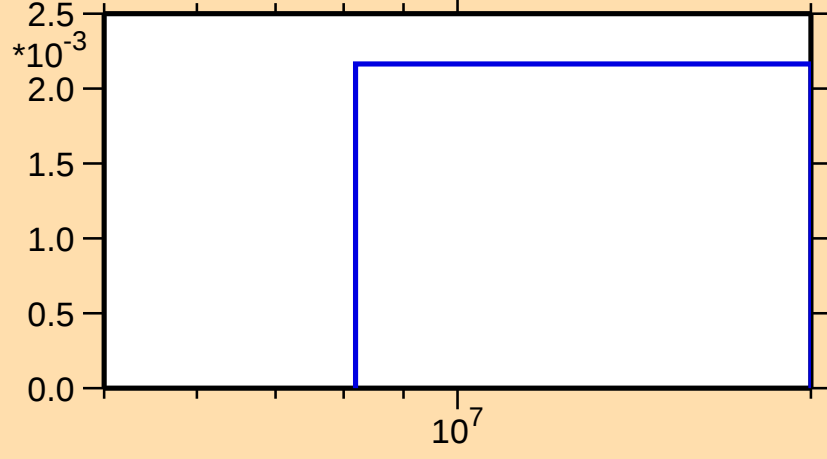
\sigma vs. E for ^{259}\text{Lw}(n,3n\alpha)
