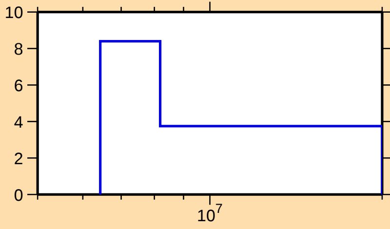
\Delta\sigma/\sigma vs. E for ^{259}\text{Lw}(n,\text{tot.})
