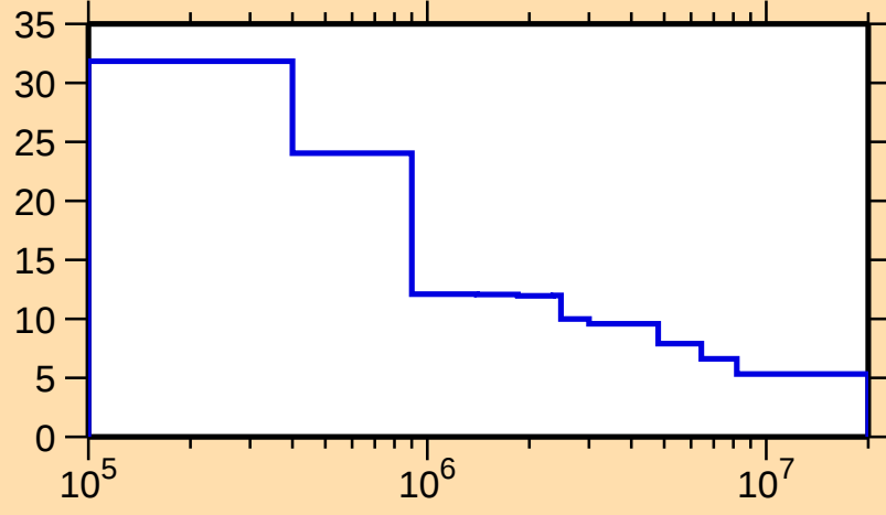
\Delta\sigma/\sigma vs. E for ^{259}\text{Lw}(n, n_{\text{nonel.}})
