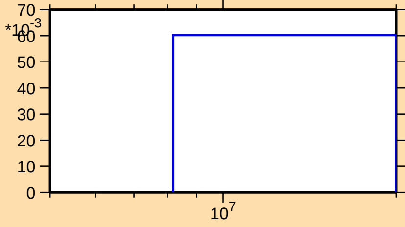
\sigma vs. E for ^{259}\text{Lw}(n,3n)
