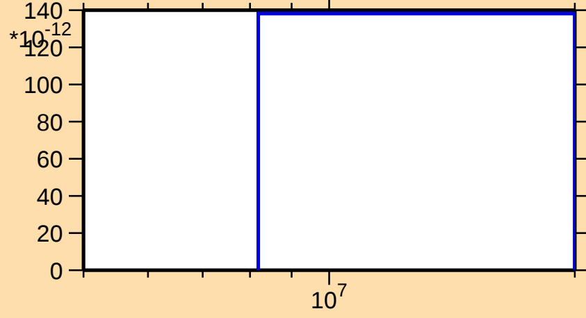
\sigma vs. E for ^{259}\text{Lw}(n,\text{He3})
