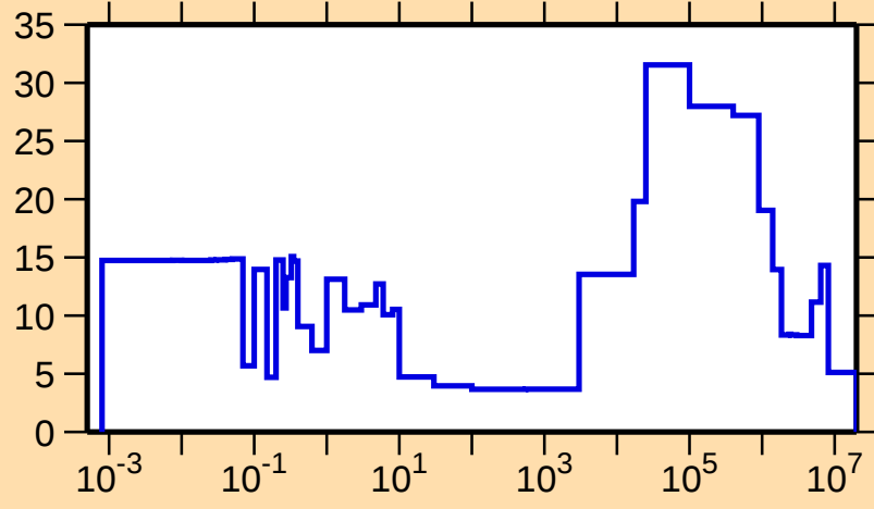
\Delta\sigma/\sigma vs. E for ^{259}\text{Lw}(n,\text{el.})
