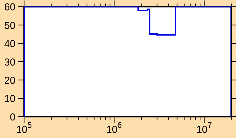
\Delta\sigma/\sigma vs. E for ^{259}\text{Lw}(n, n_1)
