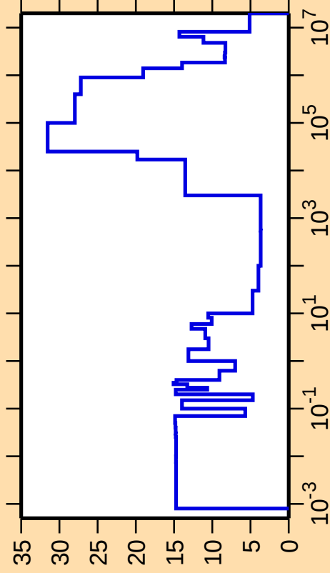
\Delta\sigma/\sigma vs. E for ^{259}\text{Lw}(n,\text{el.})
