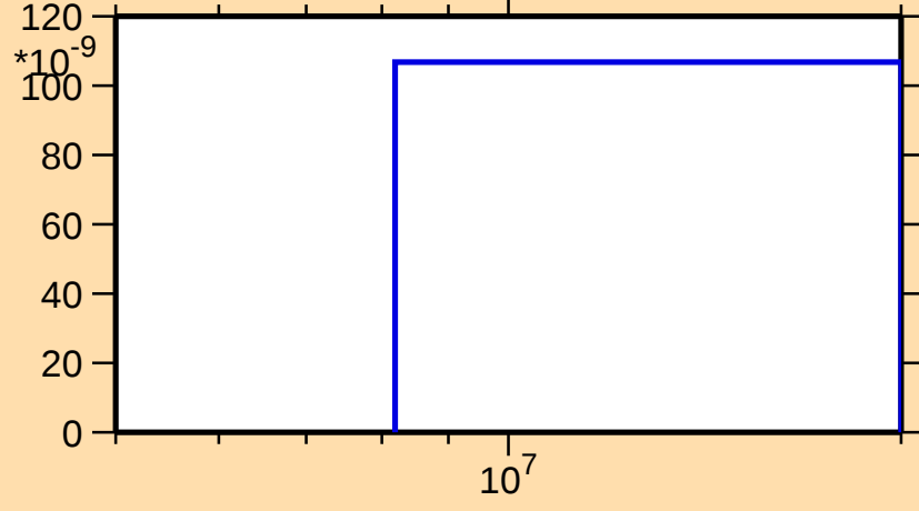
\sigma vs. E for ^{259}\text{Lw}(n,nd)
