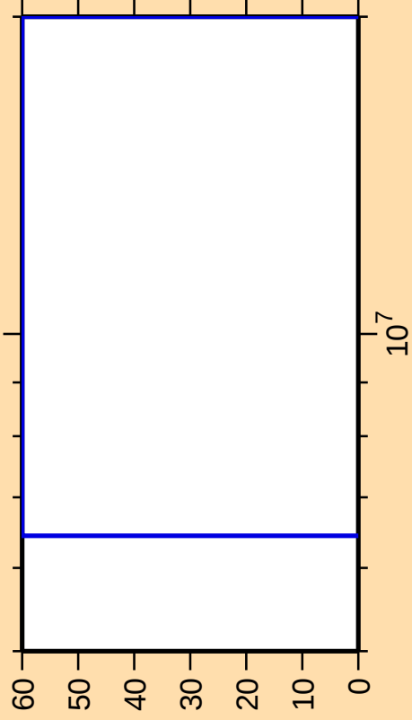
\Delta\sigma/\sigma vs. E for ^{259}\text{Lw}(n,2n\alpha)
