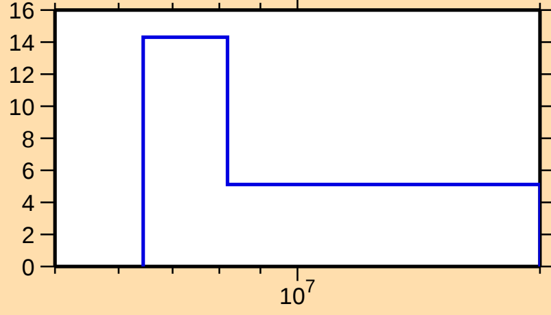
\Delta\sigma/\sigma vs. E for ^{259}\text{Lw}(n,\text{el.})
