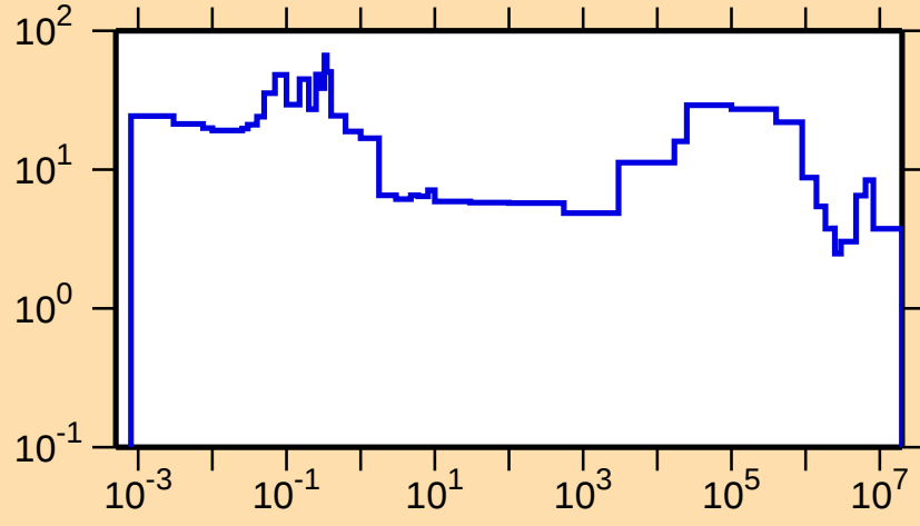
\Delta\sigma/\sigma vs. E for ^{259}\text{Lw}(n,\text{tot.})
