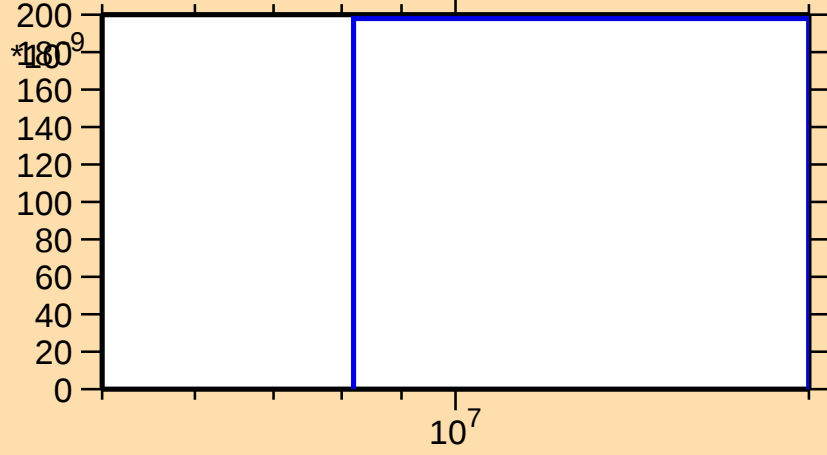
\sigma vs. E for ^{259}\text{Lw}(n,nt)
