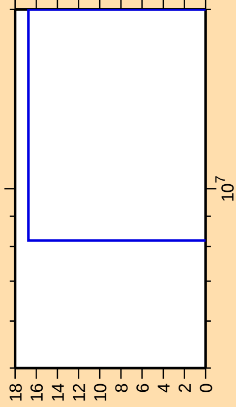
\Delta\sigma/\sigma vs. E for ^{259}\text{Lw}(\text{mt117})
