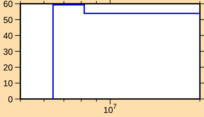
\Delta\sigma/\sigma vs. E for ^{259}\text{Lw}(n,\text{inel.})
