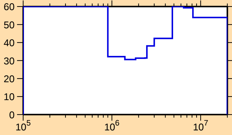
\Delta\sigma/\sigma vs. E for ^{259}\text{Lw}(n,\text{inel.})
