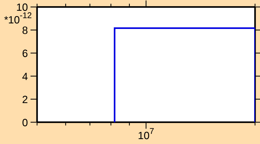
\sigma vs. E for ^{259}\text{Lw}(\text{mt117})
