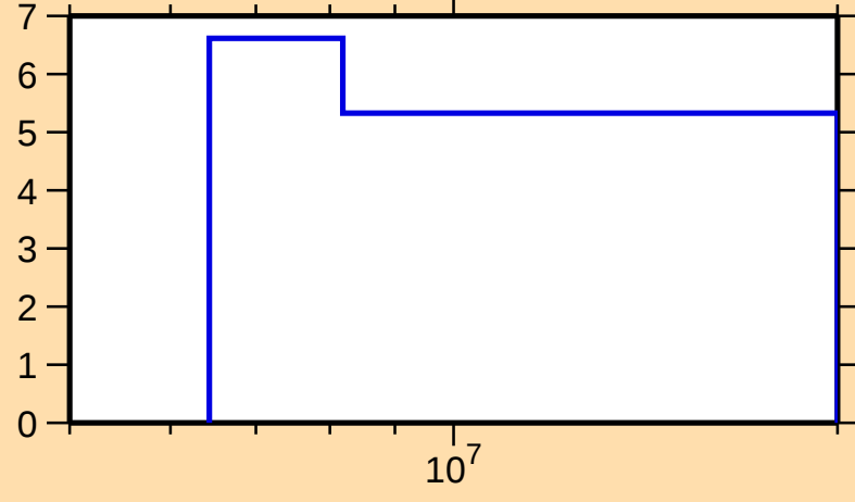
\Delta\sigma/\sigma vs. E for ^{259}\text{Lw}(n,\text{nonel.})
