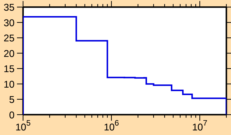
\Delta\sigma/\sigma vs. E for ^{259}\text{Lw}(n,\text{nonel.})
