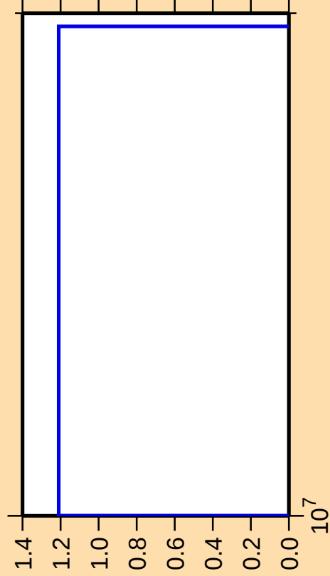
\Delta\sigma/\sigma vs. E for ^{154}\text{Lu}(n,\text{nt})
