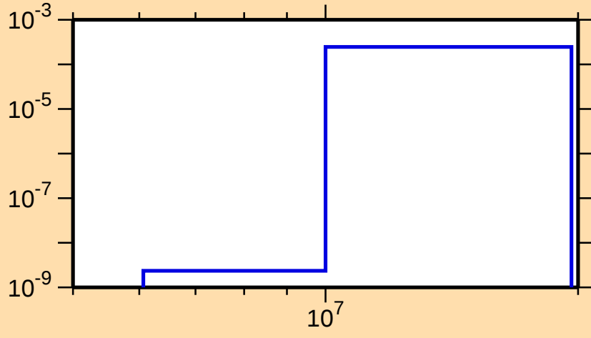
\sigma vs. E for ^{154}\text{Lu}(n,\text{pd})
