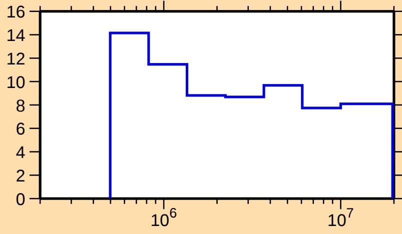
\Delta\sigma/\sigma vs. E for ^{154}\text{Lu}(n,n\text{onel.})
