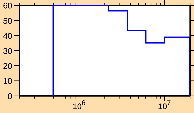
\Delta\sigma/\sigma vs. E for ^{154}\text{Lu}(n,n\text{cont.})
