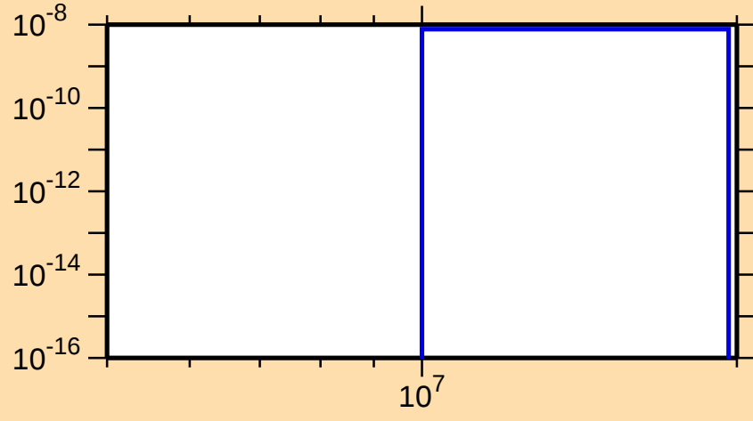
\sigma vs. E for ^{154}\text{Lu}(\text{mt } 34)
