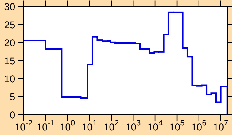
\Delta\sigma/\sigma vs. E for ^{154}\text{Lu}(n,\text{el.})
