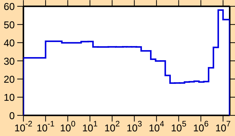
\Delta\sigma/\sigma vs. E for ^{154}\text{Lu}(n,p)
