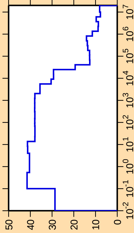
\Delta\sigma/\sigma vs. E for ^{154}\text{Lu}(n,\text{nonel.})
