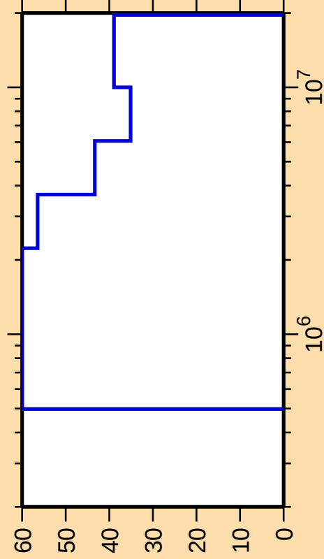
\Delta\sigma/\sigma vs. E for ^{154}\text{Lu}(n,\text{ncont.})
