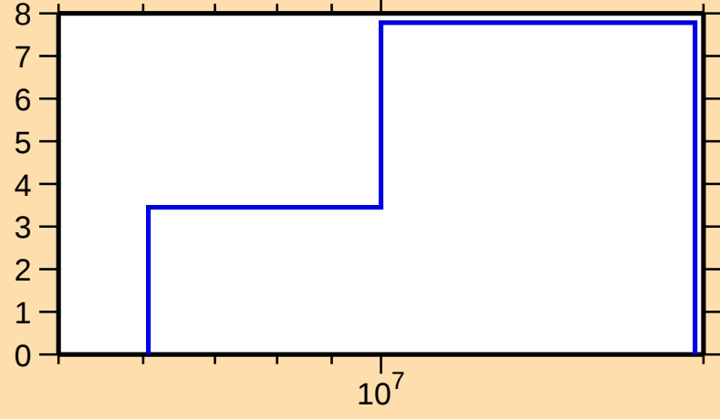
\Delta\sigma/\sigma vs. E for ^{154}\text{Lu}(n,\text{el.})
