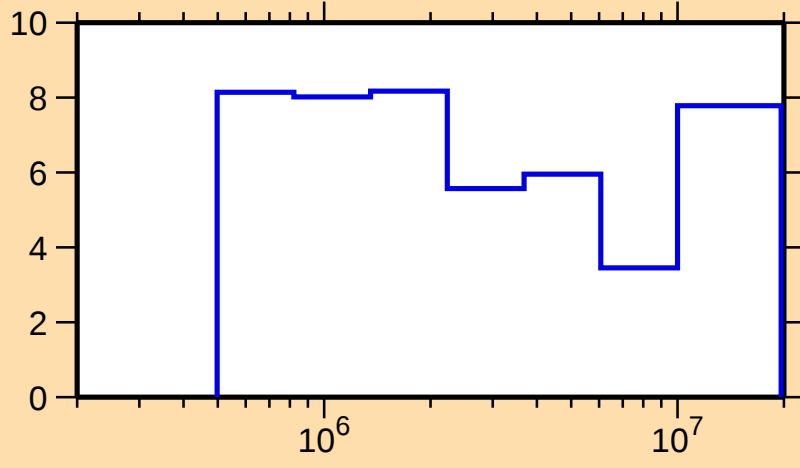
\Delta\sigma/\sigma vs. E for ^{154}\text{Lu}(n,\text{el.})
