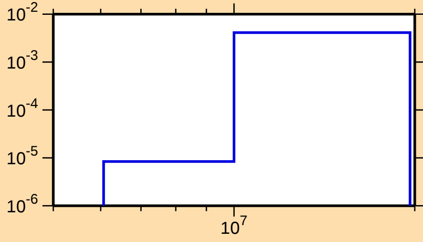
\sigma vs. E for ^{154}\text{Lu}(n,2n)
