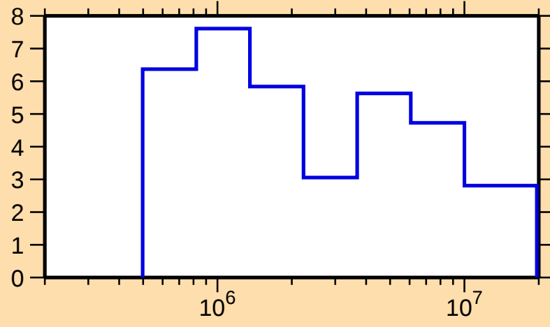
\Delta\sigma/\sigma vs. E for ^{154}\text{Lu}(n,\text{tot.})
