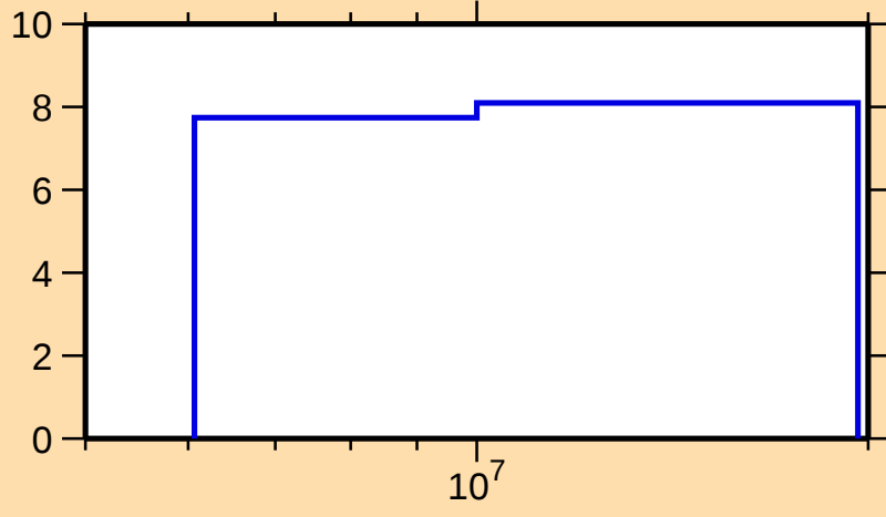
\Delta\sigma/\sigma vs. E for ^{154}\text{Lu}(n,\text{nonel.})
