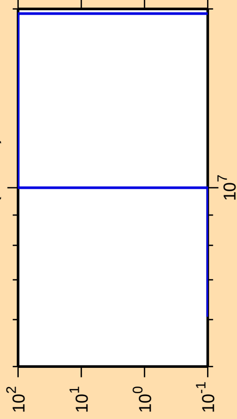
\Delta\sigma/\sigma vs. E for ^{154}\text{Lu}(\text{mt } 34)
