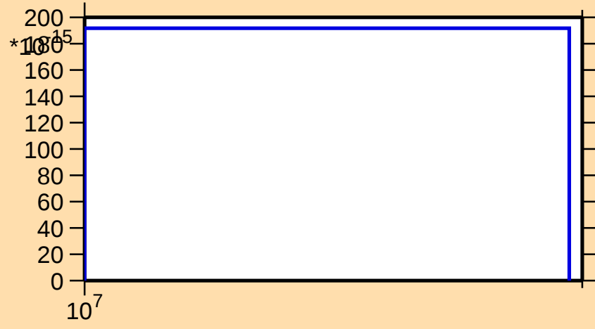
\sigma vs. E for ^{154}\text{Lu}(n,\text{nt})
