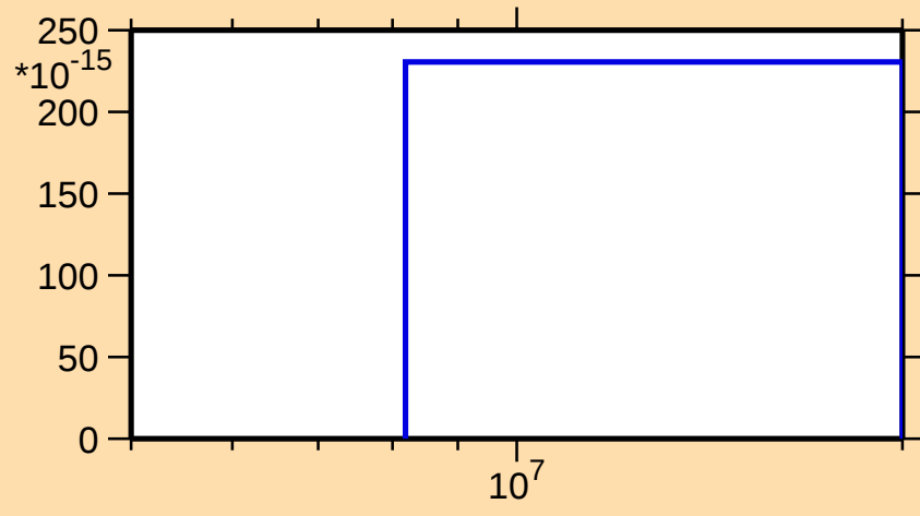
\sigma vs. E for ^{154}\text{Lu}(n,nt)
