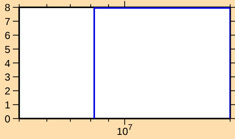
\Delta\sigma/\sigma vs. E for ^{154}\text{Lu}(n,\text{nonel.})
