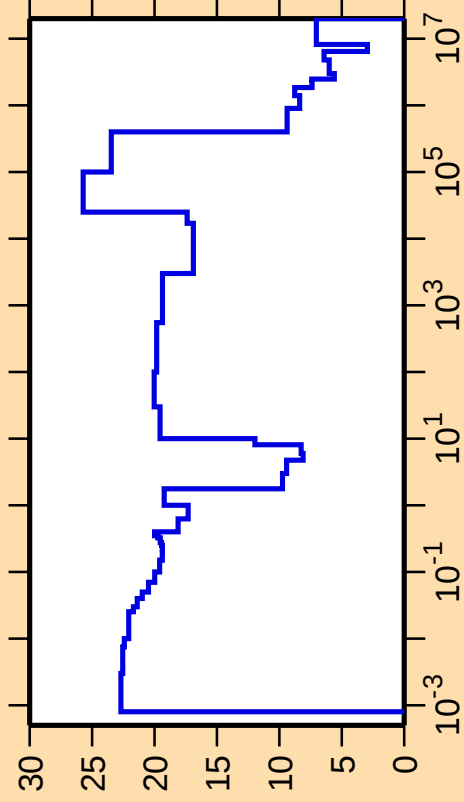
\Delta\sigma/\sigma vs. E for ^{154}\text{Lu}(n,\text{el.})
