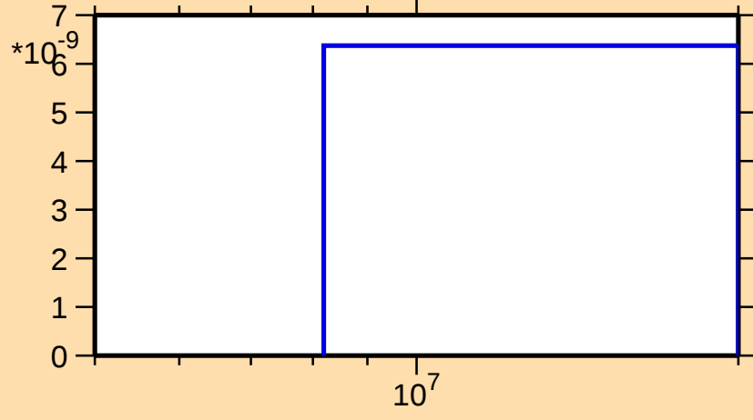
\sigma vs. E for ^{154}\text{Lu} (mt 34)
