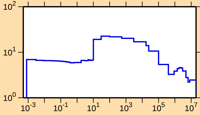
\sigma vs. E for ^{154}\text{Lu}(n,\text{el.})
