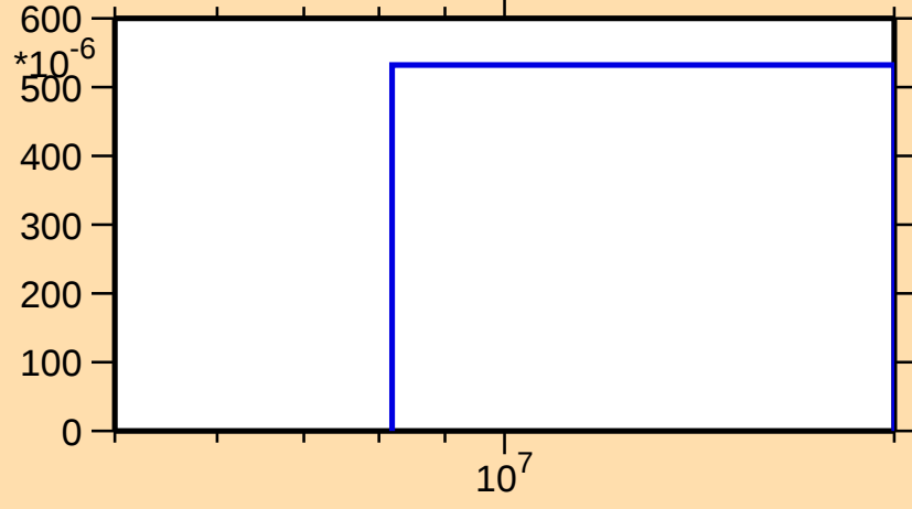
\sigma vs. E for ^{154}\text{Lu}(n,2np)
