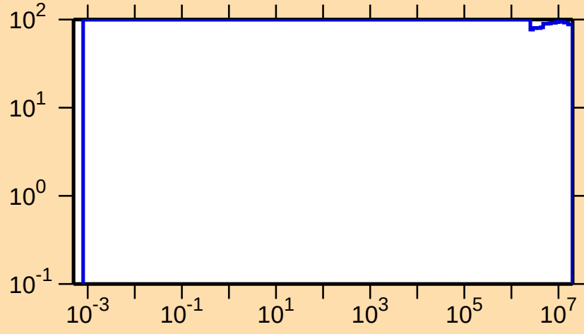
\Delta\sigma/\sigma vs. E for ^{157}\text{Lu}(n,p)
