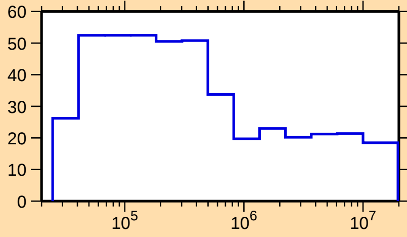
\Delta\sigma/\sigma vs. E for ^{157}\text{Lu}(n,\text{tot.})
