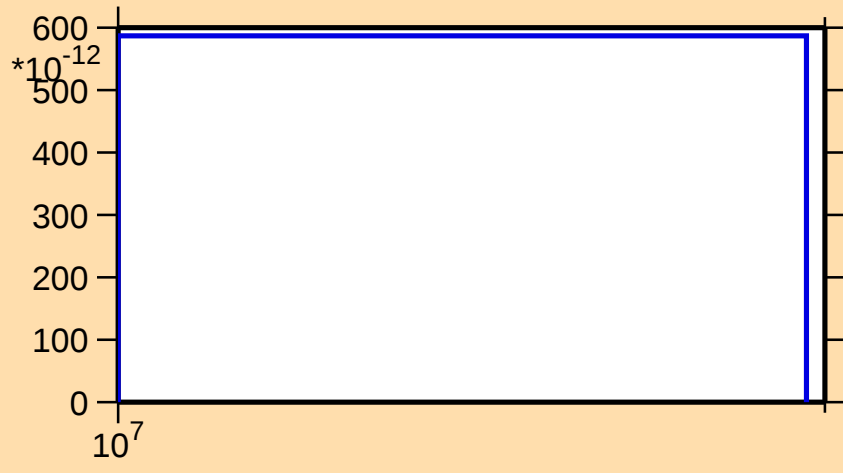
\sigma vs. E for ^{157}\text{Lu}(n,nt)
