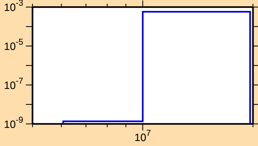
\sigma vs. E for ^{157}\text{Lu}(n,t)
