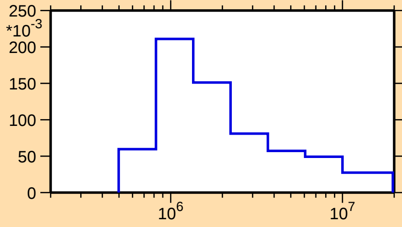
\sigma vs. E for ^{157}\text{Lu}(n,n_3)
