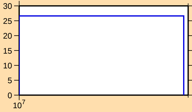
\Delta\sigma/\sigma vs. E for ^{157}\text{Lu}(n,\text{el.})
