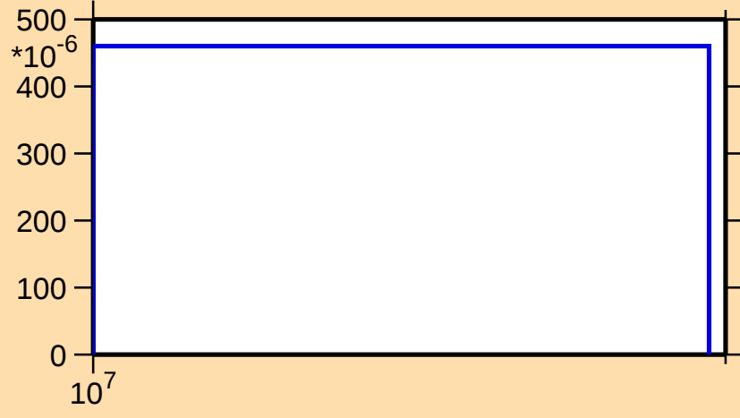
\sigma vs. E for ^{157}\text{Lu}(n,2np)
