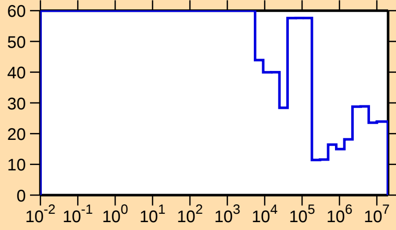
\Delta\sigma/\sigma vs. E for ^{157}\text{Lu}(n,\text{nonel.})
