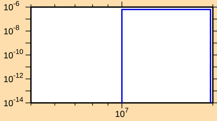
\sigma vs. E for ^{157}\text{Lu}(n,\text{nd})
