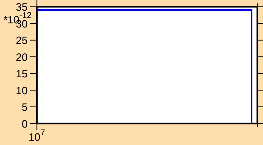
\sigma vs. E for ^{157}\text{Lu} (mt 34)
