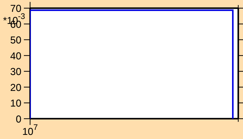
\sigma vs. E for ^{157}\text{Lu}(n,2n)
