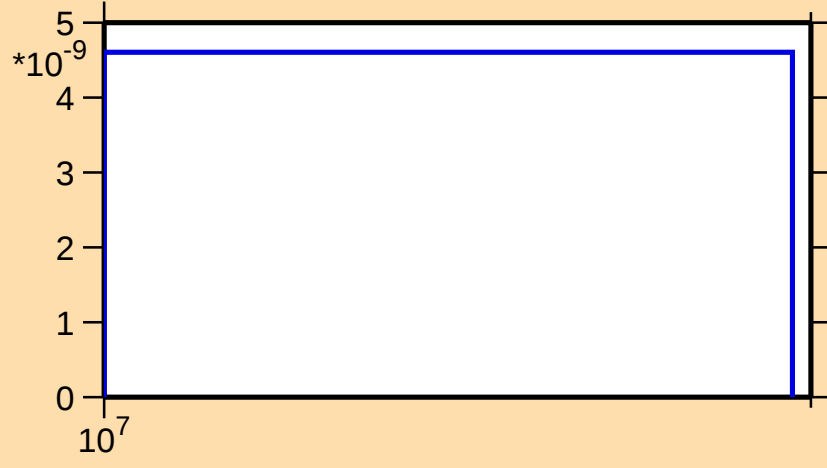
\sigma vs. E for ^{157}\text{Lu}(n,\text{pt})
