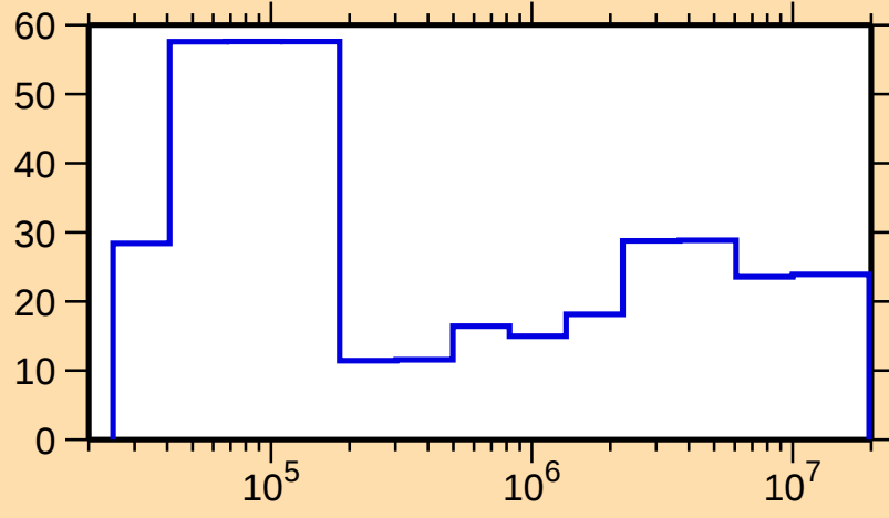
\Delta\sigma/\sigma vs. E for ^{157}\text{Lu}(n,\text{nonel.})
