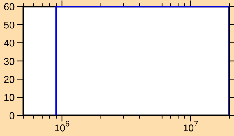
\Delta\sigma/\sigma vs. E for ^{157}\text{Lu}(n,\text{ncont.})
