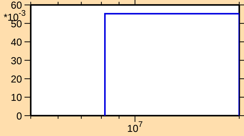
\sigma vs. E for ^{157}\text{Lu}(n,2n)
