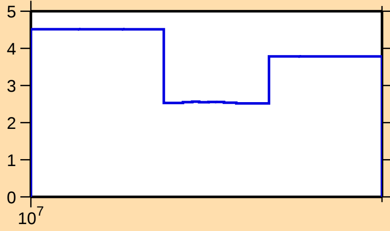
\Delta\sigma/\sigma vs. E for ^{157}\text{Lu}(n,\text{tot.})
