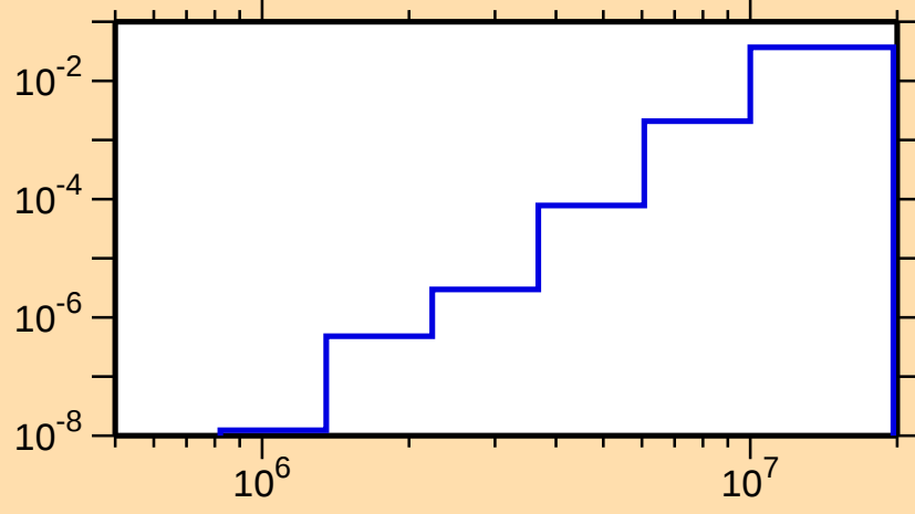
\sigma vs. E for ^{157}\text{Lu}(n,n\alpha)
