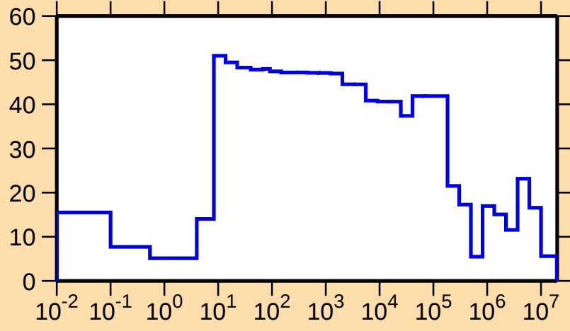
\Delta\sigma/\sigma vs. E for ^{157}\text{Lu}(n,\text{el.})
