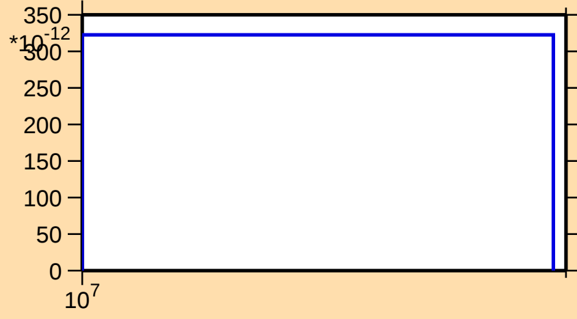
\sigma vs. E for ^{157}\text{Lu}(n,\text{nt})
