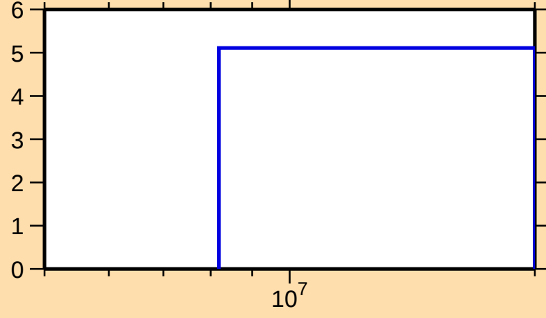
\Delta\sigma/\sigma vs. E for ^{157}\text{Lu}(n,\text{el.})
