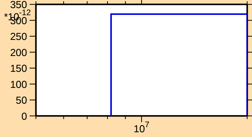
\sigma vs. E for ^{157}\text{Lu}(n,nt)
