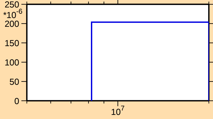
\sigma vs. E for ^{157}\text{Lu}(n,2np)
