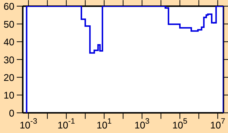
\Delta\sigma/\sigma vs. E for ^{157}\text{Lu}(n,\gamma)
