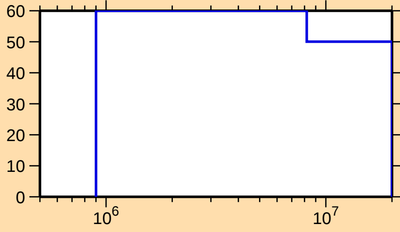
\Delta\sigma/\sigma vs. E for ^{157}\text{Lu}(n,n\text{cont.})
