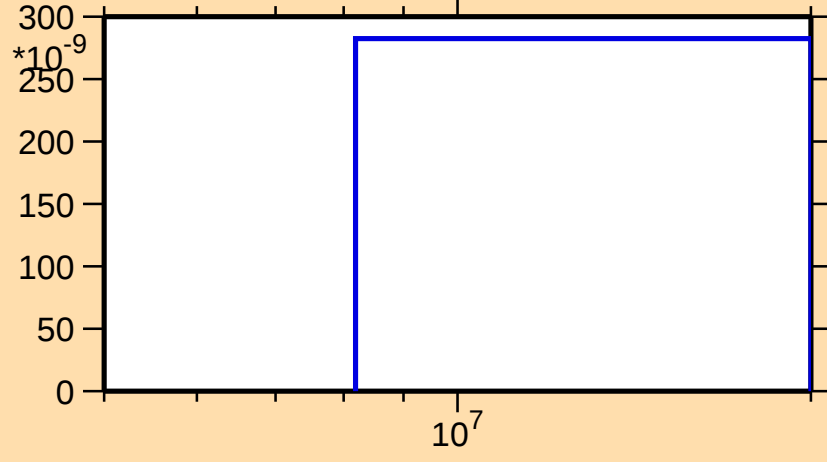
\sigma vs. E for ^{157}\text{Lu}(n,\text{nd})
