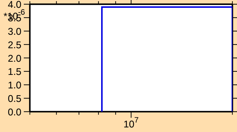
\sigma vs. E for ^{157}\text{Lu}(n,\text{pd})
