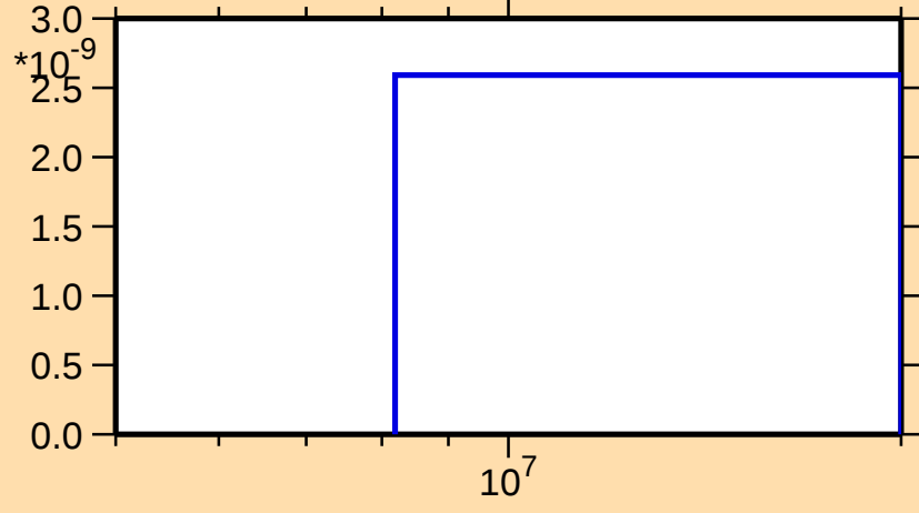
\sigma vs. E for ^{157}\text{Lu}(n,\text{pt})
