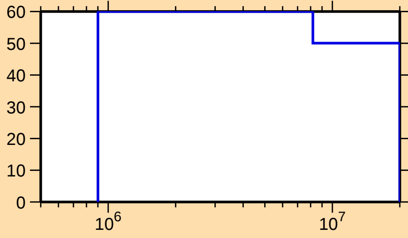
\Delta\sigma/\sigma vs. E for ^{157}\text{Lu}(n,n\text{cont.})
